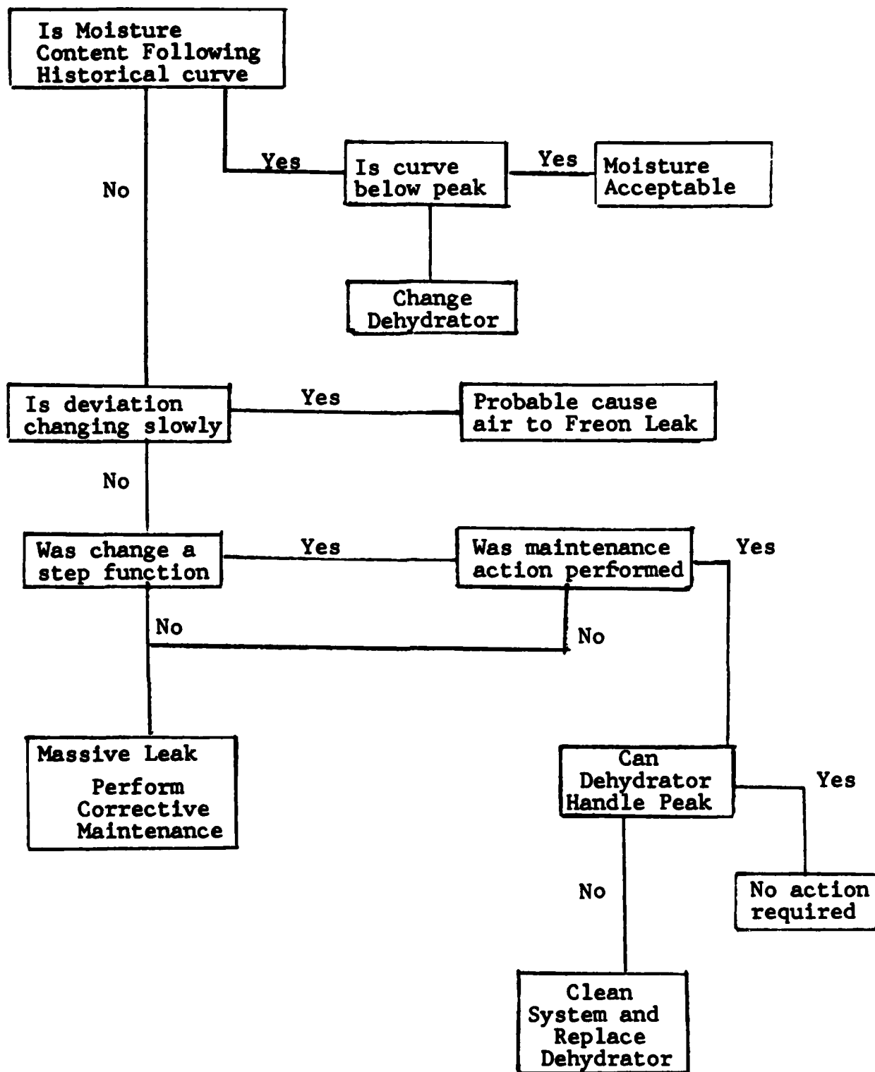
Figure 7.2-1. Moisture Logic Tree
