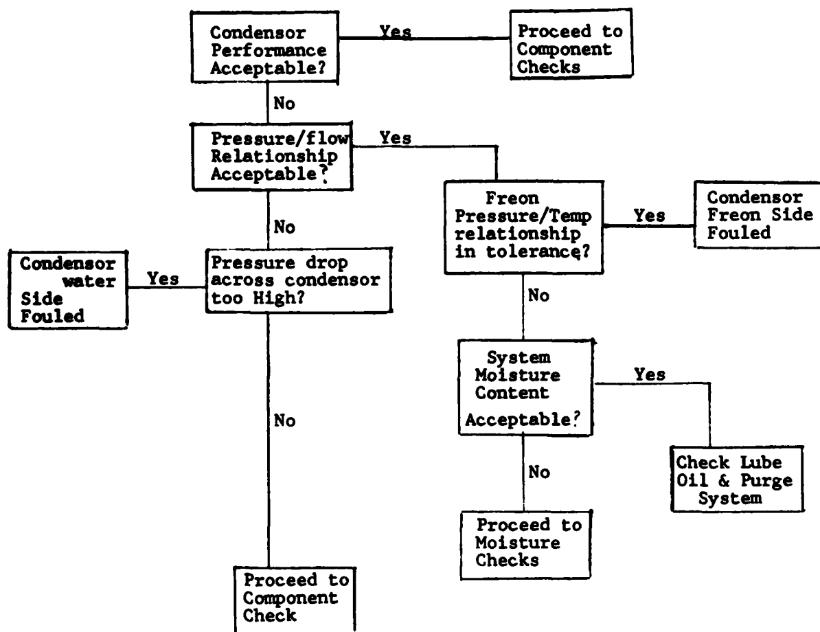
FIGURE 7.2-2. Condensor Performance Logic Tree
