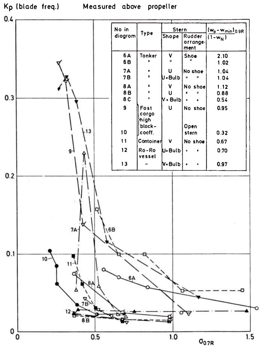
Figure 56 - Pressure Pulse Coefficients for Some Different Projects (From Lindgren and Bjärne 13 )
