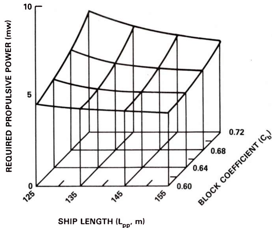
Figure 13 - 12,000\text{-m}^3 Displacement RO/RO. Required Propulsive Power Versus Hull Length and Fullness. Speed is 18 Knots. (From Williams 8 )
