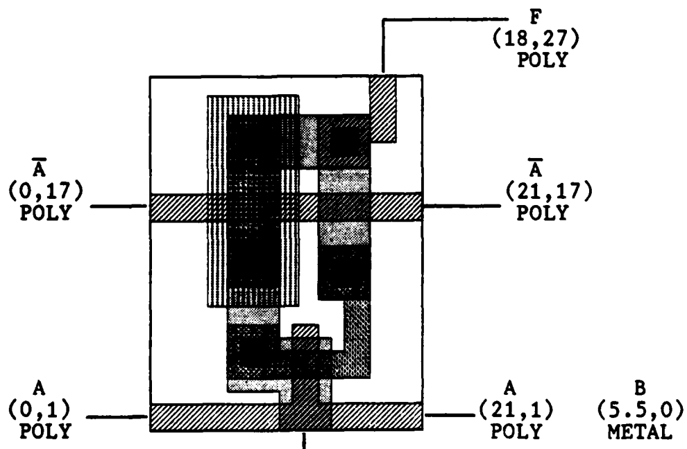
Cifplot
