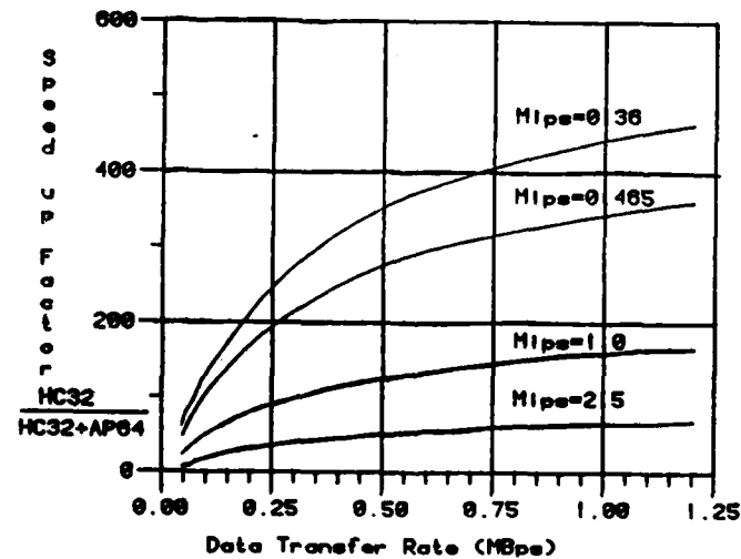
Figure 9 Effect of Data Transfer Rate on Speed up Factor for the Decomposition Processor. (U=8736). AP Speed = 18.2 MFLCPS.
