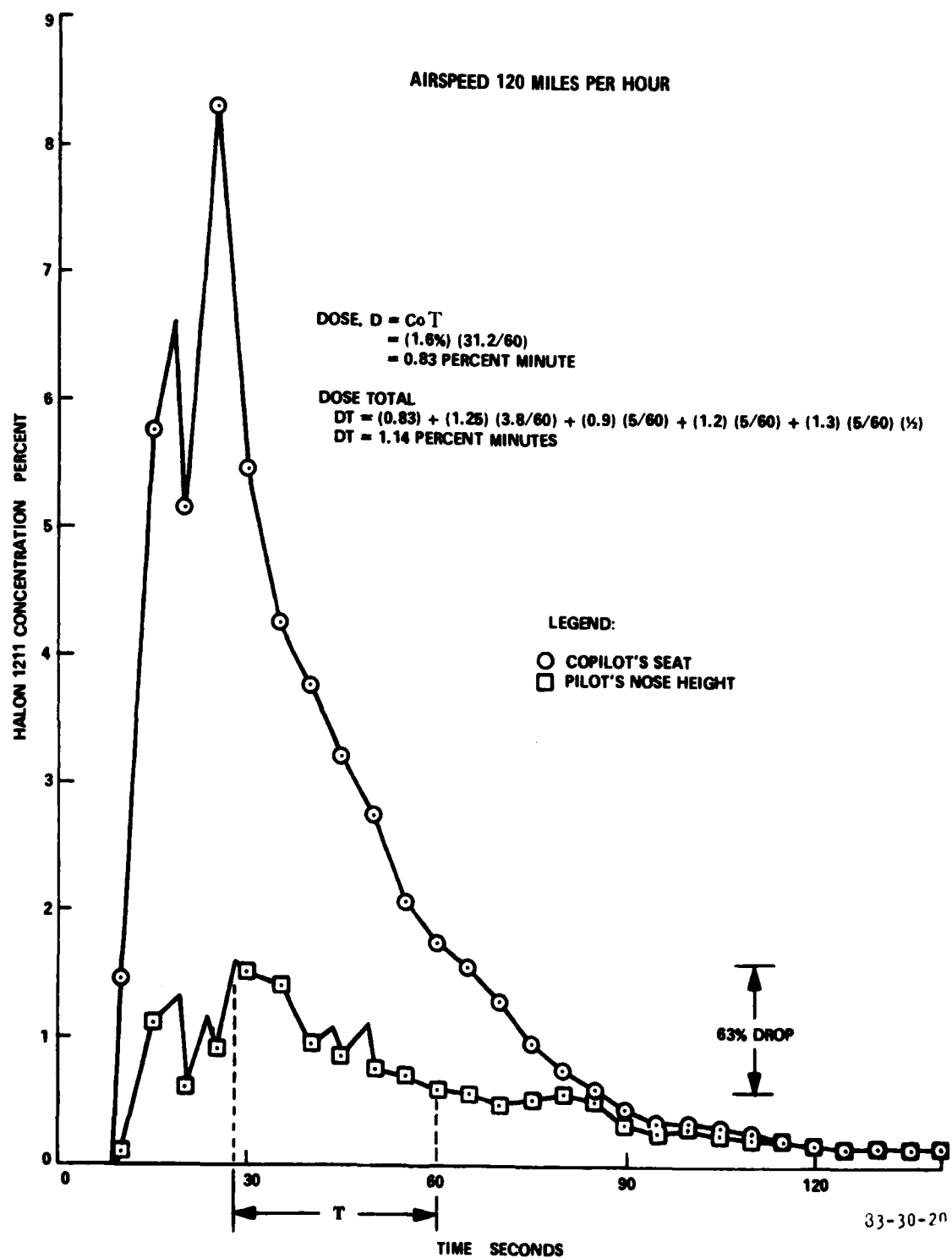
FIGURE 20. HALON 1211 CONCENTRATIONS - 2.5 POUND EXTINGUISHER DIRECTED TO THE COPILOT'S SEAT - ALL VENTS CLOSED
