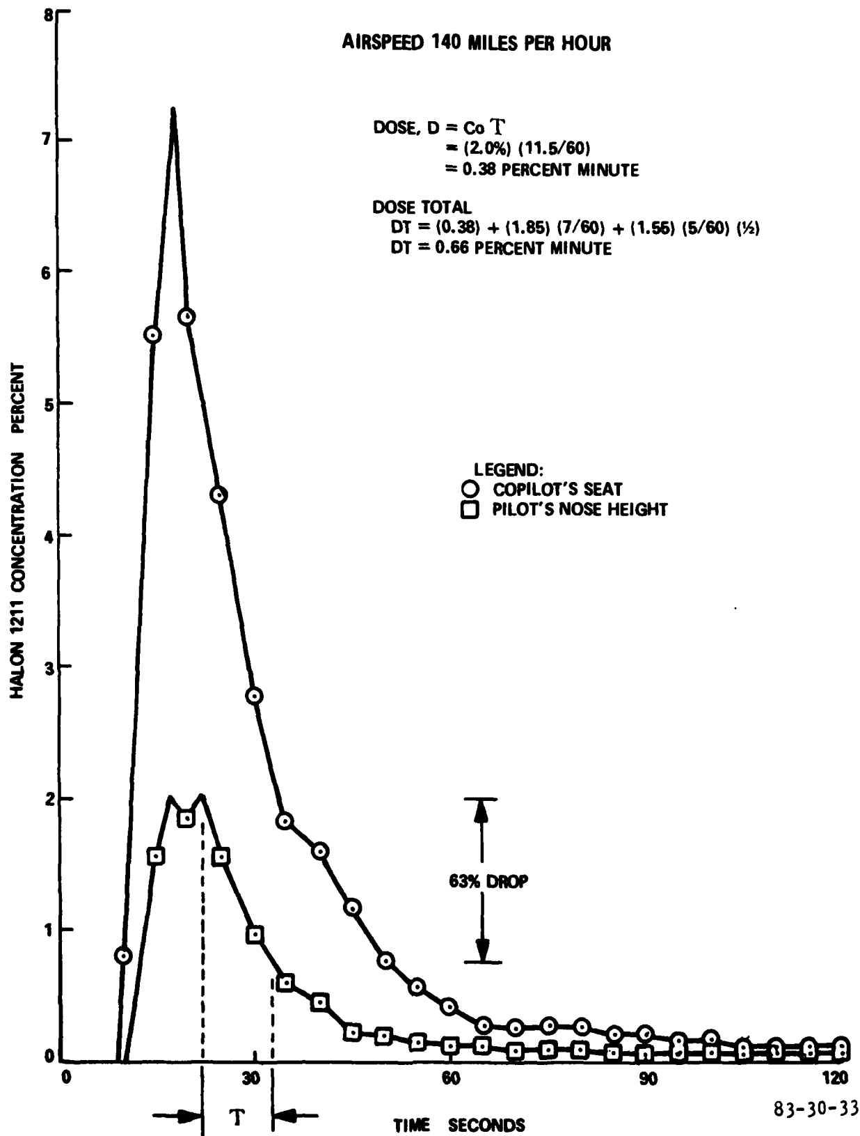
FIGURE 33. HALON 1211 CONCENTRATIONS - 2.5 POUND EXTINGUISHER DIRECTED TO THE COPILOT'S SEAT - AIRSPEED 140 MPH - OVERHEAD VENTS OPEN
