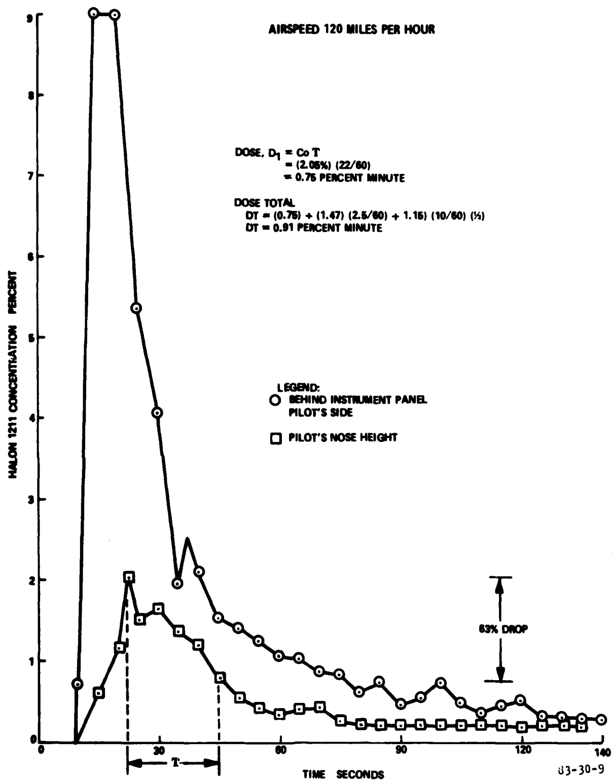
FIGURE 9. HALON 1211 CONCENTRATIONS - 2.5 POUND EXTINGUISHER DIRECTED UNDER INSTRUMENT PANEL - PILOT'S SIDE - OVERHEAD VENTS OPEN (DOSE TOTAL 0.91 PERCENT MINUTE)
