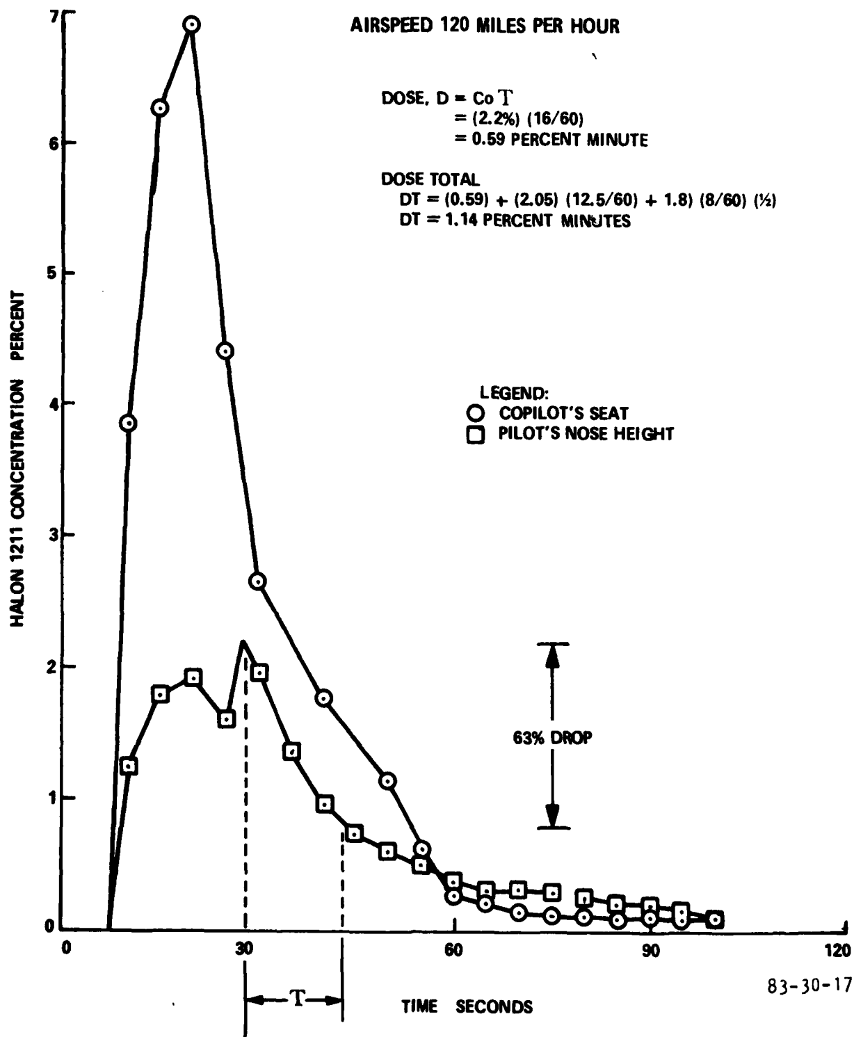
FIGURE 17. HALON 1211 CONCENTRATIONS - 2.5 POUND EXTINGUISHER DIRECTED TO THE COPILOT'S SEAT - OVERHEAD VENTS OPEN (DOSE TOTAL 1.14 PERCENT MINUTE)
