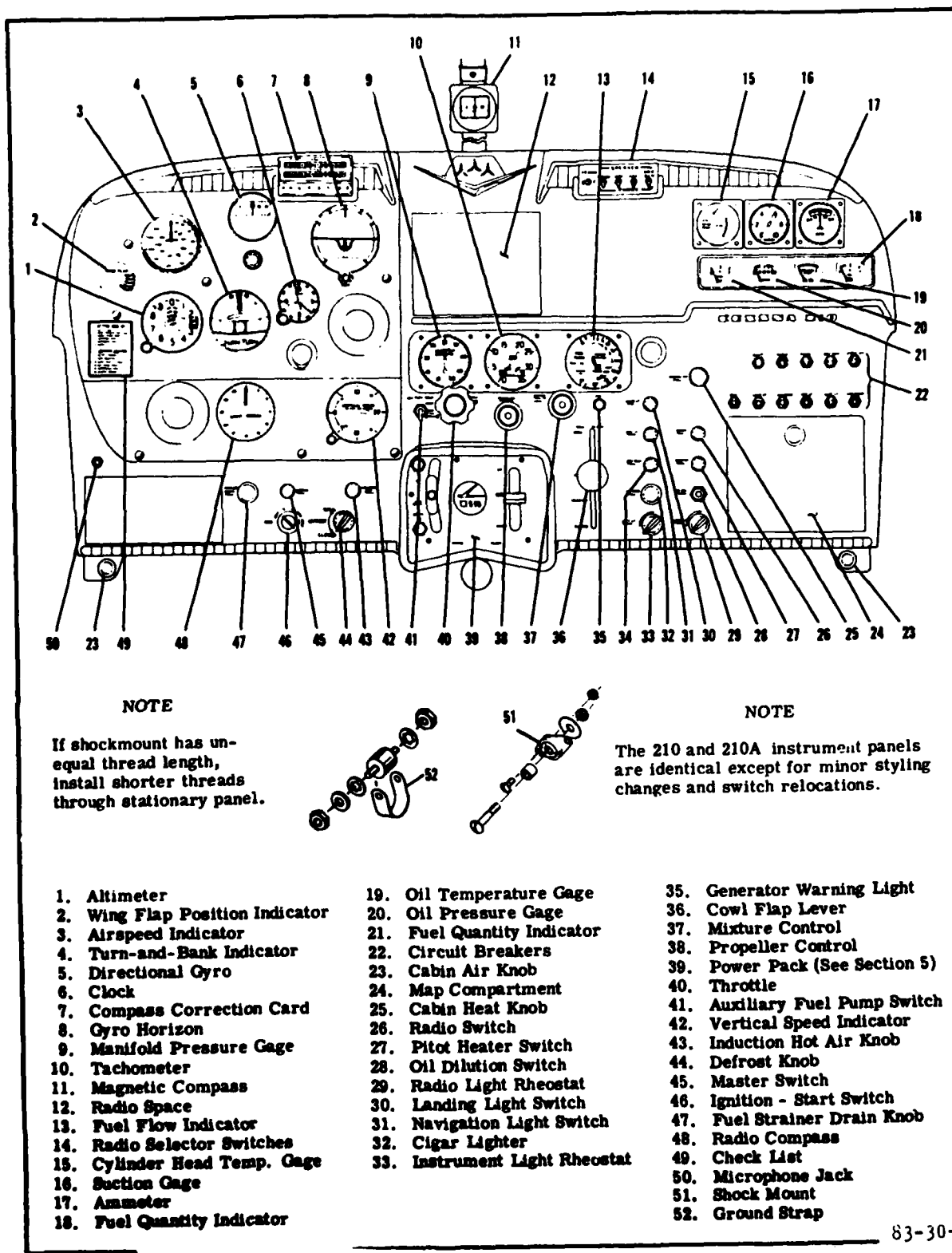
FIGURE 4. INSTRUMENT PANEL - CESSNA MODEL 210C AIRPLANE
