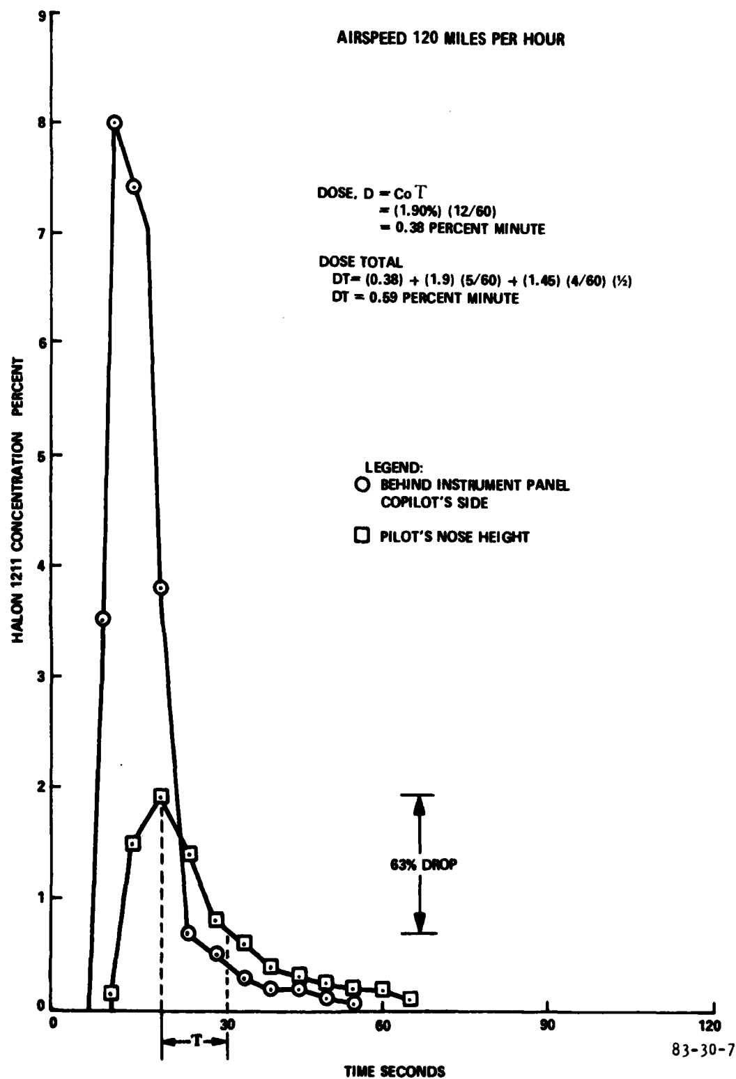
FIGURE 7. HALON 1211 CONCENTRATIONS - 2.5 POUND EXTINGUISHER DIRECTED UNDER INSTRUMENT PANEL - COPILOT'S SIDE - ALL VENTS OPEN
