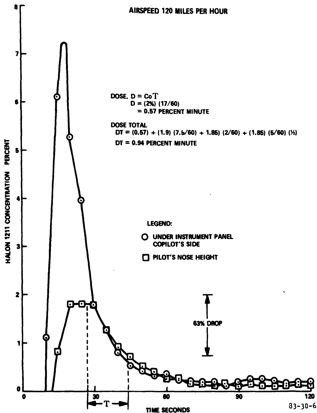
FIGURE 6. HALON 1211 CONCENTRATIONS - 2.5 POUND EXTINGUISHER DIRECTED UNDER INSTRUMENT PANEL - COPILLOT'S SIDE - OVERHEAD VENTS OPEN (DOSE TOTAL 0.94 PERCENT MINUTE)
