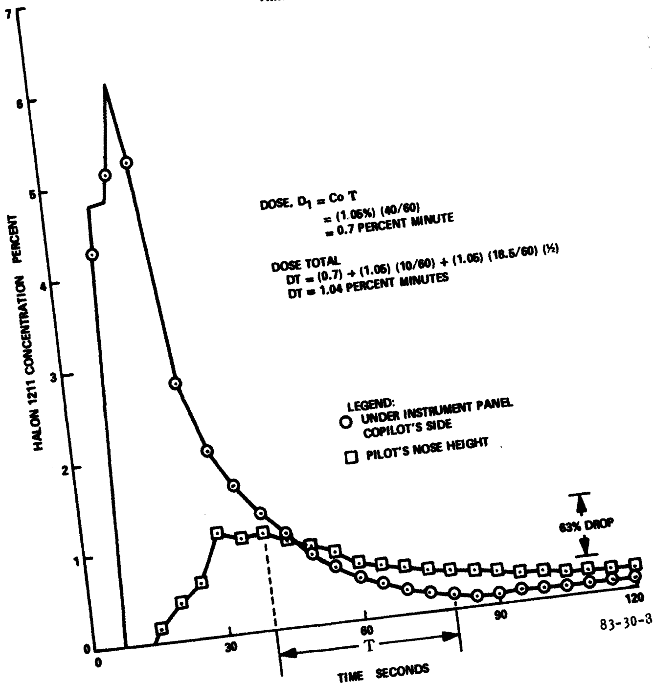
FIGURE 8. HALON 1211 CONCENTRATIONS - 2.5 POUND EXTINGUISHER DIRECTED UNDER INSTRUMENT PANEL - COPILOT'S SIDE - ALL VENTS CLOSED
