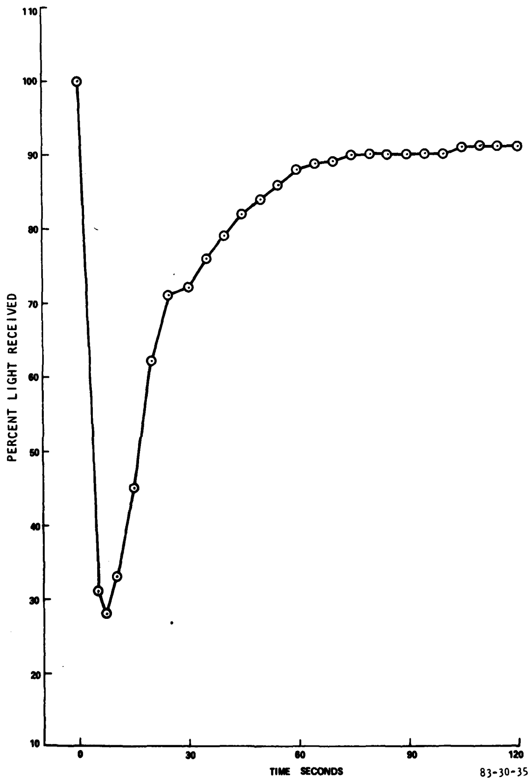
FIGURE 35. SPOTMETER MEASUREMENTS - 2.5 POUND CHEMICAL POWDER EXTINGUISHER DIRECTED TO THE COPILOT'S SEAT
