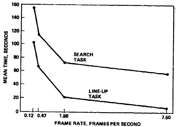
Figure 32. Effects of Video Frame Rate on Target Search and Target Line-up Task Time
