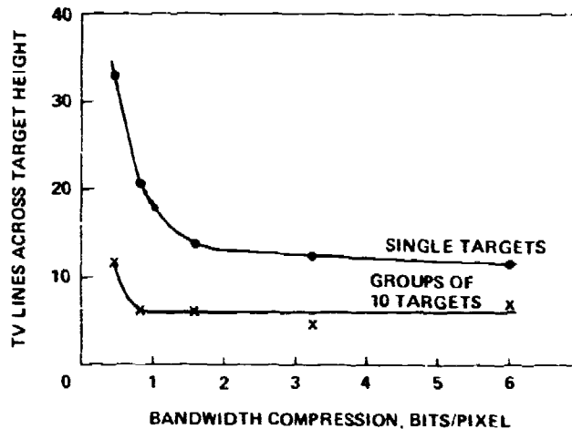
Figure 15. Interaction Between Bandwidth Compression And Target Numerosity For Target Detection Performance
