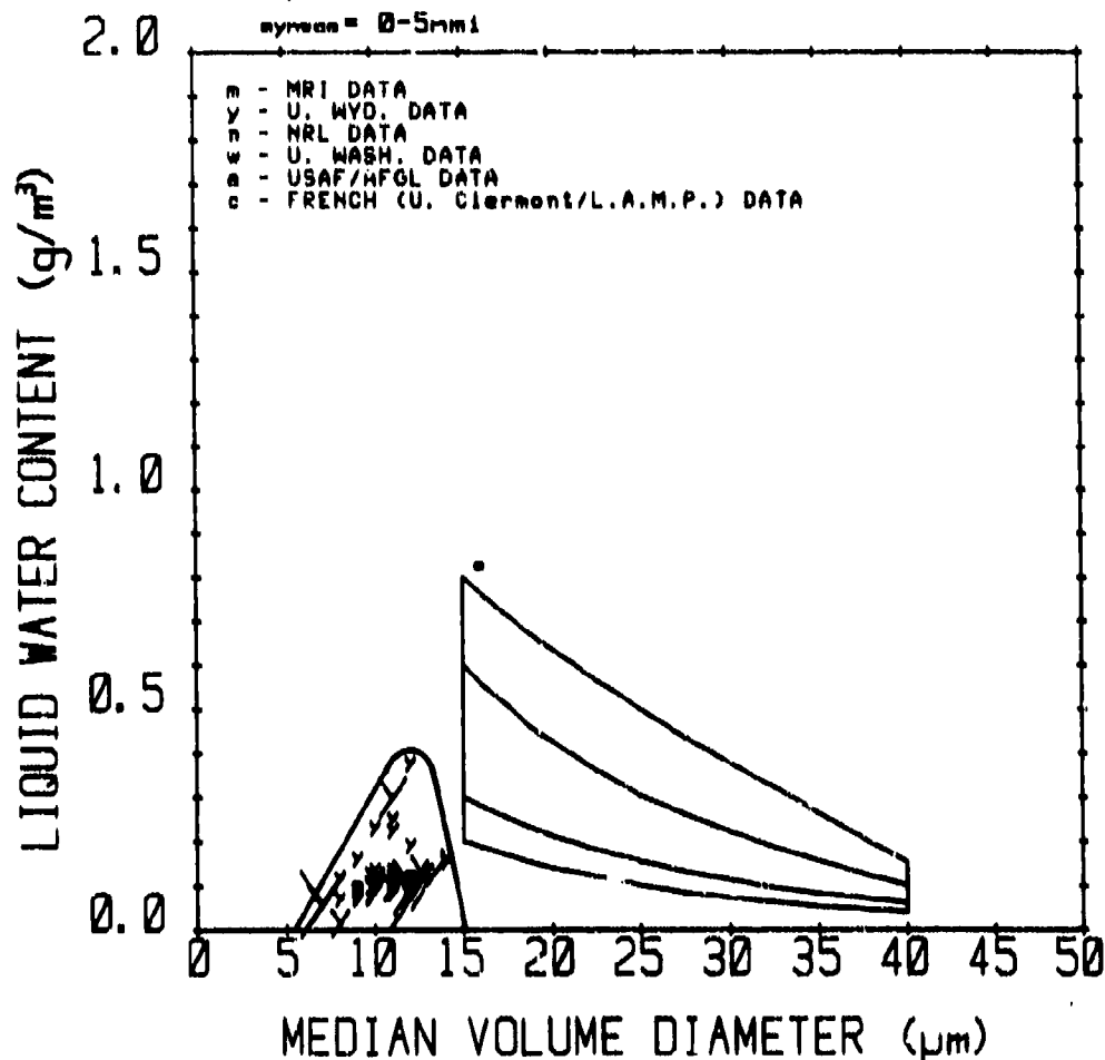
FIGURE 26. SCATTERPLOT OF OBSERVED LWC, MVD COMBINATIONS IN THE MODERN DATA FOR LAYER CLOUDS UP TO 10,000 FT AGL AND FOR CLOUD TEMPERATURES FROM -30°C to -20°C. The various plotting symbols represent different data sources as indicated in the key. The size of each plotted symbol is proportional to its statistical weight (i.e., the observed horizontal extent of the associated icing event) as shown by the scale above the graph. The center of each plotted symbol corresponds to the average (and approximately constant) value of LWC and MVD observed during the icing event. Values of LWC for which no MVD measurements are available are plotted arbitrarily at 1 μm MVD. A total of 174 data miles is represented in this graph. The Continuous Maximum envelope from FIG. 1 of FAR-25, App. C, is superimposed for comparison. The other smooth curve is the observed, apparent limit to the CONUS data for this temperature interval.
