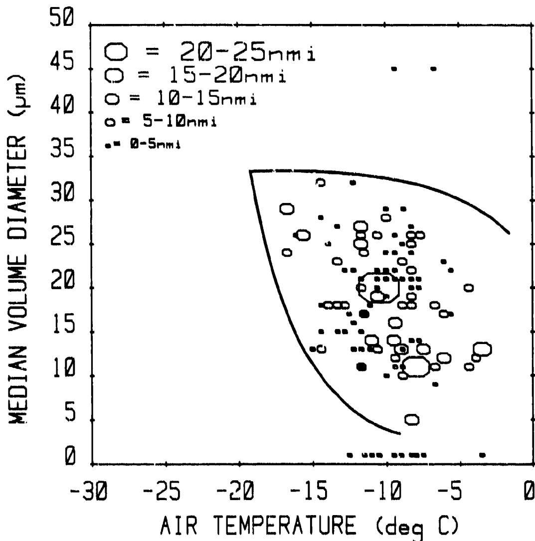
FIGURE 41. SCATTERPLOT OF MVD VS. OAT FOR NACA (1946-1950) DATA FROM SUPERCOOLED CONVECTIVE CLOUDS ( C_u , C_b ) UP TO 10,000 FT AGL. The size of each symbol is proportional to its statistical weight (i.e., the observed horizontal extent of the associated icing event) as shown by the scale above the graph. The center of each symbol corresponds to the average (and approximately constant) value of MVD and OAT observed during the icing event. The solid line bounding the data points represents the apparent upper and lower limit to MVD as a function of temperature for supercooled convective clouds below 10,000 ft AGL. The position of the line is based on extreme MVD values in both the NACA and modern data sets. The data points plotted at 1\ \mu\text{m} MVD are those for which the MVD values are actually unknown. A total of 620 data miles is represented in this graph.
