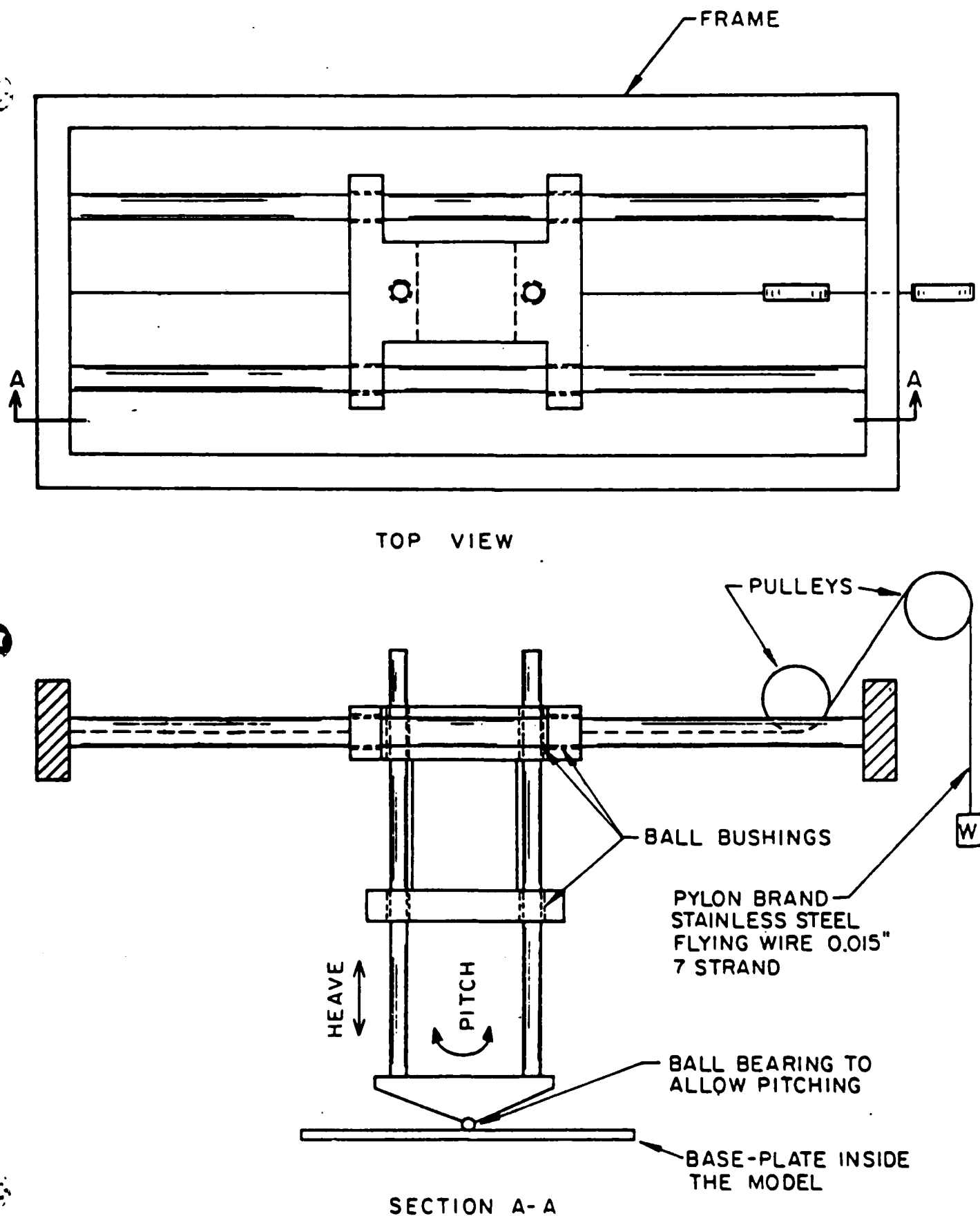
Figure 9. Schematic View of the Constant Force Dynamometer
