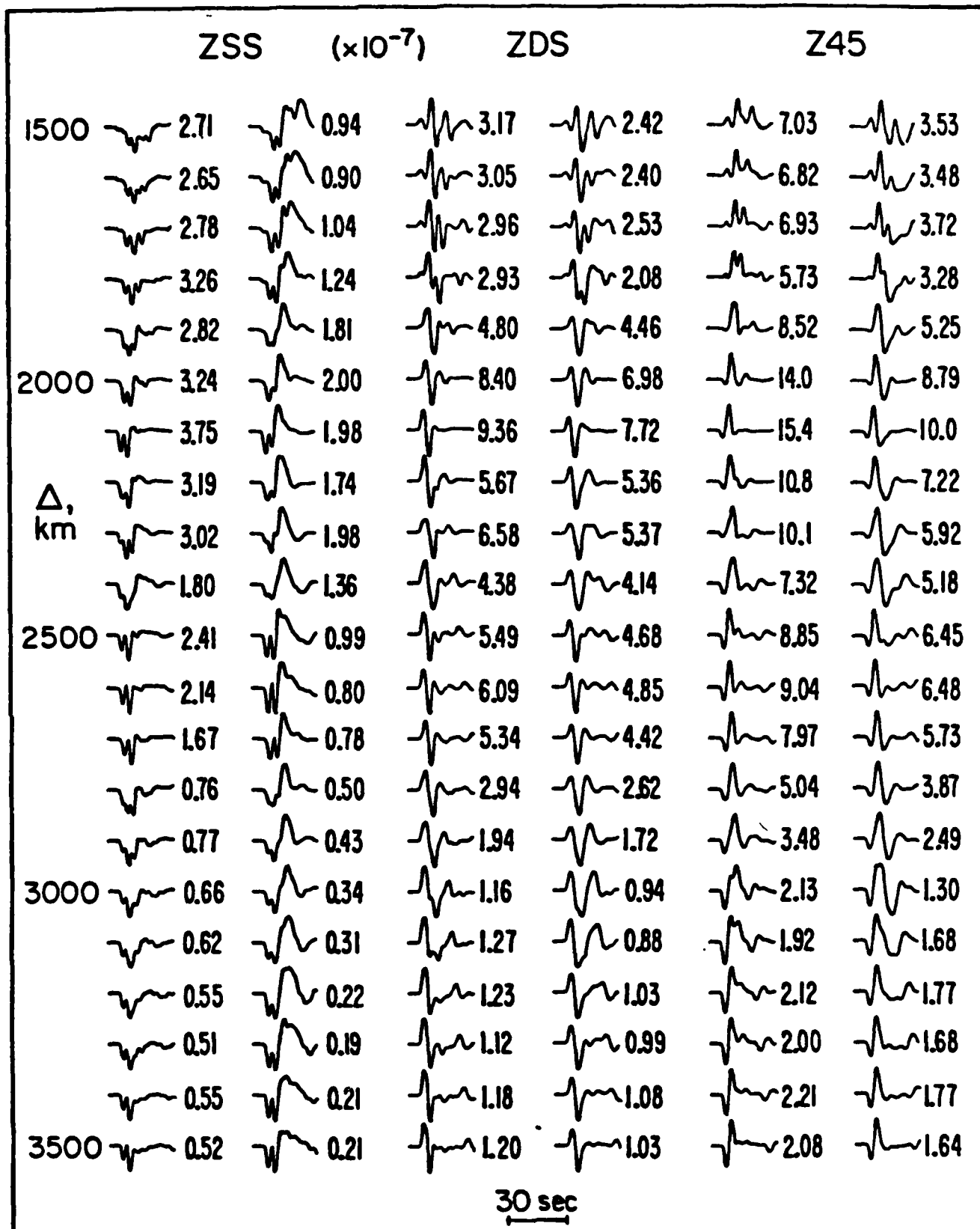
Fig 4.13 - Upper-mantle synthetics without and with instrument for the three fundamental orientations assuming a source depth of 8 km, t^*=1 , and \delta t_1 = \delta t_2 = \delta t_3=1 for the source time history.
