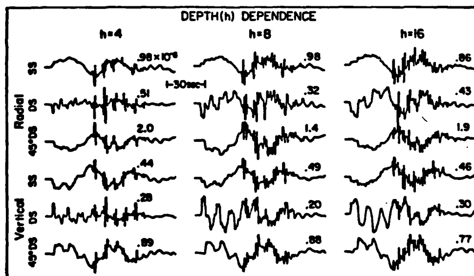
Fig 4.3 - Motions of all three types of faults at \Delta = 1000 km as a function of source depth. The numbers above each trace indicate the zero to peak amplitude in centimeters assuming M_0 = 4\pi\rho \times 10^{20} dyne-cm and trapezoidal time history (0.5, 0.5, 0.5 sec).
