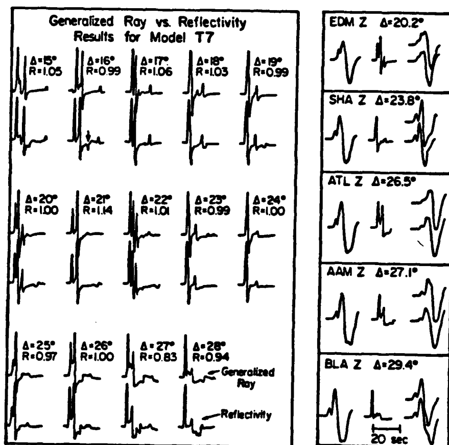
Fig 4.12 - (a) The slightly smoothed delta function responses from a reflectivity calculation (bottom) are compared to those from a generalized ray (top) for model T7. (b) First column contains the predicted waveshape due to the source only; second column is the delta function response of the model T7; third column is the convolution of the first two columns. The observed waveforms from the Borrego Mountain earthquake are on the top for comparison.
