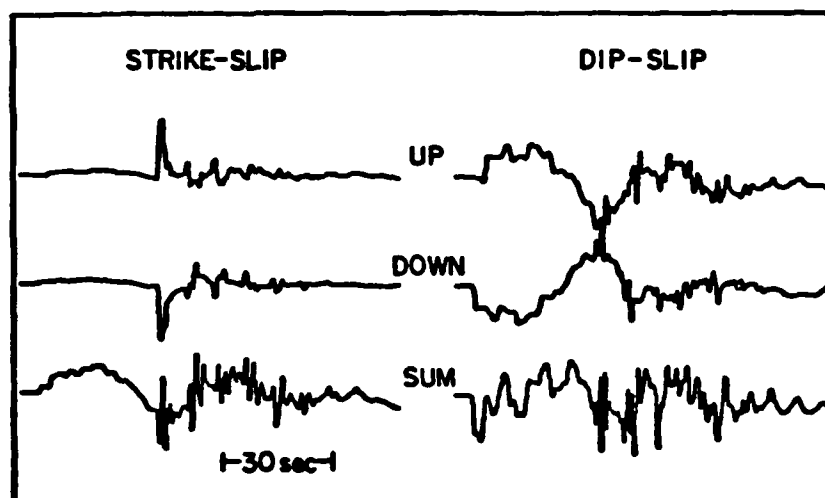
Fig 4.2 - Radial components of motion at \Delta = 1000 km in terms of upgoing, downgoing, and summed for trapezoidal time history (0.5, 0.5, 0.5 sec).
