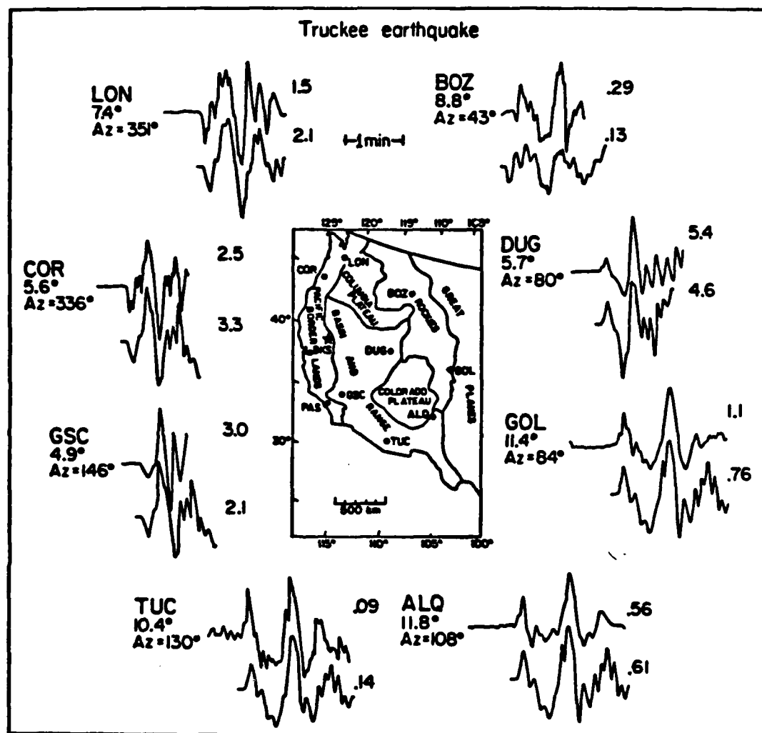
Fig 4.6 - The vertical P_n waveforms of the 1966 Truckee earthquake. The star denotes the epicenter. The data is the top trace at each station and the trace below is the synthetic fit. The strike-slip mechanism has two nodal planes which project through TUC and BOZ. To the right of each trace is the observed or predicted amplitude (on the basis of M_0 = .8 \times 10^{25} dyne-cm) in 10^{-3} cm.
