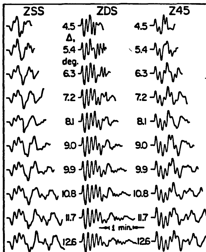
Fig 4.5 - Theoretical displacement profiles for the vertical component. The Green's functions were computed from the model presented in Table 1 and have been convolved with a source time function represented by a trapezoid ( t_1=1 , t_2=1 , t_3=1 ), a triangular filter (2 second rise and fall), and a WWSSN long-period instrument.
