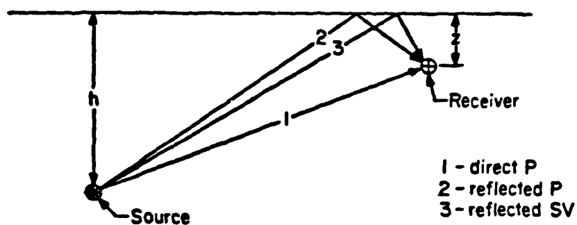
Fig A3 - Schematic showing the interaction of the three arrivals that form the receiver function.
