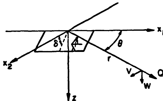
Fig 2.4 - Coordinate system for the dislocation formulation where ( \theta ) indicates the strike, ( \delta ) the dip of the hanging wall, and ( \lambda ) the motion of the hanging wall relative to the footwall.
