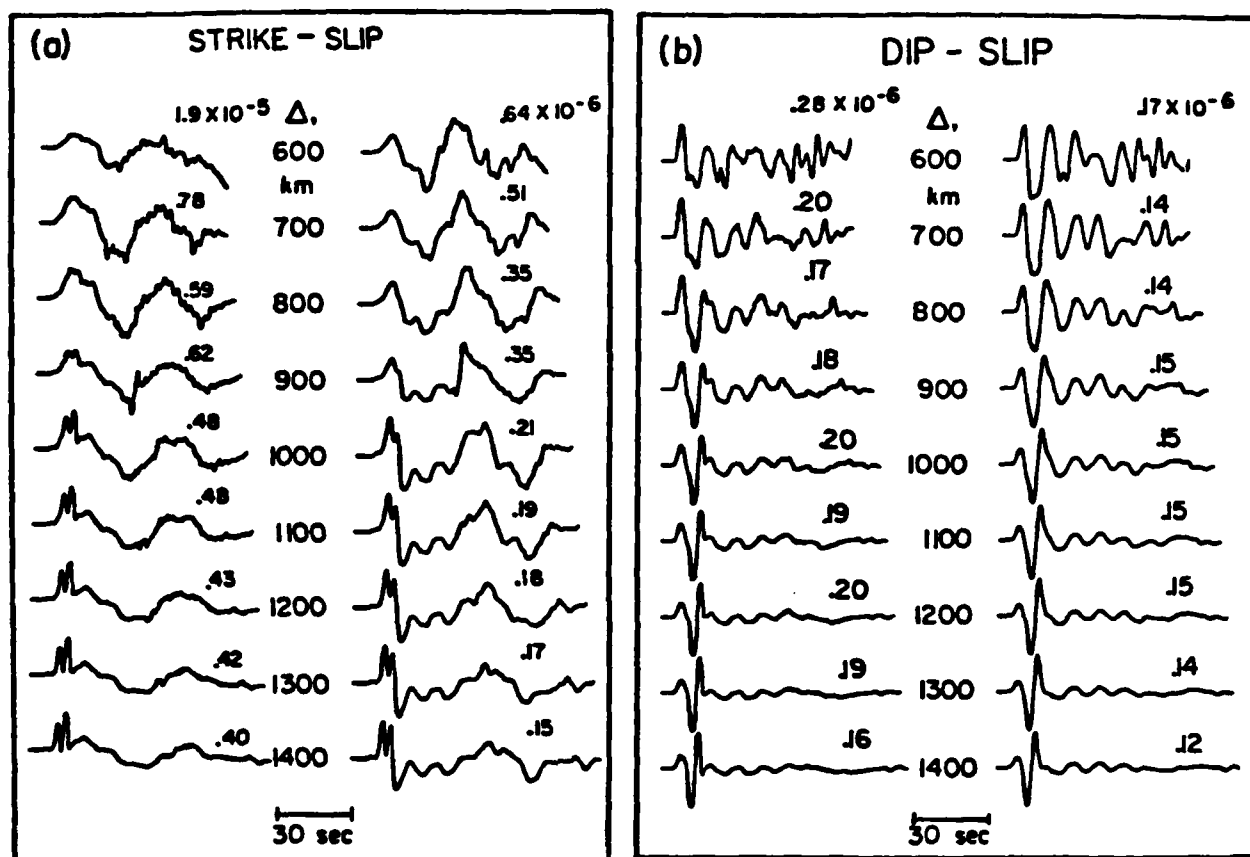
Fig 4.11 - (a) Strike-slip excitation going from P_{NL} domination to P and long-period synthetics. (b) Dip-slip excitation going from P_{NL} domination to P and long-period synthetics.
