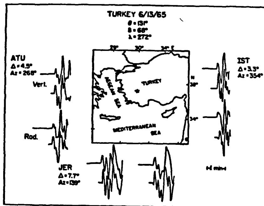
Fig 4.8 - Location of the Turkey event (star) and the recording stations. The filtered data and synthetics for both the vertical and radial components are shown (After Wallace and Helmberger, 1982).
