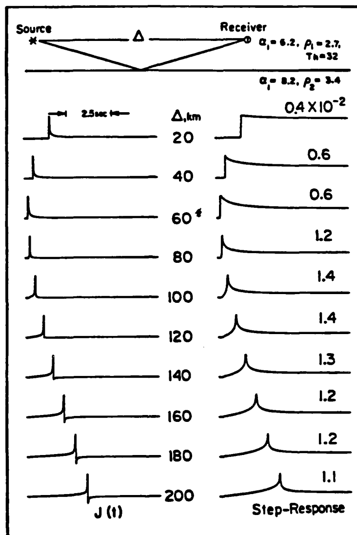
Fig 2.3 - The responses of J(t) and \phi(t) as a function of source-receiver separation. Note that the graphical convolution operator at the larger ranges has two parts: before t = R/\alpha_1 , the square-root singularities are congruent and produce a log similarity at t = R/\alpha_1 ; the second part corresponds to a weighted step response as in figure 2.2.
