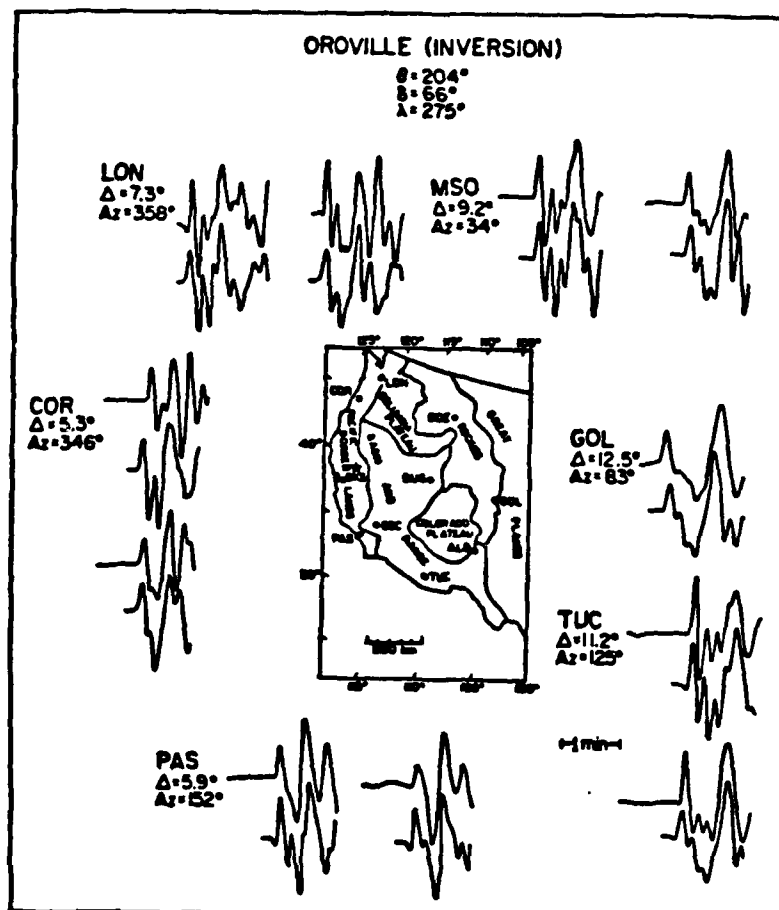
Fig 4.7 - Filtered data and synthetics from the Oroville earthquake. At all the stations except GOL both the vertical (the first trace pair) and radial components are shown.
