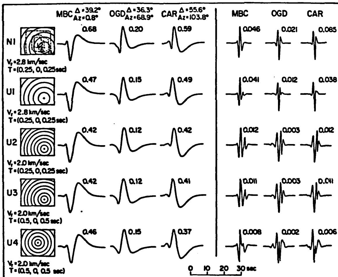
Fig 5.2 - Comparison of the short-period and long-period synthetics at the teleseismic stations for various fault models. The numbers are the amplitudes in micrometers calculated for the seismic moment of .5 \times 10^{24} dyne-cm. The top row corresponds to a particular distribution of faulting appropriate for the Coyote earthquake where the dislocation is largest at the center and tapers down at the edges. The U1, U2, U3, and U4 models show uniform slip histories but with different rupture speeds (After Liu and Helmberger, 1982).
