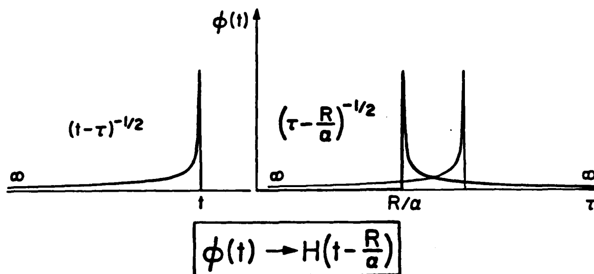
Fig 2.2 - Schematic diagram explaining the convolution operation by graphical means. We reverse the direction of the square-root operation and perform the multiplication of the two functions for values of \tau from (0) to (t) and sum. The results are zero until the two functions overlap.
