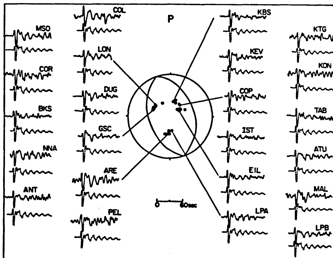
Fig 3.6 - Focal mechanism plot showing the P-first motions for the Bermuda earthquake, March 24, 1978. Observed (upper) and synthetic (lower) P wave traces from the vertical long-period WSSN seismograms for stations shown in Figure 1. Note an initial simple event followed by more complicated water reverberations (After Stewart and Helmberger, 1981).
