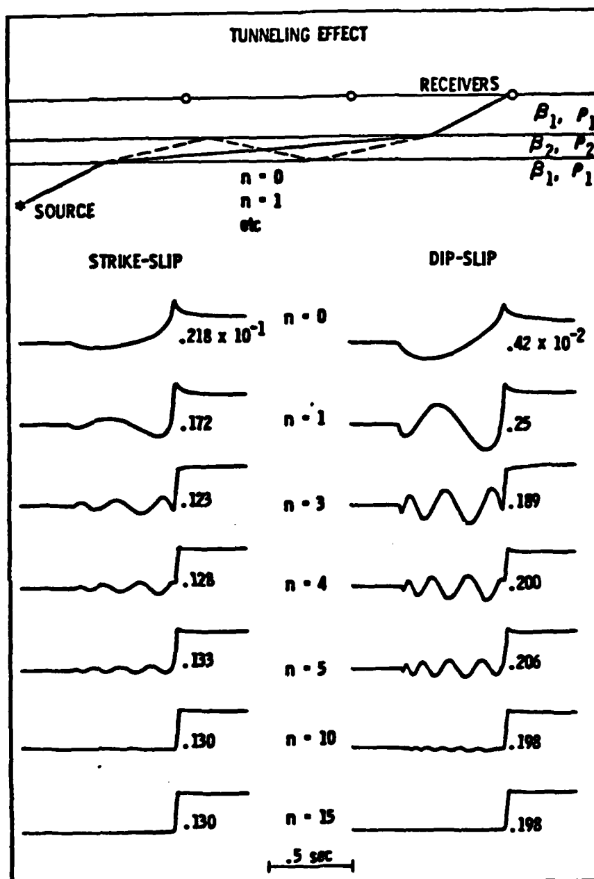
Fig A2 - Numerical step response of tunneling. The source depth is 3 km with a 20 km source-receiver separation. Seismic parameters are \rho_1 = 2.3 \text{ gm/cm}^3 , \beta_1 = 2.02 \text{ km/sec} , and \rho_2 = 2.4 \text{ gm/cm}^3 , \beta_2 = 2.31 \text{ km/sec} , with a barrier thickness of 10 meters. Relative peak amplitudes are given for each case. n indicates the number of rays included in the sum.
