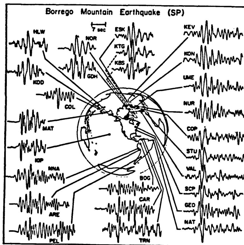
Fig 5.1 - Short-period P waveforms recorded at WSSN stations. Note the coherence of the first several seconds of the waveforms from stations at similar azimuths. The star denotes the location of the earthquake (After Ebel and Helmberger, 1982).
