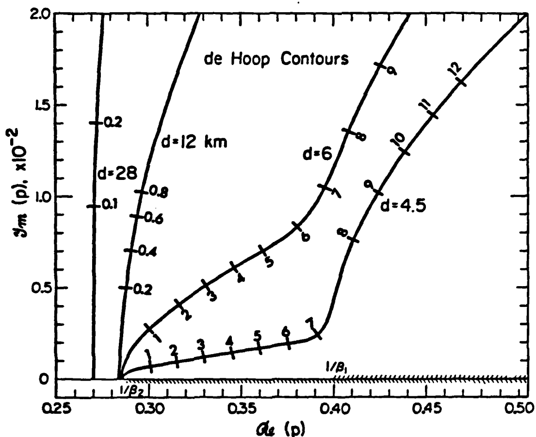
Fig 2.6 - Contours of Im versus Re(p) for the direct rays shown in Figure 2.5. The branch cuts run along the Re(p) coordinate, starting at 1/\beta_2 and 1/\beta_1 , respectively. The parameter time is marked along each contour.
