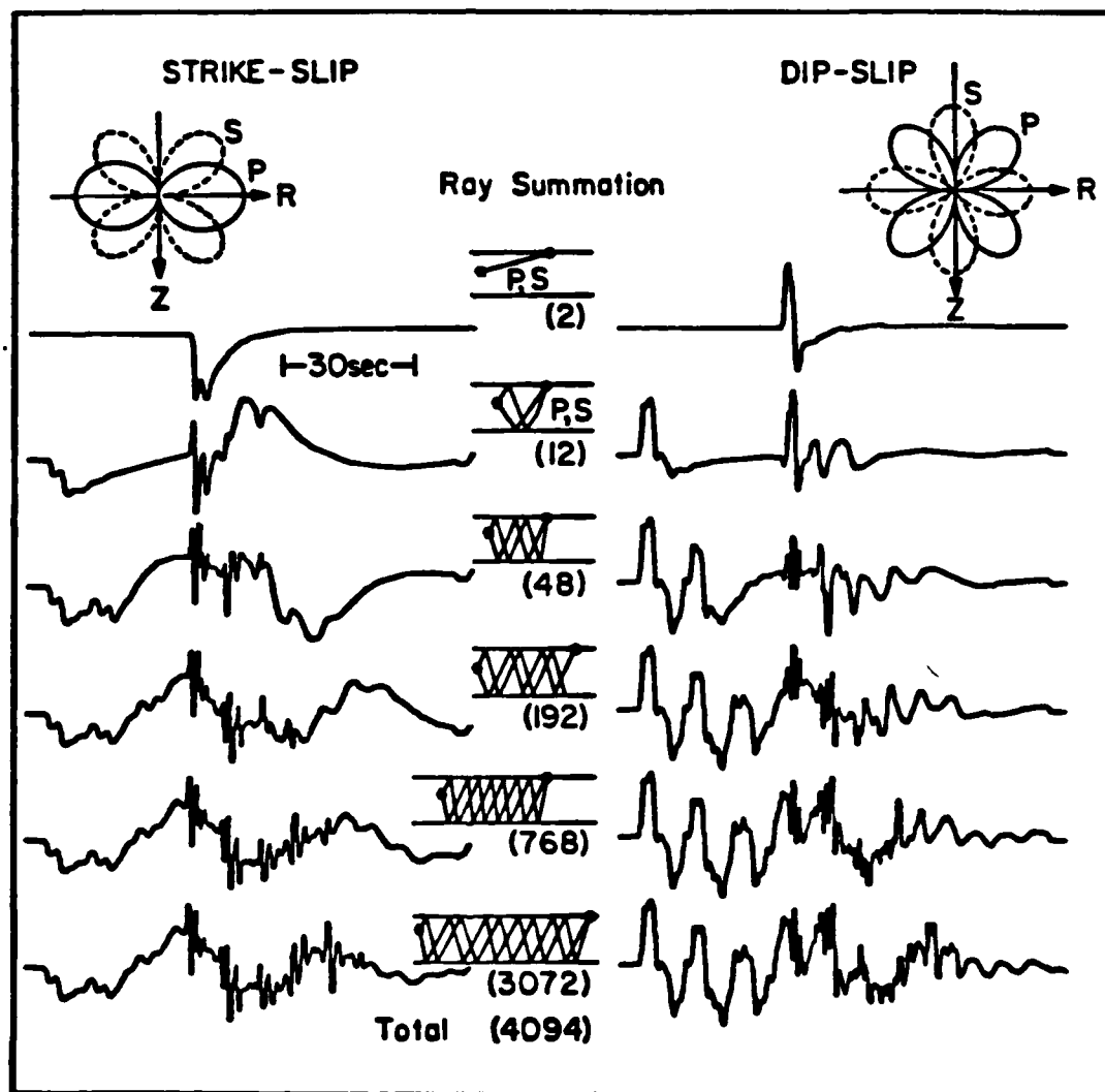
Fig 4.1 - Vertical components of motion as a function of ray summation assuming a trapezoidal time function described by 0.5, 0.5, 0.5, for pure strike-slip and dip-slip orientations at \Delta = 1000 km.
