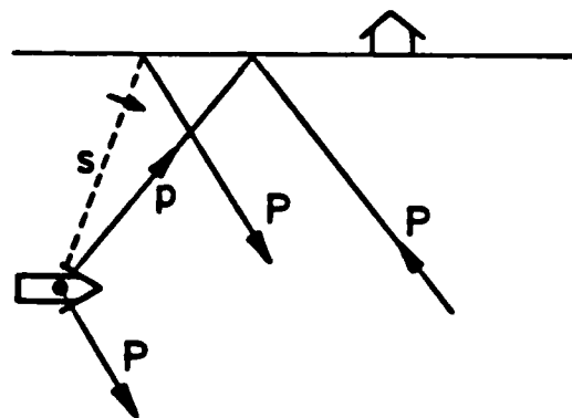
Fig 3.1 - Schematic representation of the phases P , pP , and sP .
