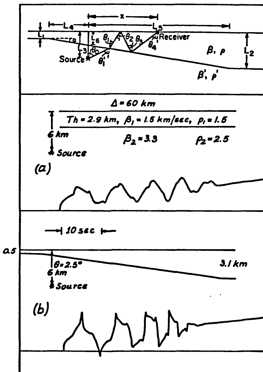
Fig 2.8 - Comparison of the step responses for a flat and dipping layer where the elastic parameters are the same.
