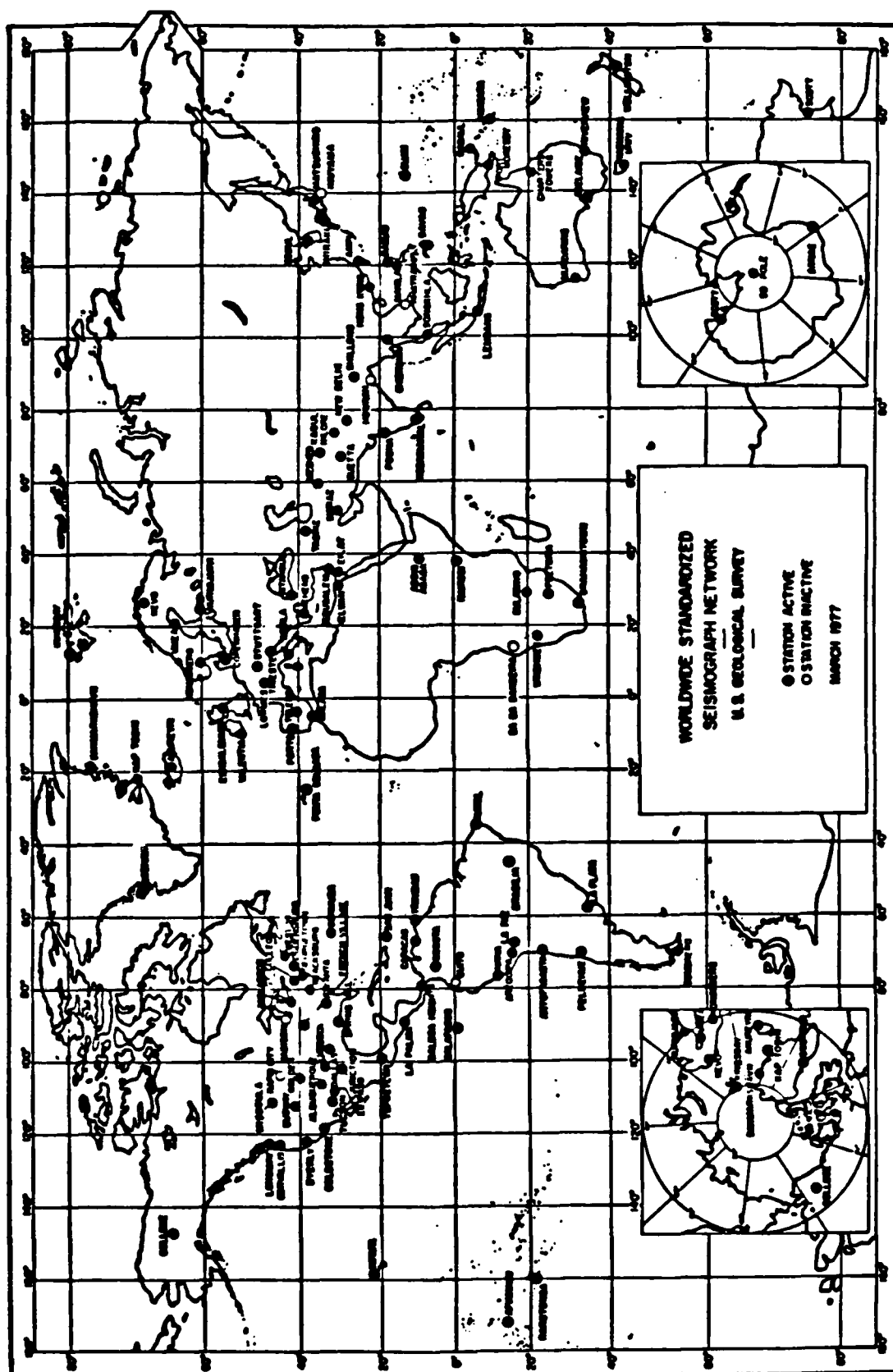
Fig 1.1 - WSSN global network (after USGS).
