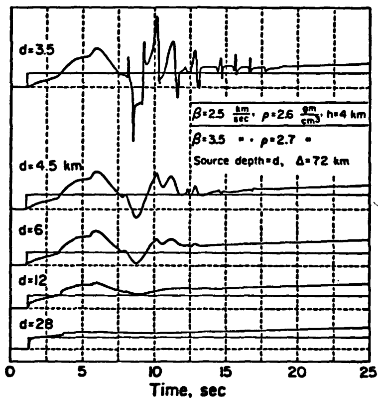
Fig 2.5 - SH step responses at the surface assuming a point strike-slip dislocation situated at various depths. The amplitudes are scaled relative to the top trace with the step response for a homogeneous half-space (bottom properties) displayed for comparison.
