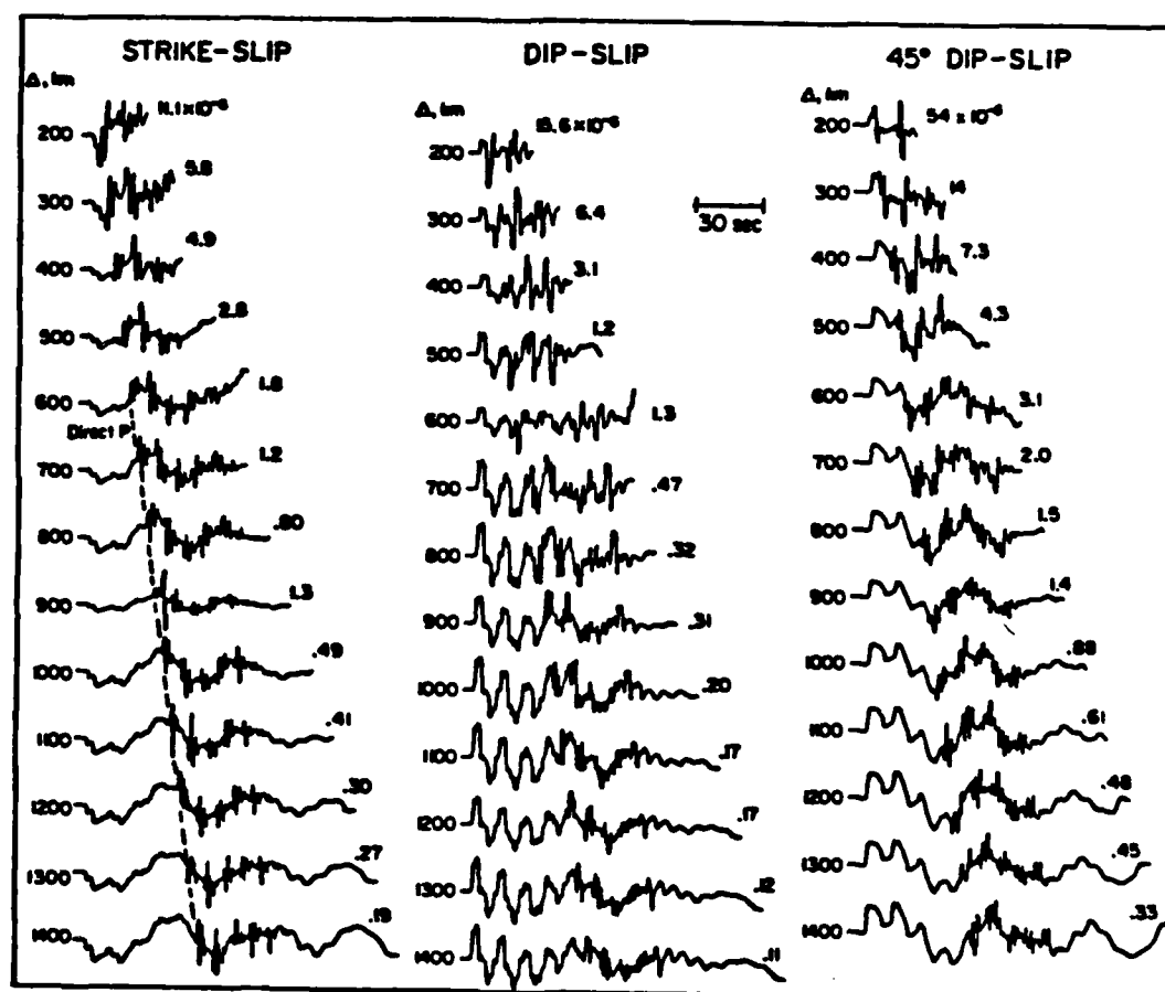
Fig 4.4 - Profiles of the vertical displacements for the three fundamental faults. The numbers above each trace indicate the zero to peak amplitude in centimeters assuming M_0 = 4\pi\rho_0 \times 10^{20} dyne-cm and trapezoidal time history (0.5, 0.5, 0.5 sec). This time history was convolved with the delta function response to reduce the high-frequency spikes created by the post-critical reflections so that the longer periods become more apparent (After Wallace et al. , 1981a).
