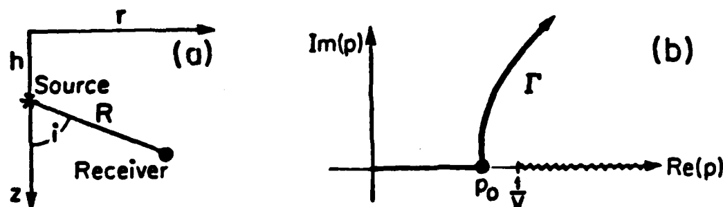
Fig 2.1 - Source-receiver geometry (a) and complex ( p ) plane (b) with branch cut starting at (1/V) and running out along the real ( p ) axis.
