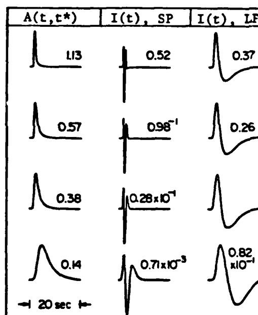
Fig 1.2 - The first column displays A(t, t^*) as a function of t^* assuming 0.5, 1.0, 1.5, and 4, from top to bottom. The middle column displays the convolution of A(t, t^*) with the short period instrumental response, and similarly for the long period on the right. The relative amplitudes are indicated by the numbers above each trace.
