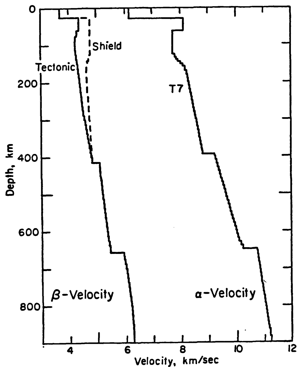
Fig 4.10 - Velocity depth functions for T7 (Burdick and Helmberger, 1978) and two recent shear-wave models (Grand and Helmberger, 1982).
