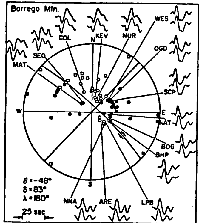
Fig 3.4 - Observed (top) and synthetic (bottom) long period P waveforms at 14 WWSS stations. The P-first motion plot is represented by the equal area stereographic projection of the lower half of the focal sphere. Black dots indicate compression (upward breaking P) and open circles indicate dilatation (downward breaking P). The heavy solid lines denote the nodal planes used in determining the fault orientation, \theta (strike), \delta (dip), \lambda (slip direction). Modified after Burdick and Mellman (1976).
