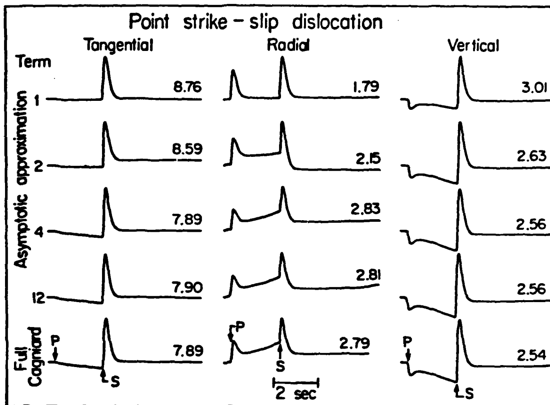
Fig 2.9 - Comparison of the various components of motion for a strike-slip orientation at \Delta = 16 km for a whole space. The top four rows contain the asymptotic summation after 1, 2, 4, and 12 items. The full solution is displayed on the bottom.
