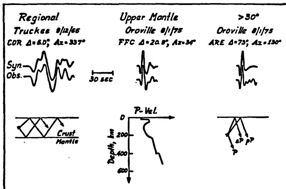
Fig 1.3 - Example observations and synthetics at ranges where the earth appears simple ( > 30^\circ ), slightly complicated (upper-mantle ranges, 30^\circ to 14^\circ ), and quite complicated (less than 14^\circ ).
