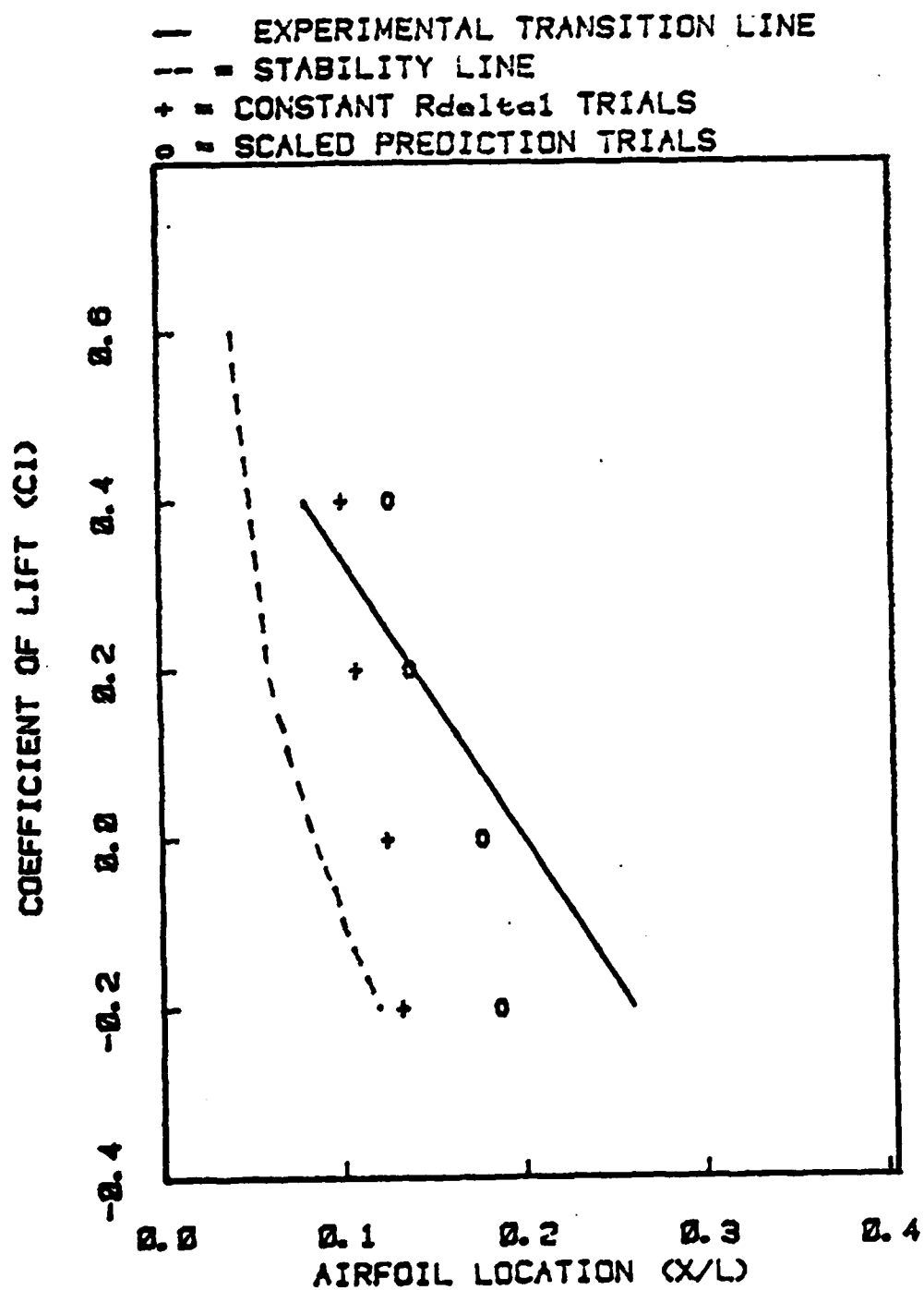
Fig 13 Prediction Trials for R_l=5.0\text{mil.}
