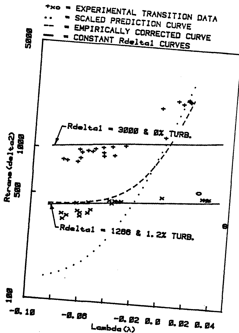
Fig 11 Prediction Curves and Data.
