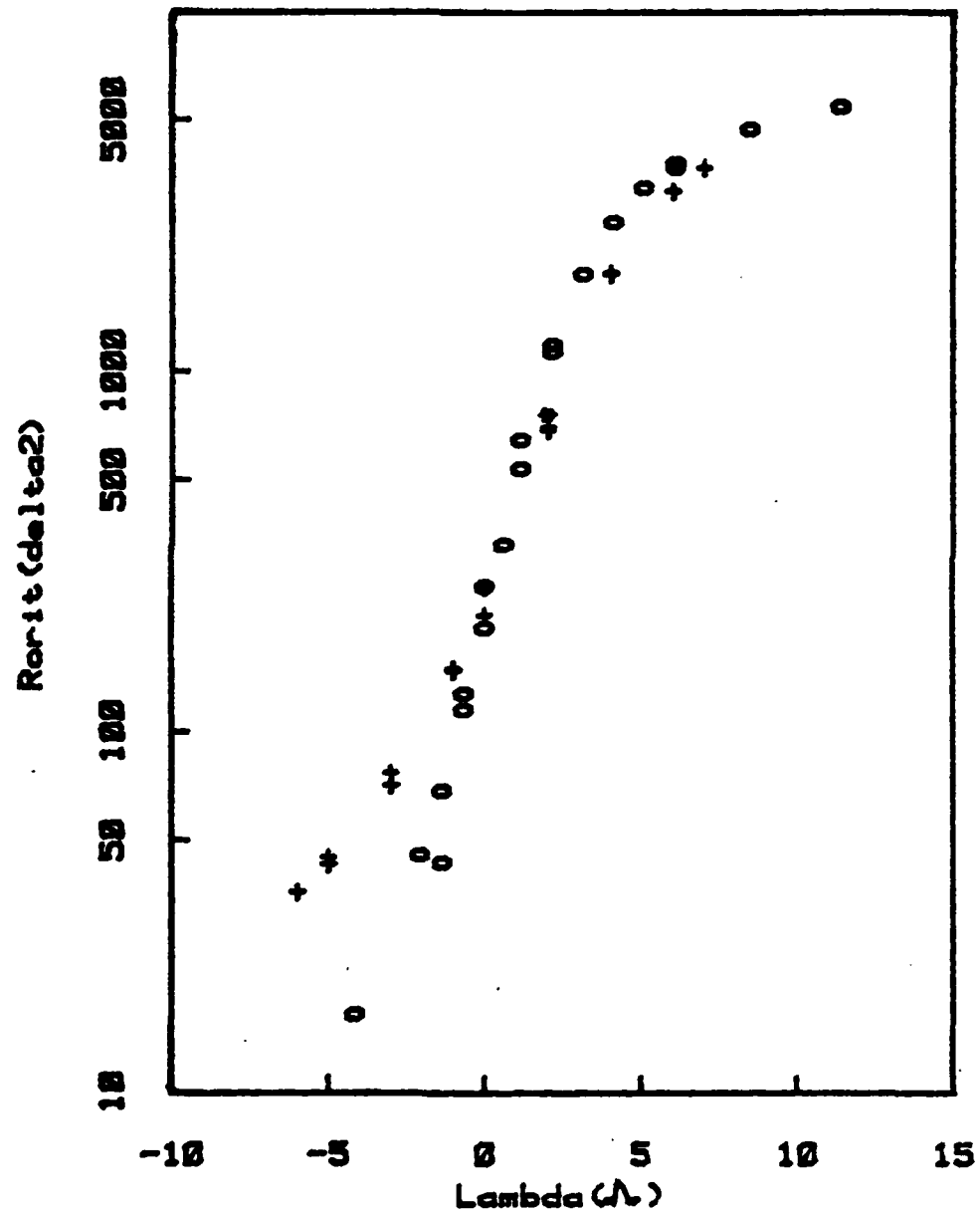
Fig 6 Combined Stability Results.
