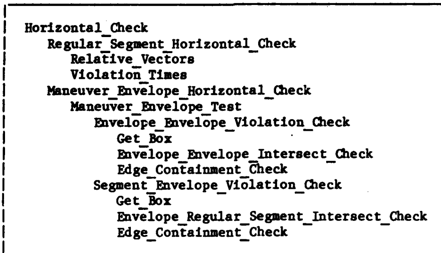
Figure 4-22 shows a PDL representation of the Horizontal Check algorithm.
