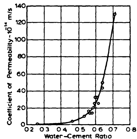
Figure 3. Relationship between permeability and water-cement ratio for mature cement pastes
