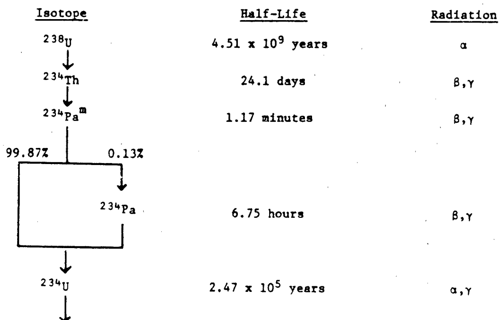
Figure 1: Decay chain of ^{238} -Uranium
