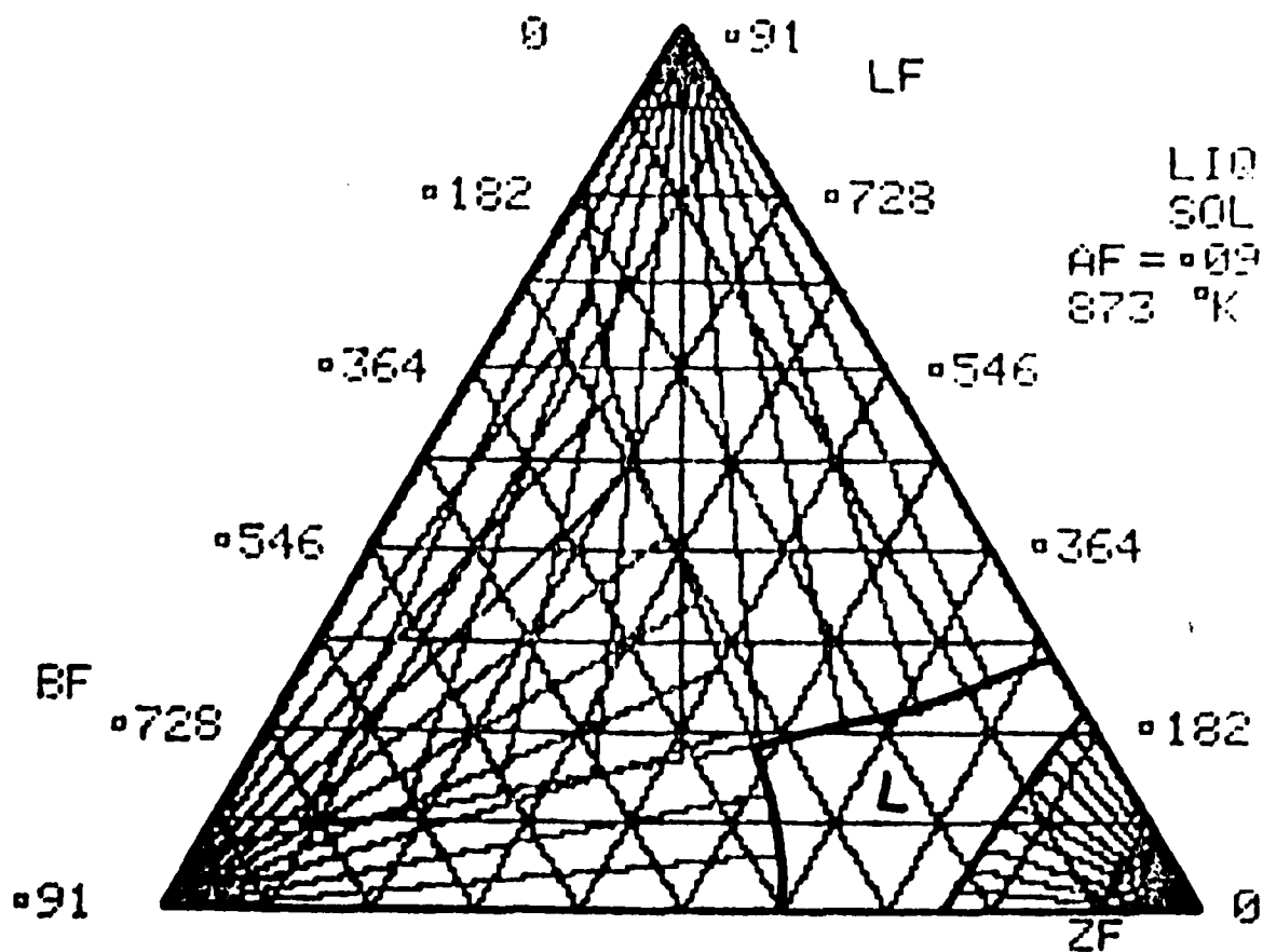
Figure 4 Calculated Solid-Liquid Equilibria in LF-ZF-BF with AF=0.09
