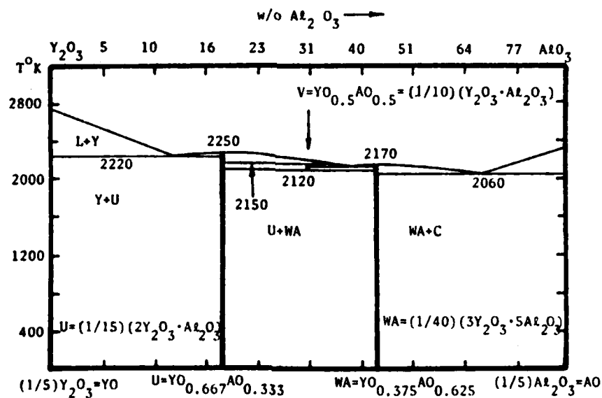
Figure 6. Calculated 1/5\text{Y}_2\text{O}_3 - 1/5\text{Al}_2\text{O}_3 Phase Diagram
