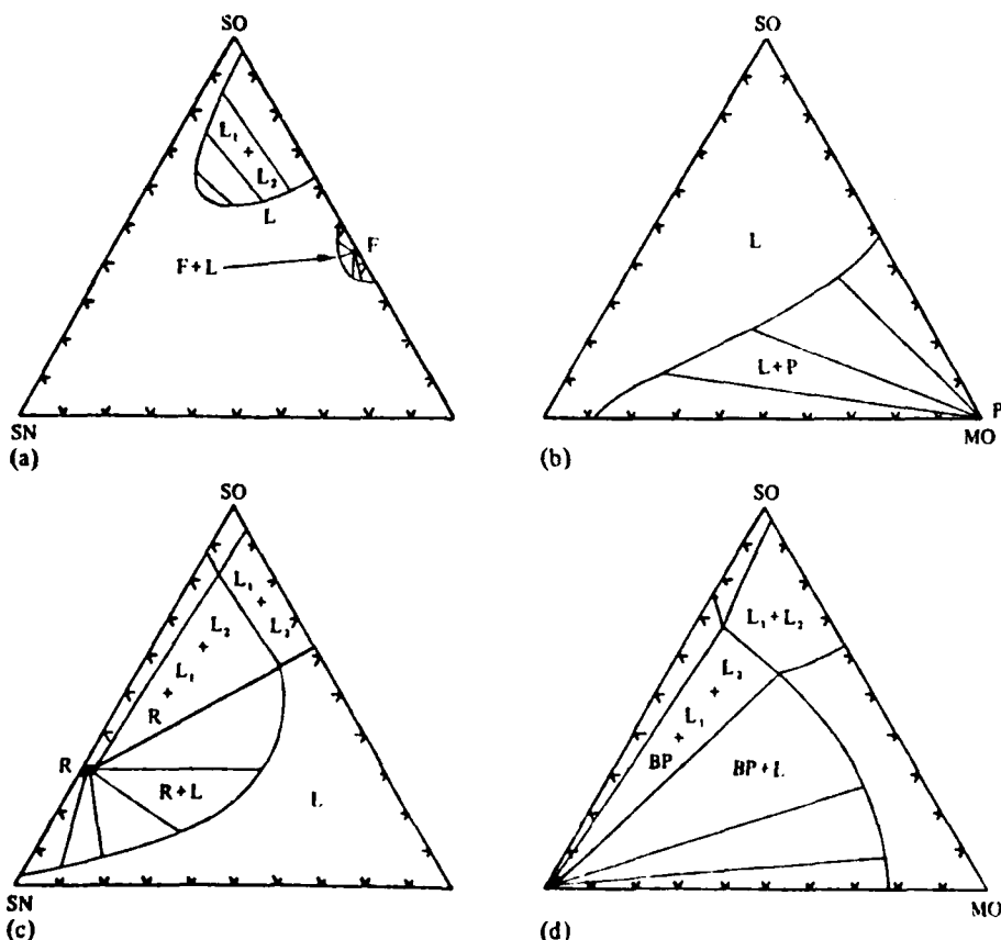
Figure 2. Calculated pairwise equilibria in the \text{SiO}_2\text{-MgO-Si}_3\text{N}_4 system at 2100 K (see tables 1-5 for explanation of symbols). (a) F-L; (b) L-P (P, periclasite); (c) L-R; (d) BP-L.
