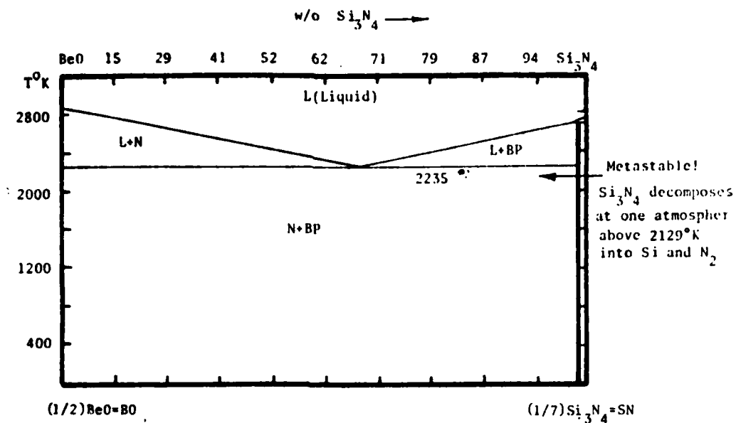
Figure 5. Calculated 1/2\text{BeO} - 1/7 \text{Si}_3\text{N}_4 Phase Diagram
