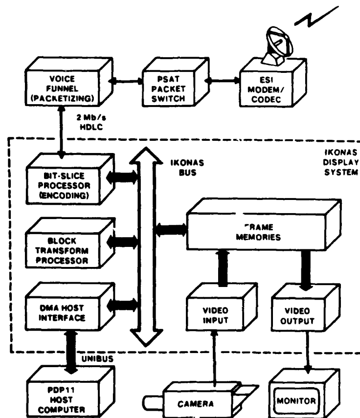
Figure 1: Block Diagram of Real-Time Implementation
