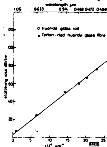
Fig. 2 Fibre spectral scattering loss for a \text{ZrF}_4\text{-BaF}_2\text{-LaF}_3\text{-AlF}_3\text{-LiF-PbF}_2 Teflon-clad fibre
