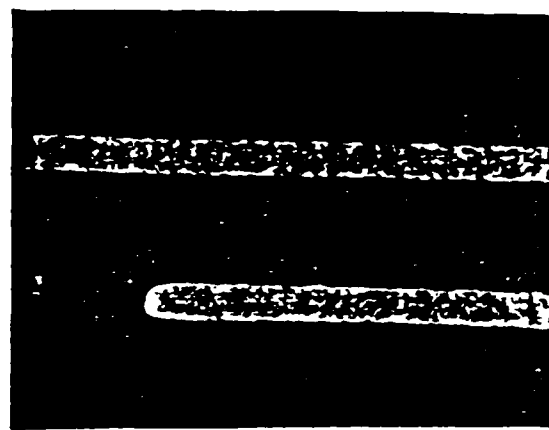
Fig. 3. 960X magnification of 6- \mu m wide lines showing a 6- \mu m period in edge roughness.
