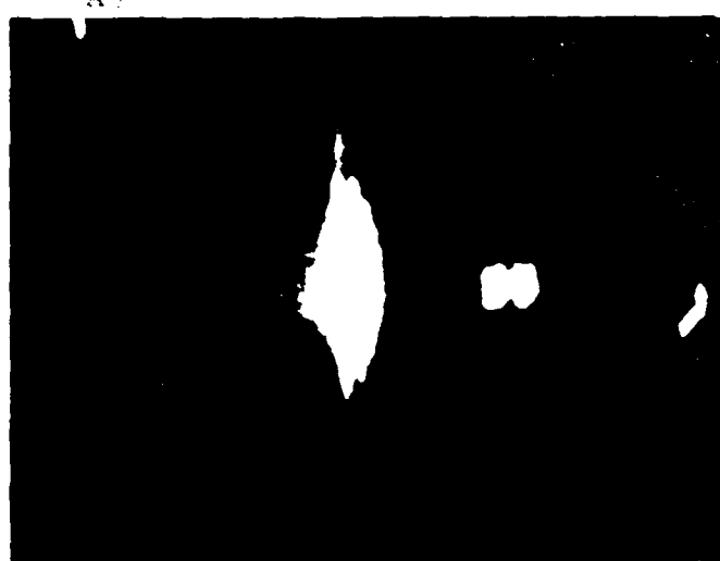
Figure VI-10. Far-field of output prism-coupled waveguide. Fabricated by ion-exchange in a superlattice sample of \text{GaAs}/\text{AlGaAs} of 100\text{ nm} period. A 100\text{ nm} wide waveguide was etched into the surface. The waveguide was coupled to a 100\text{ nm} wide output waveguide.
