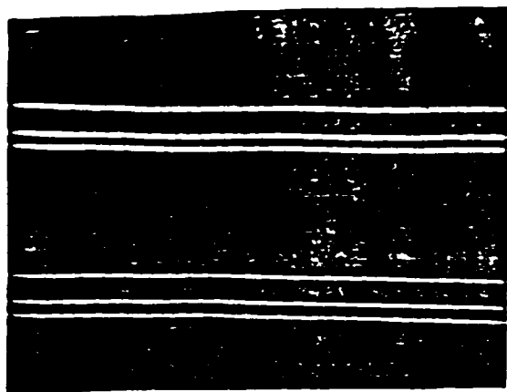
Fig. 2. 204.8X magnification of mask for parallel lines fabricated by laser writing. Lines 4- \mu m (lower group) and 7- \mu m (upper group) wide were written using 40 \mu W and 80 \mu W of laser power, respectively.
