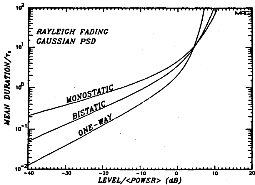
Figure 10. Mean duration of fades below an arbitrary level.
