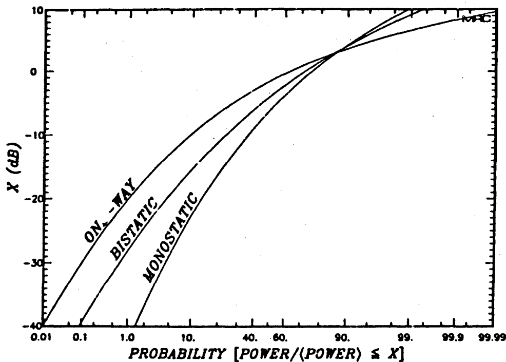
Figure 1. Cumulative distribution of the received power.
