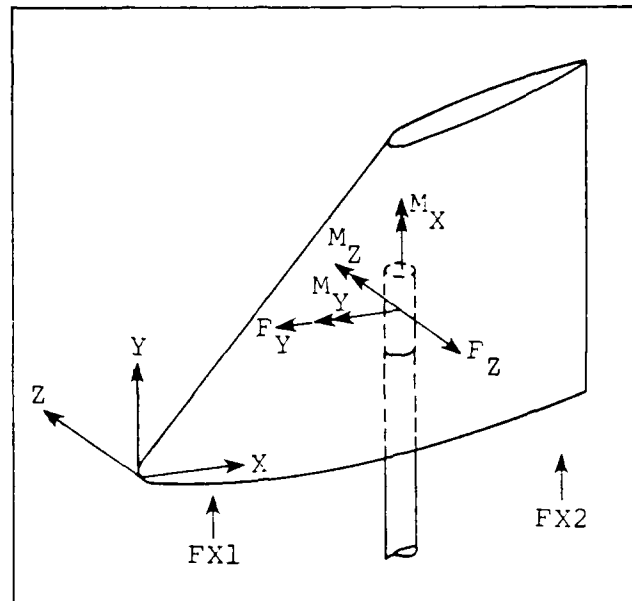
Figure 4.- Wing coordinates and balance force and moment system.
