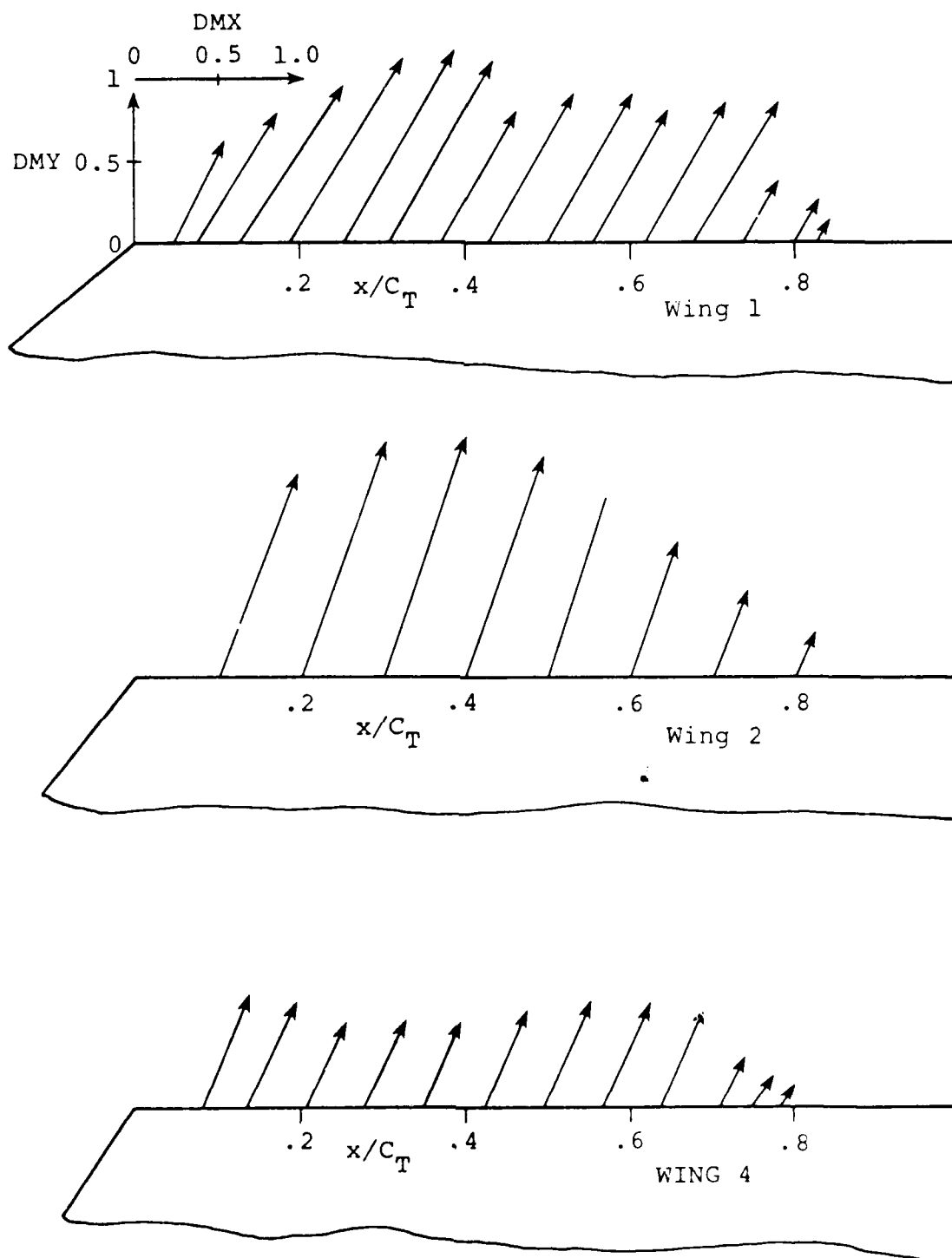
Figure 6.- Tip blowing momentum vectors.
