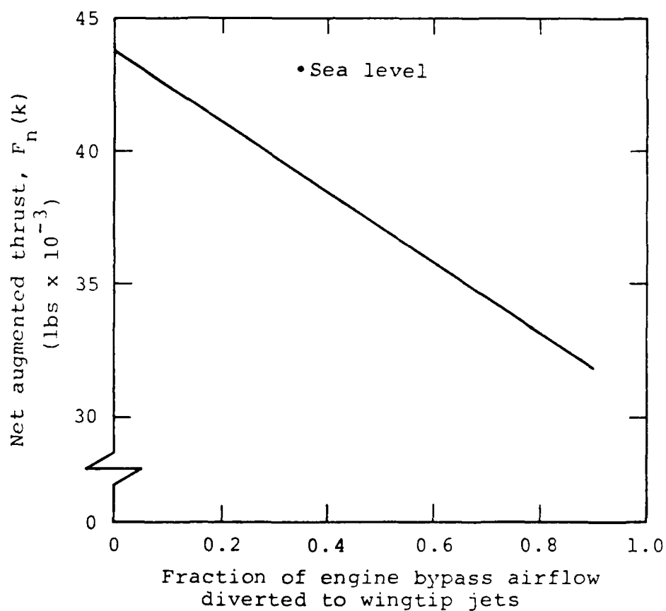
Figure 16.- Thrust degradation due to diverting engine bypass airflow to wingtip jets (engine exhaust nozzle adjusted to provide same exit velocity).
