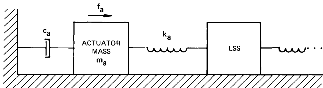
Figure 3-2. Single transmission type actuator.
