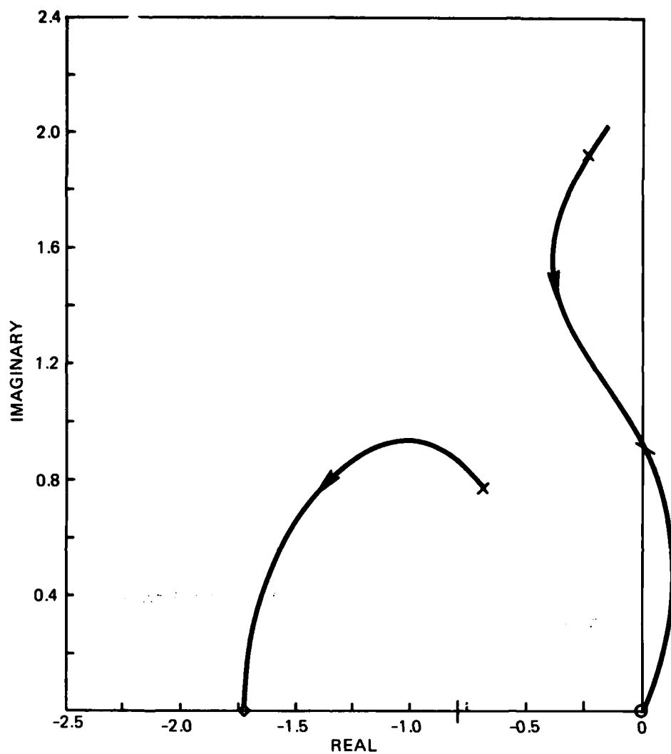
Figure 3-6. Closed-loop root locus.
