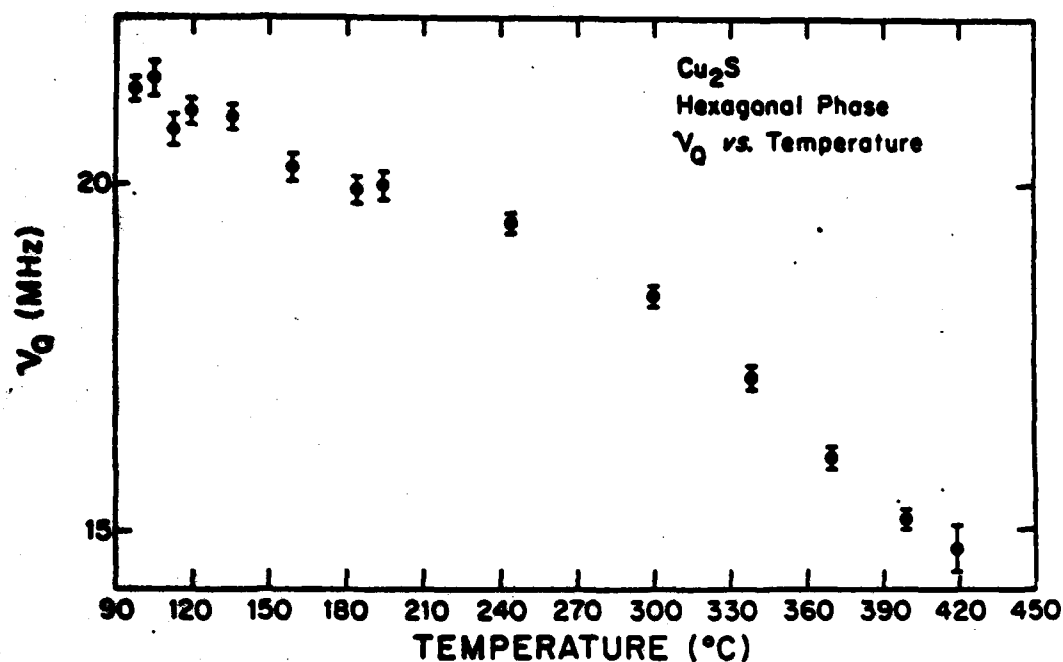
Figure 2. Quadrupolar frequency vs. T for 111 Cd impurities in hexagonal phase Cu 2 S.
