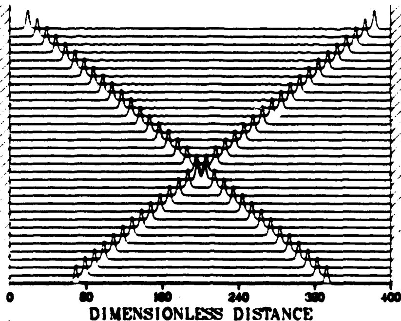
Figure 1 -- Head-on collision of an identical pair of solitary waves of amplitude 0.386. Computations are carried out in a computational channel of 3200 equally-spaced grid points using \Delta x = \Delta t = 1/8 . The profiles shown are equally-spaced in time, starting at the bottom, with the vertical spacing between profiles set so that disturbances that propagate at c_{\text{dimensional}} = \sqrt{gH_0} would be aligned along \pm 45^\circ in the figure.
