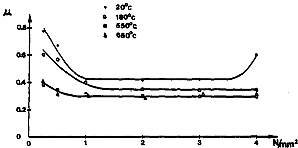
figure 19 : Evolution of the coefficient of friction of Cr_2O_3 sliding against itself in air, versus the apparent contact pressure (5 m/mn, 20 - 180 - 550 - 650°C)
