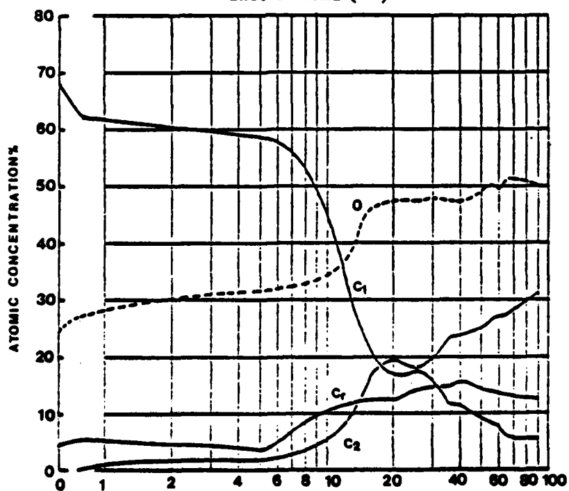
figure 14 : Curve of the atomic concentration of the elements of one point of the surface, versus ionic erosion time : \text{Cr}_7\text{C}_3 -NiCr after testing in air at 900^\circ\text{C} - glazed area
