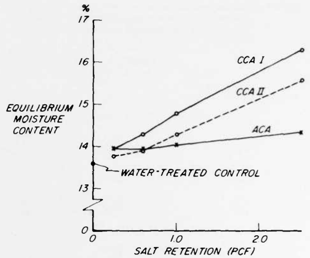
Figure 3.—Effect of preservative systems and retention level on equilibrium moisture content (air-dried and kiln-dried specimens combined). (M 151 583)
