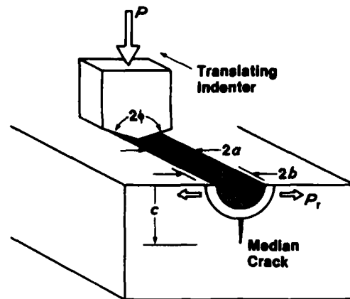
Figure 1 Schematic showing parameters of line flaw system.
