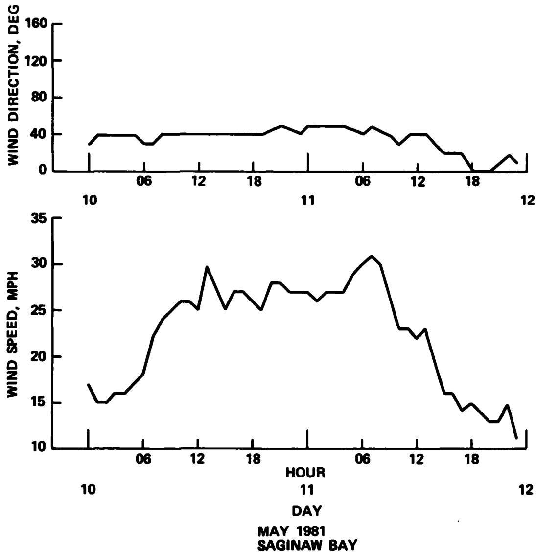
Figure 13. Wind data used for calibration test
