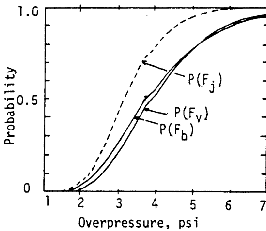
Fig. 3. Probability of Joist Failure
