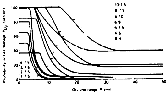
Fig. 3 Fire damage range for various building type contents indices blast induced ignitions W = 1 \text{ Mt}
