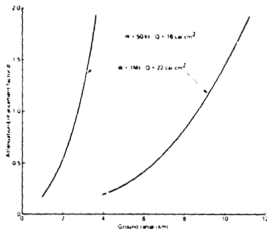
Fig. 3 Thermal reach modified by radiation attenuation or enhancement. SHOB = 152m, V = 19.3 km, T = 11.14R V 0 2R V
