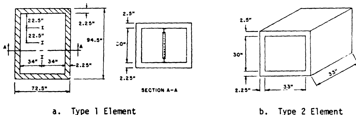
Figure 2. Test elements.
