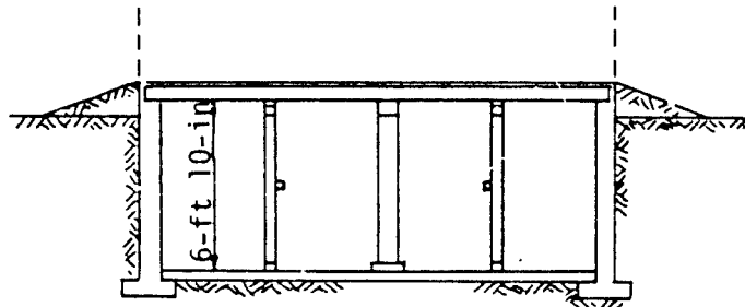
Fig. 2 Section A-A, Elevation
