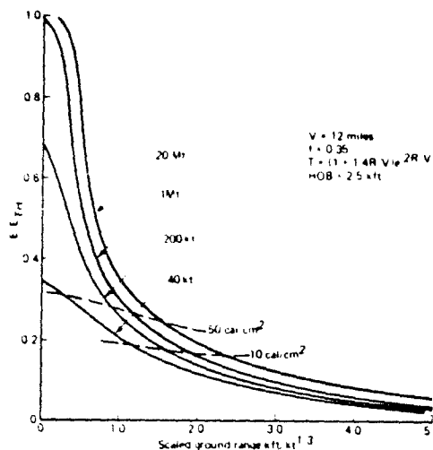
Fig. 4 Thermal radiation fraction incident after shock arrival vs. scaled ground range. V = 12 miles, T = 0.35, T = 11.14R V 0 2R V, HOB = 2.5 x ft
