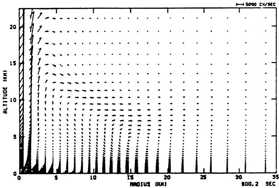
Figure 3. Particle Velocity Field at t = 15 min for (a) Case F-126 (rigid upper boundary at 20 km altitude) and (b) Case F-125 (transmissive upper boundary at 49 km altitude).
