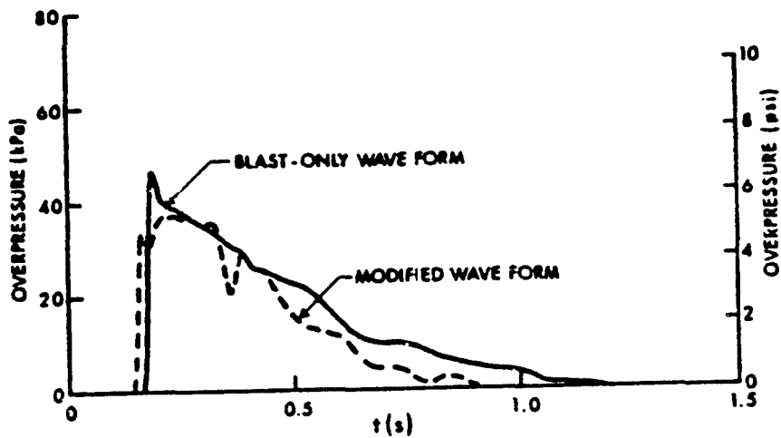
Figure 6. Predicted static overpressure modifications in CEG facility without venting TRS product.
