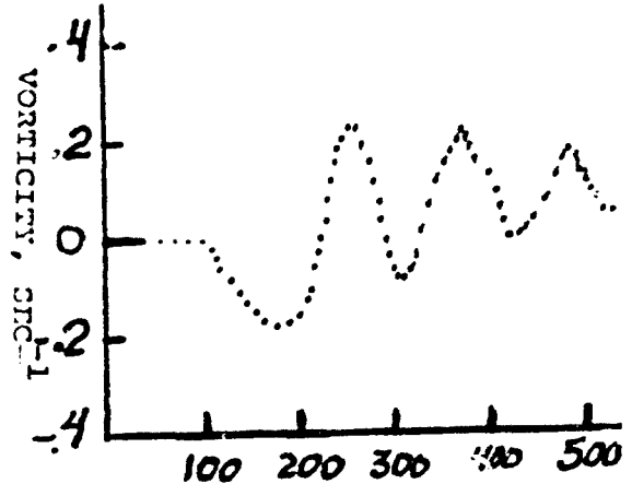
Fig. 2. Vorticity variation inside of Fire 6.
