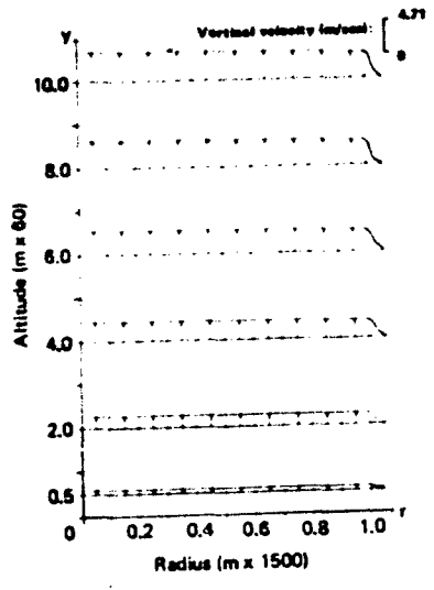
Fig. 4. Vertical velocity profiles, Hamburg firestorm.
