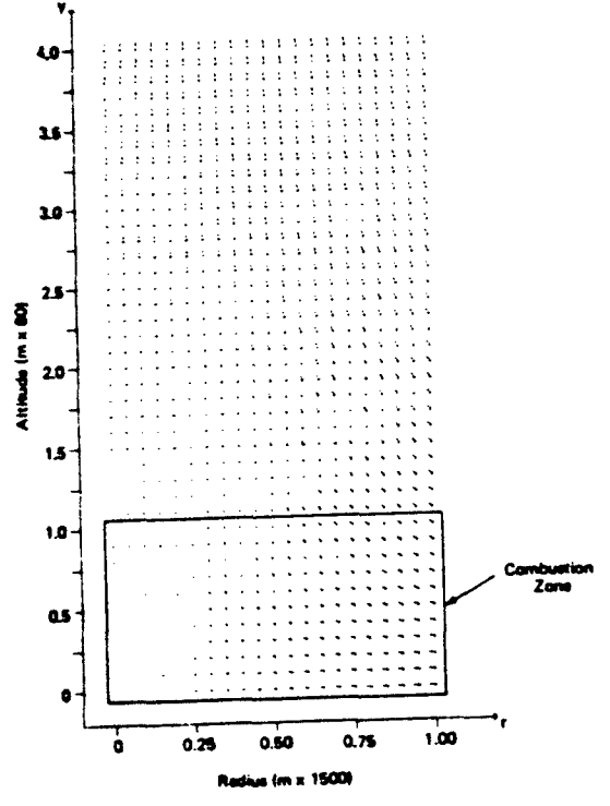
Fig. 5. Velocity field, Hamburg firestorm.
