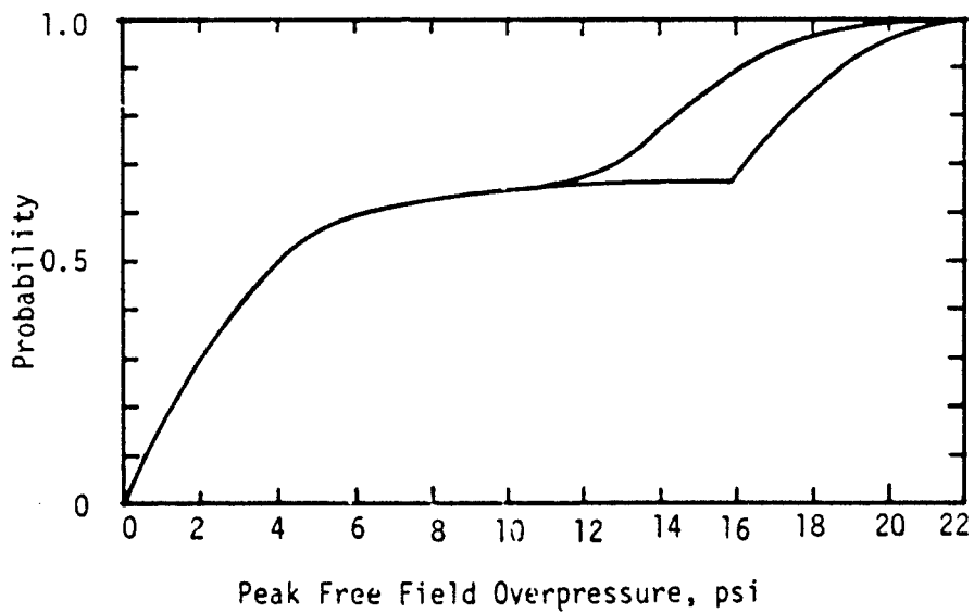
Fig. 5 Bounds on the Probability of Slab Failure
