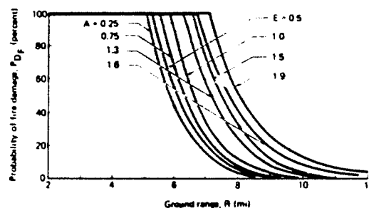
Fig. 5 Fire damage range for various amounts of radiation attenuation A and enhancement E, thermally and blast induced ignitions and fire spread, W = 1 \text{ Mt} , V = 12 \text{ mi} , \phi = 2.0 , \beta = 1.4 , building type/contents index = 4/7.5.
