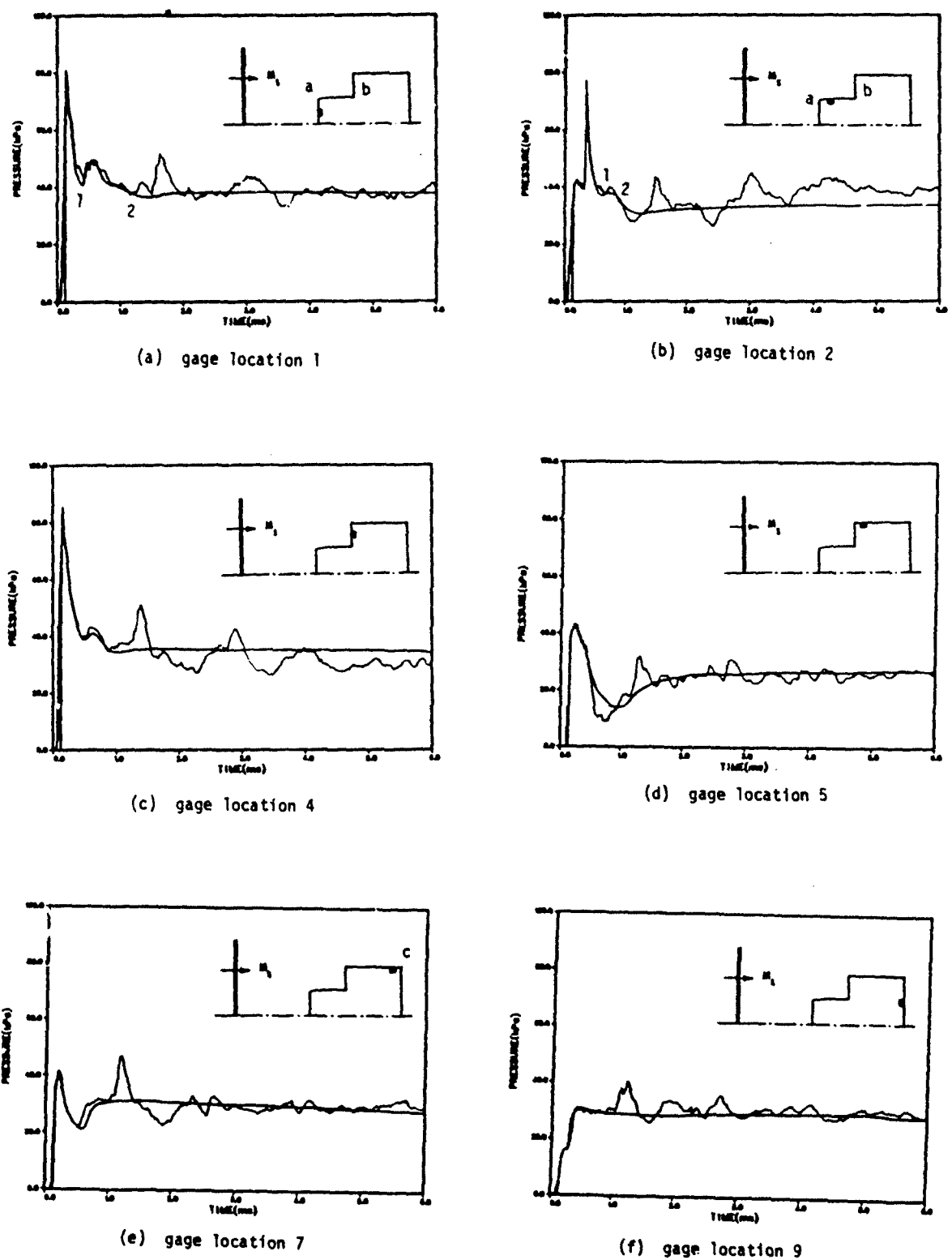
Figure 3. Pressure-time history for blast wave/truck interaction. (Shock strength overpressure = 34.2 kPa)
