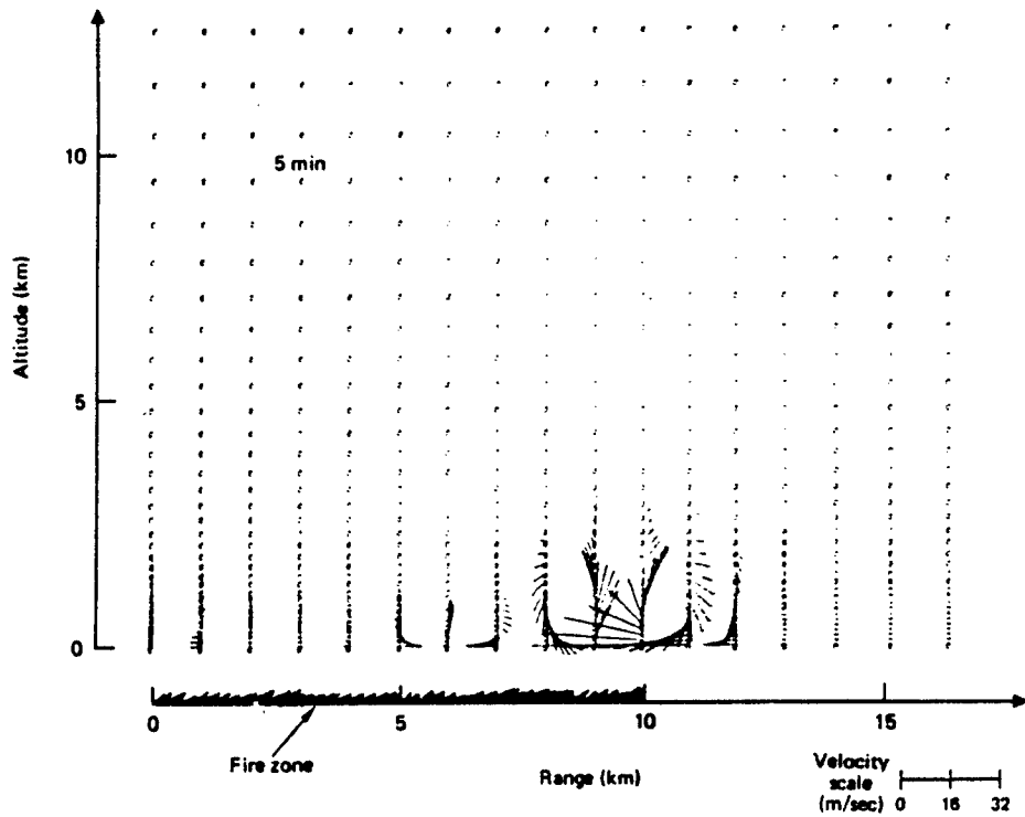
Fig. 2. Simulated flow field at 5 min. after ignition for sample 10 km fire.
