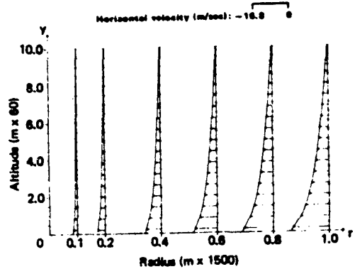
Fig. 3. Radial velocity profiles, Hamburg firestorm.
