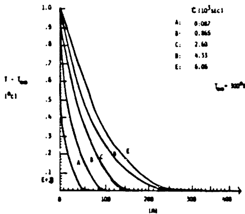
TEMPERATURE DISTRIBUTION HISTORY IN A MEDIUM WHEN SUBJECTED TO A THERMAL FLUX
