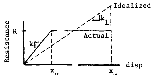
Fig. 2 Resistance Function
