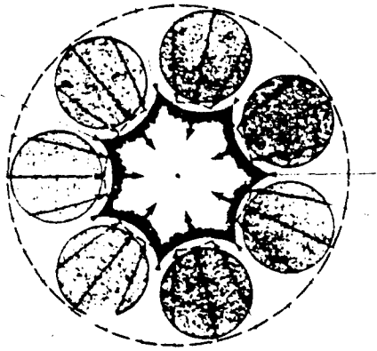
Fig. 5. Radial airflow and fire spread patterns suggested for annular cluster of large area fires.
