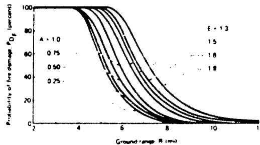
Fig. 4 Fire damage range for various amounts of radiation attenuation A and enhancement E thermally and blast induced ignitions, W = 1 \text{ Mt} , V = 12 \text{ mi} , \phi = 2.0 , \beta = 1.4 , building type/contents index = 4/7.5
