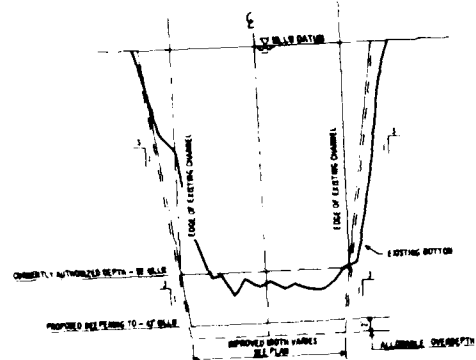
TYPICAL SECTION OAKLAND INNER HARBOR CHANNEL HORIZ SCALE 1"=100' VERT SCALE 1"=10'
