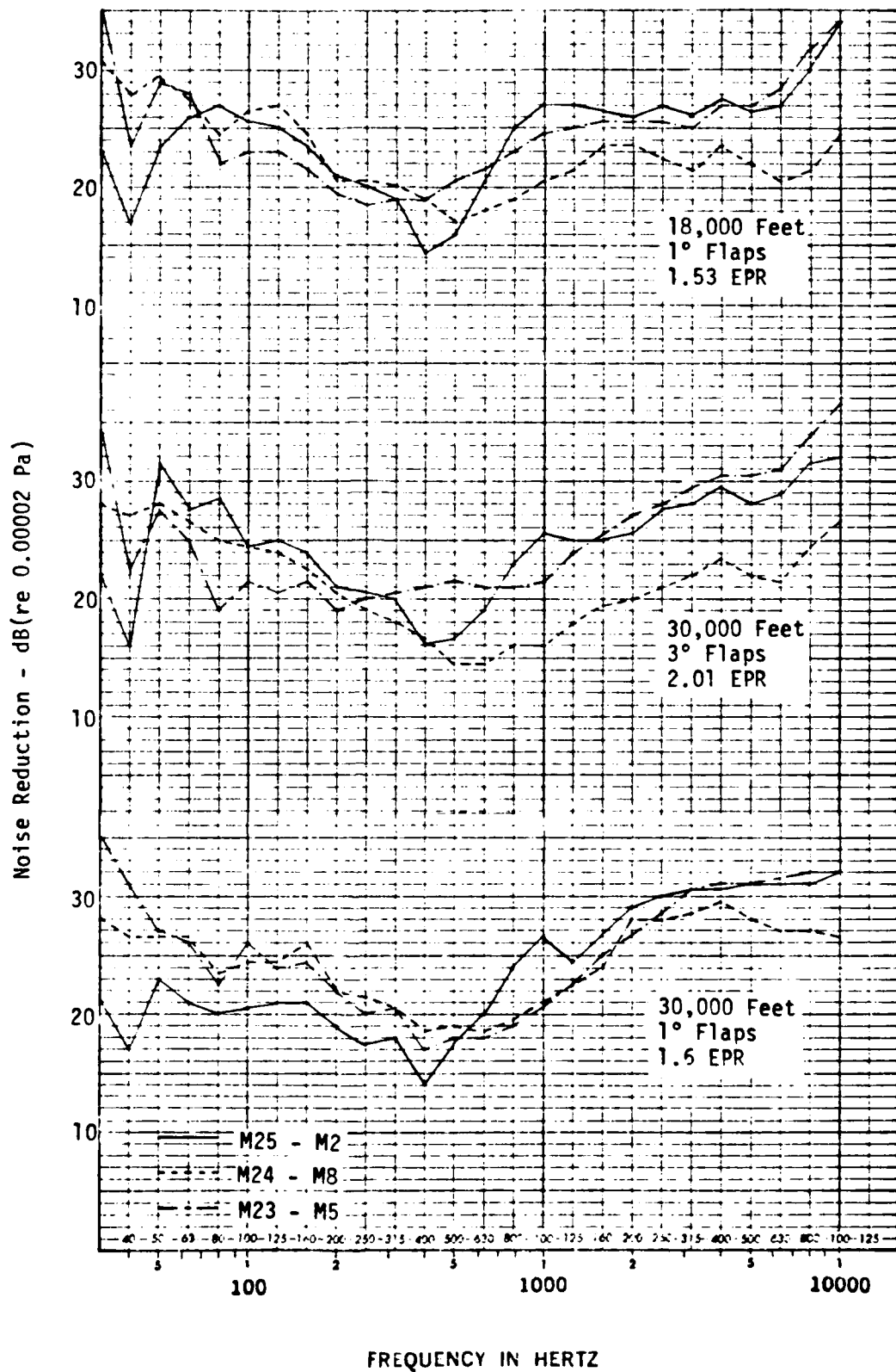
FIGURE 47 MEASURED NOISE REDUCTION FOR CRUISE CONDITIONS AT 18,000 FEET AND 30,000 FEET AND FLIGHT IDLE AT 30,000 FEET
