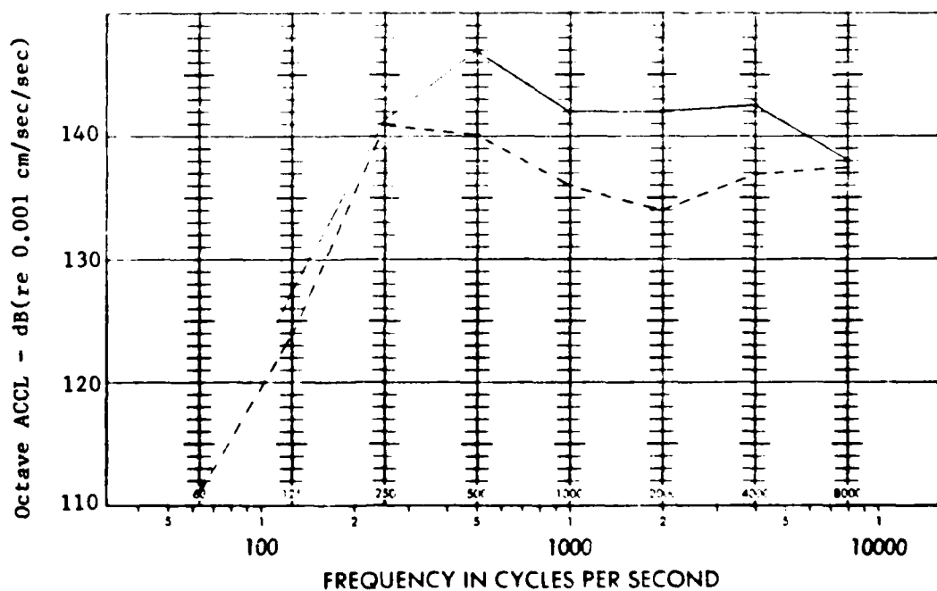
FIGURE 27 FUSELAGE WALL VIBRATION DURING TAKEOFF AND LANDING
