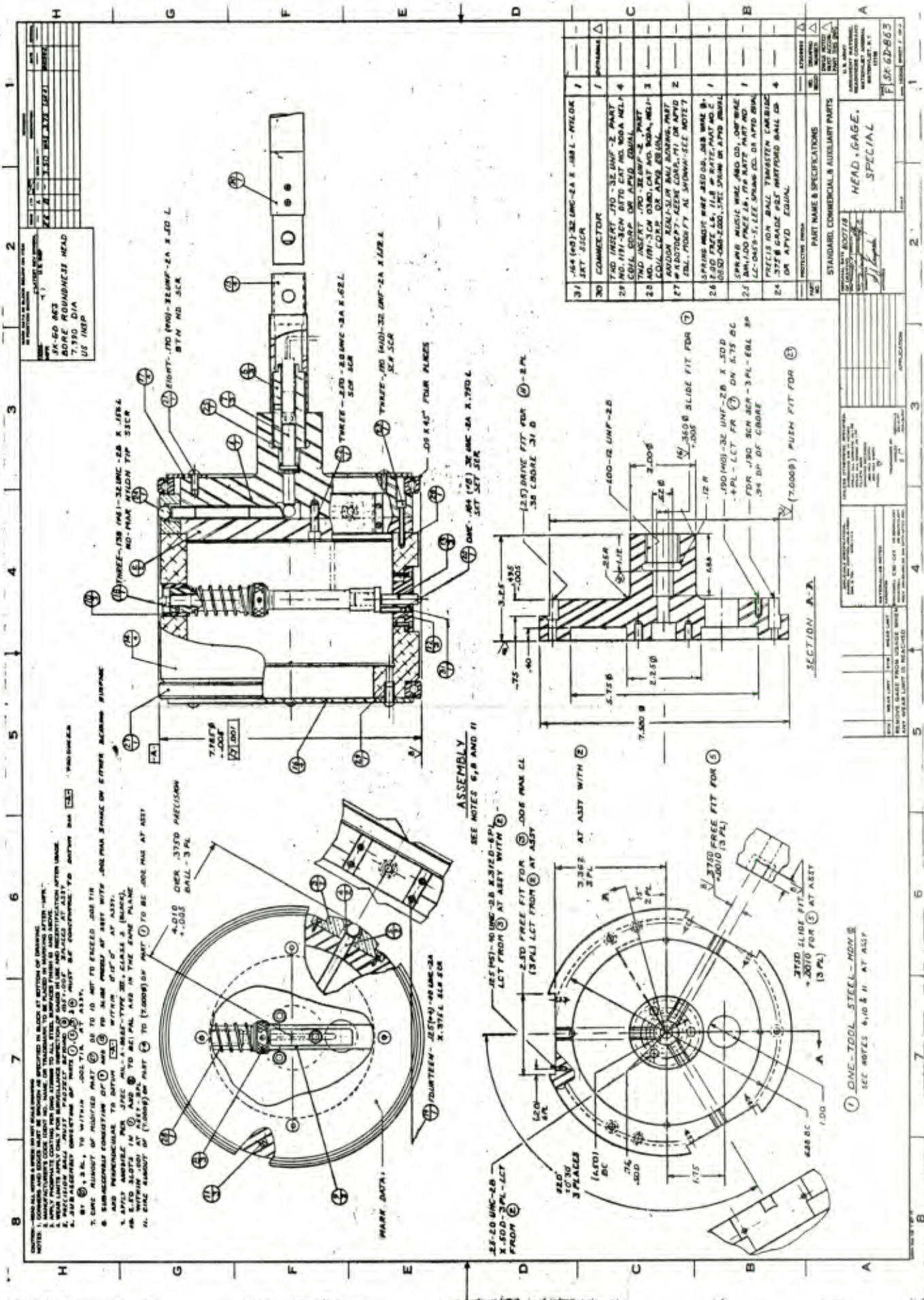
FIGURE 2. MEASUREMENT HEAD
