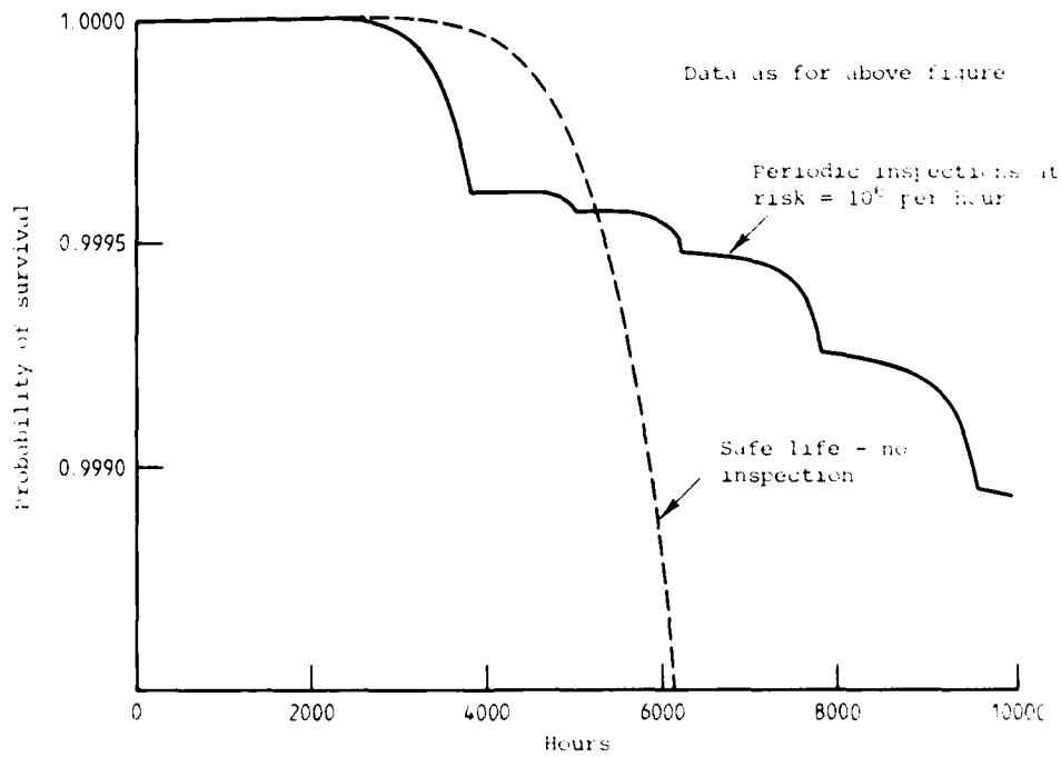
FIG. 18(b) PROBABILITY OF SURVIVAL vs LIFE (ref. 1)
