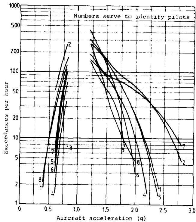
FIG. 16 VARIABILITY IN LOAD HISTORY CAUSED BY DIFFERENT PILOTS IN THE SAME AIRCRAFT (Ref. 10)
