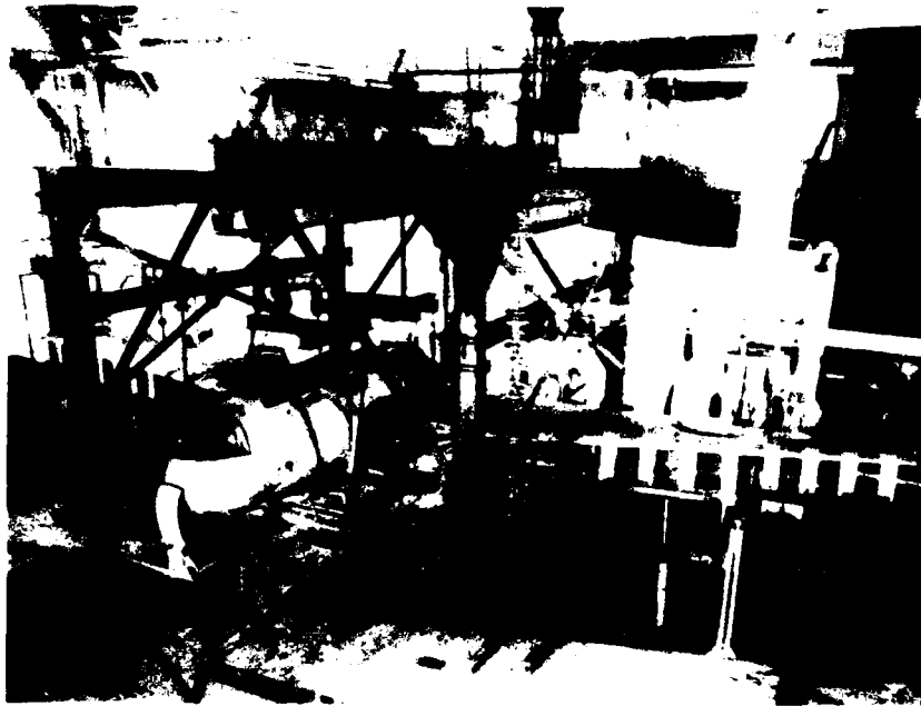
FIG. 13(a) "VAMPIRE" FULL-SCALE FATIGUE TEST RIG, WITH "DOVE" WING IN FOREGROUND (Ref. ...)
