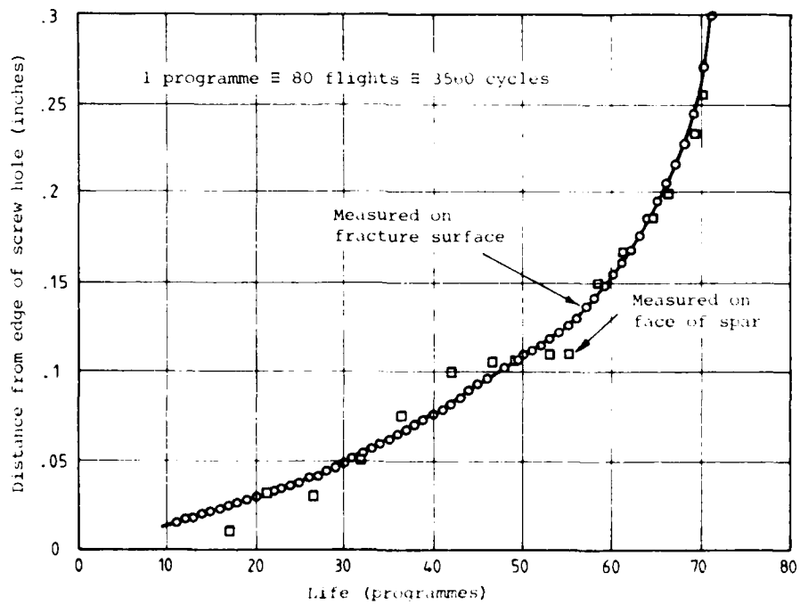
FIG. 13(b) CRACK LENGTH VERSUS LIFE, "VAMPIRE" SPAR (Ref. ...)
