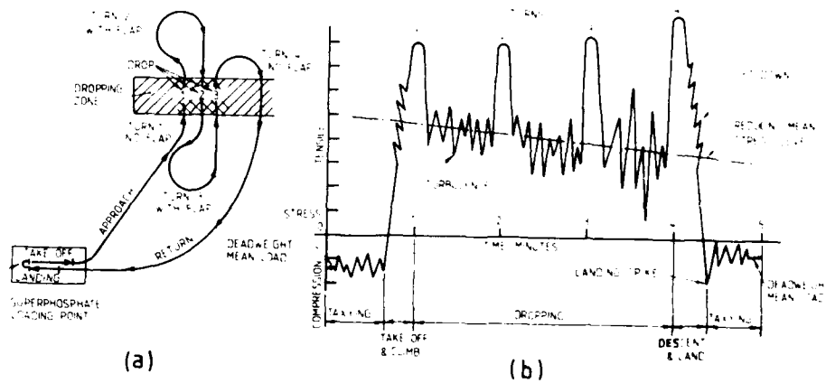
FIG. 15 (a) TYPICAL FLIGHT PATH FOR AERIAL AGRICULTURE OPERATIONS (b) STRESS-TIME PROFILE ON WING SPAR FLANGES FOR AIRCRAFT AT VARIOUS STAGES OF OPERATION (Ref. 10)
