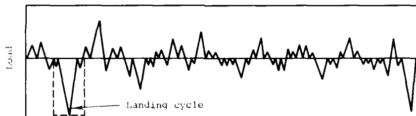
(c) Typical ground-air-ground cycle/gust load sequence (hydraulic rig)
