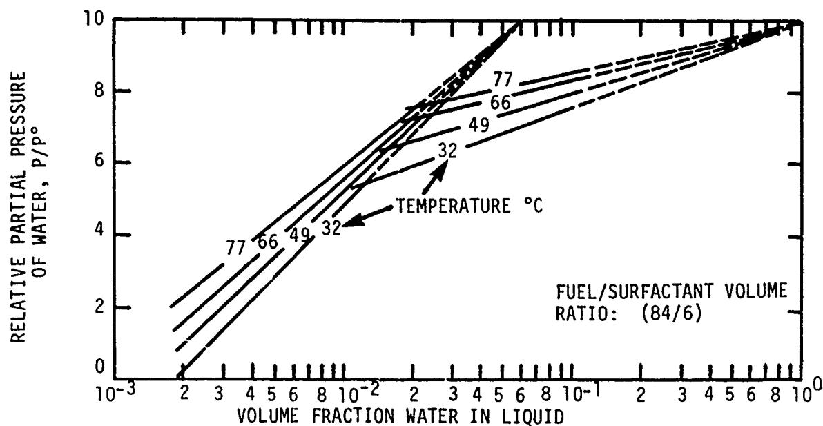
FIGURE 12. CORRELATED VAPOR LIQUID EQUILIBRIA
