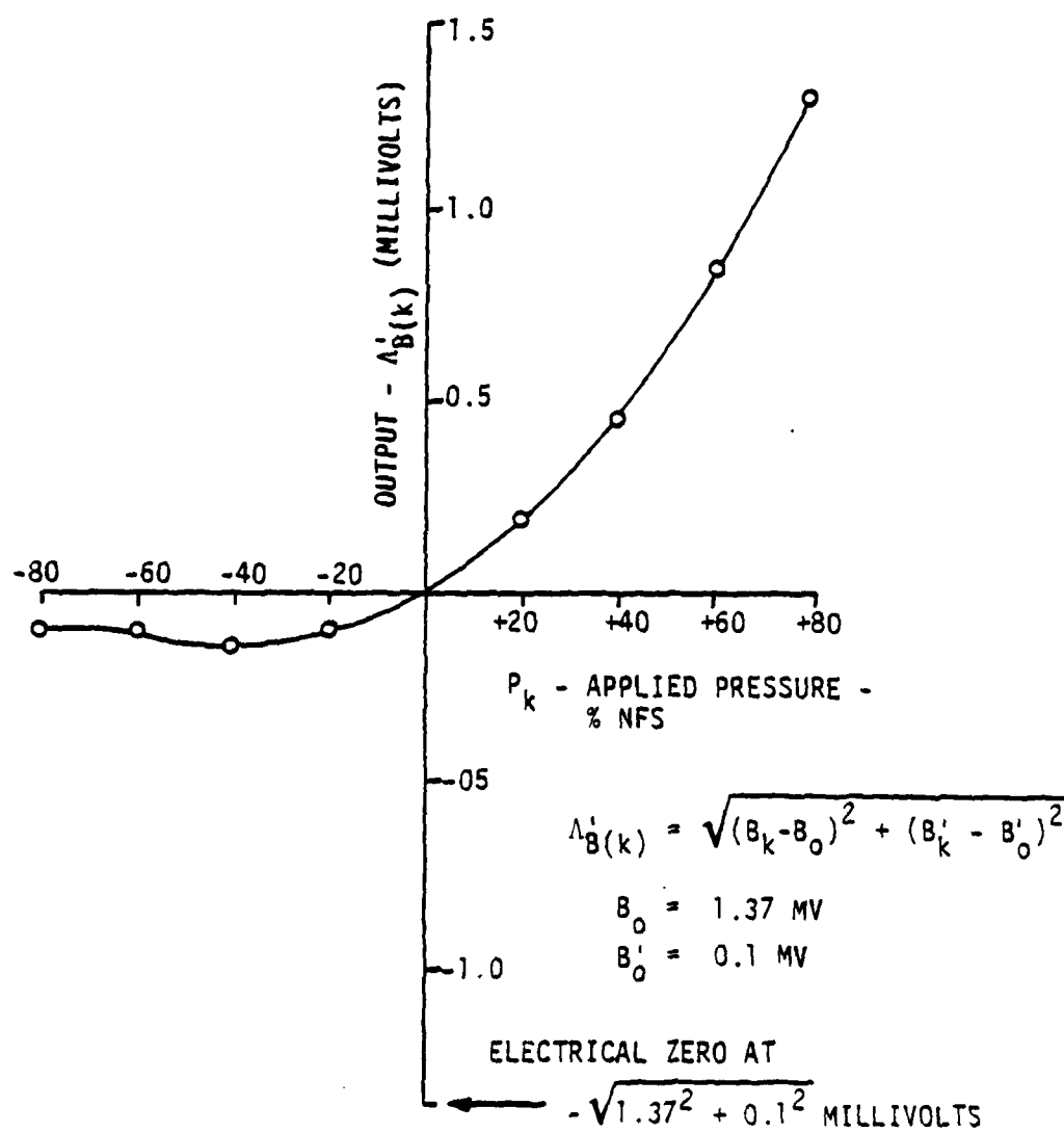
Figure 68. Calibration Data - Second Harmonic - Transducer 8-01
