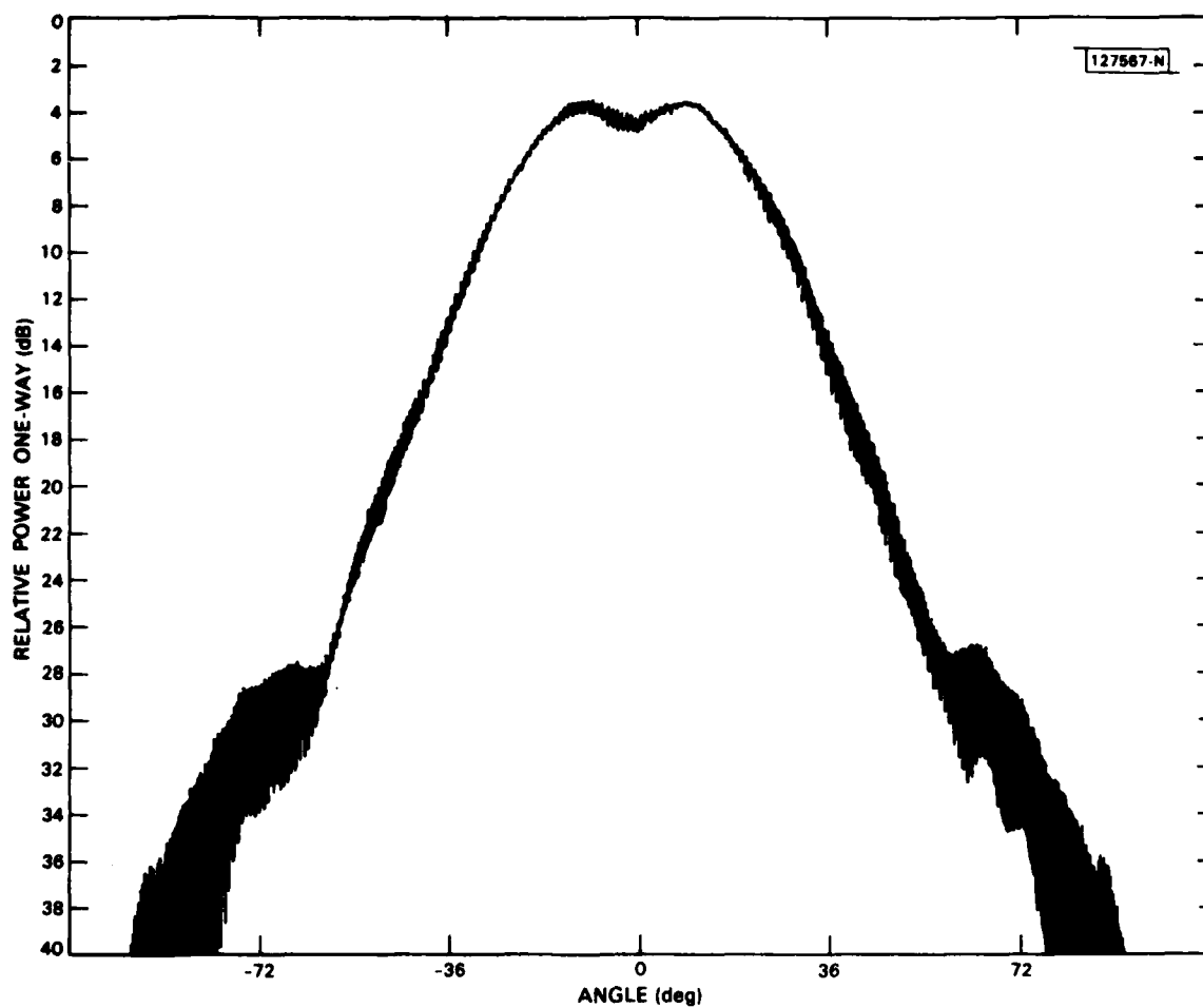
Fig. 11. Feed axial ratio pattern at 20.7 GHz.
