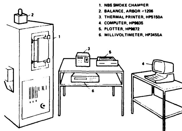
Figure 2: Equipment for Weight-Loss Data
