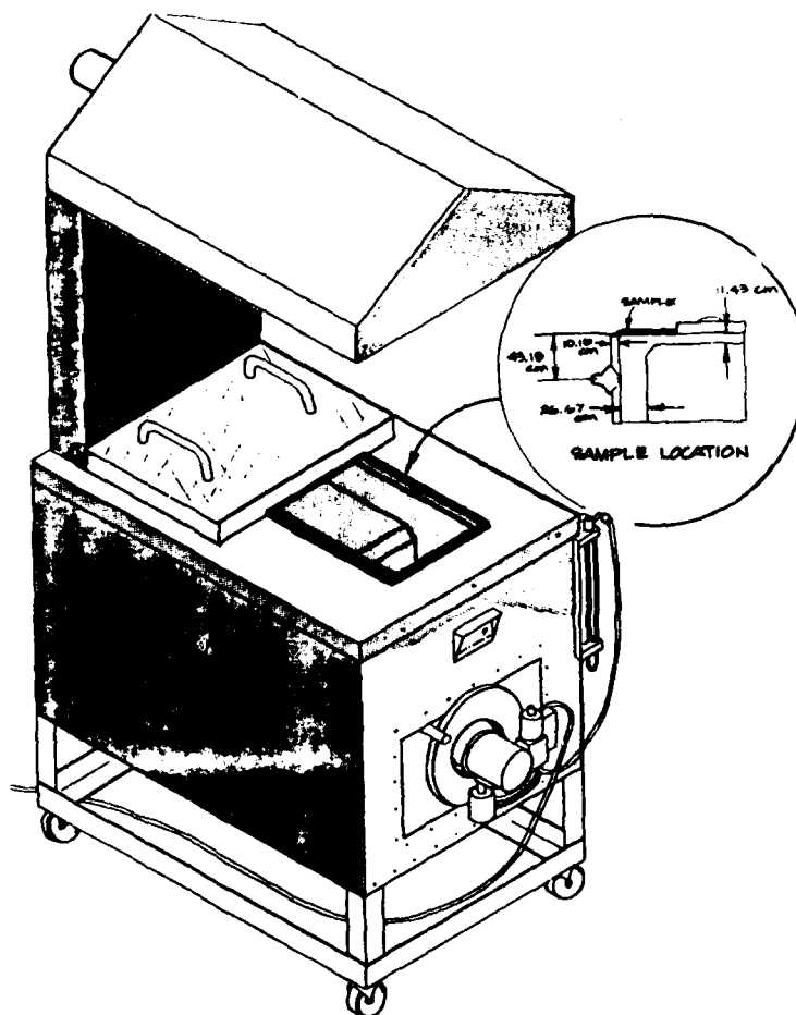
Fig. 2. Detail of T-3 Furnace.
