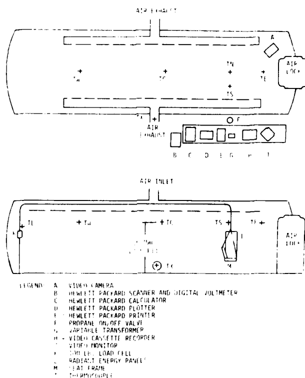
FIGURE 4. CFS INSTRUMENTATION
