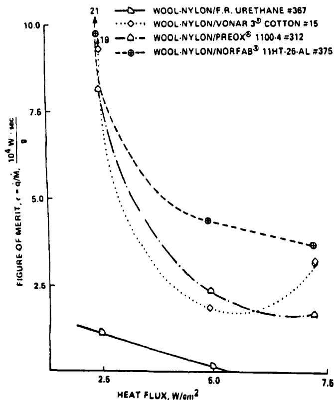
Figure 3: THERMAL EFFICIENCY COMPARISON OF HEAT BLOCKING LAYERS FOR OF URETHANE AS A FUNCTION OF HEAT FLUX AT 2 MINUTES ELAPSED TIME
