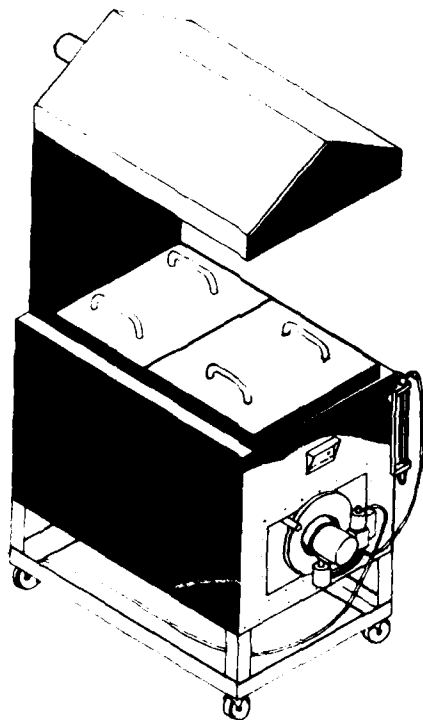
Fig. 1. The NASA-Ames T-3 Furnace.
