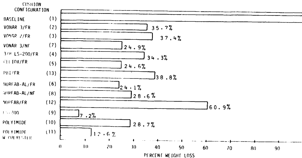
FIGURE 7. PERCENT WEIGHT LOSS
