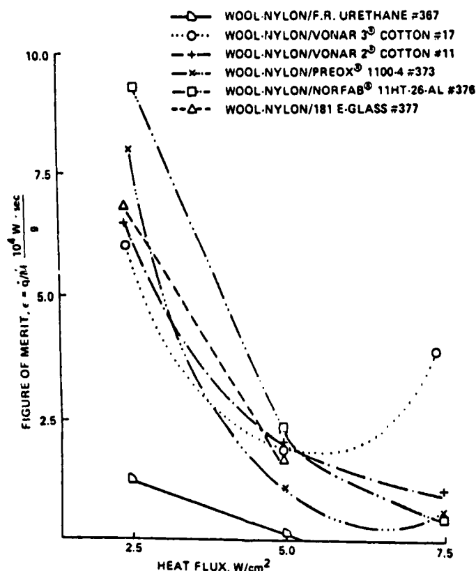
Figure 2: THERMAL EFFICIENCY COMPARISON OF HEAT BLOCKING LAYERS FOR FR URETHANE AS A FUNCTION OF HEAT FLUX AT 2 MINUTES ELAPSED TIME
