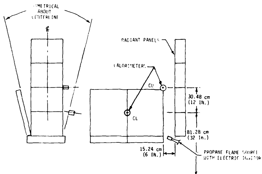
FIGURE 2. FUEL SOURCE AND CALORIMETER LOCATION
