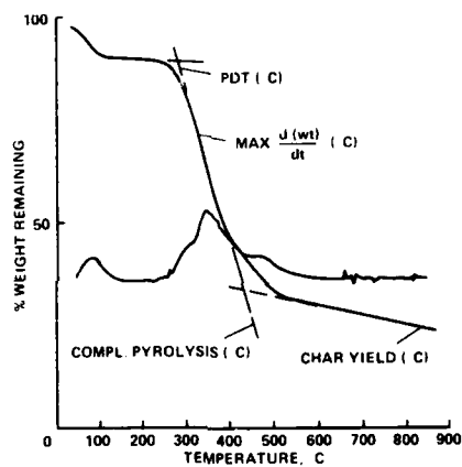
Figure 4: Typical Thermogram
