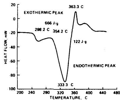
Figure 5: Differential Scanning Calorimetry of Vonar R 2
