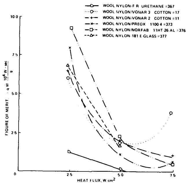
Figure 9: Figure of Merit Comparison of Heat Blocking Layers - F.R. Urethane as a Function of Heat Flux at 2 Min.
