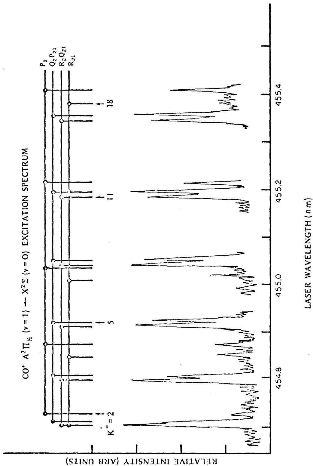
Fig. 11. Laser-induced fluorescence spectrum of a small portion of the rotational states in the CO + (A-X) system used to probe the rotational state populations in the X, v''=0 state produced by the N + + CO charge transfer reaction.
