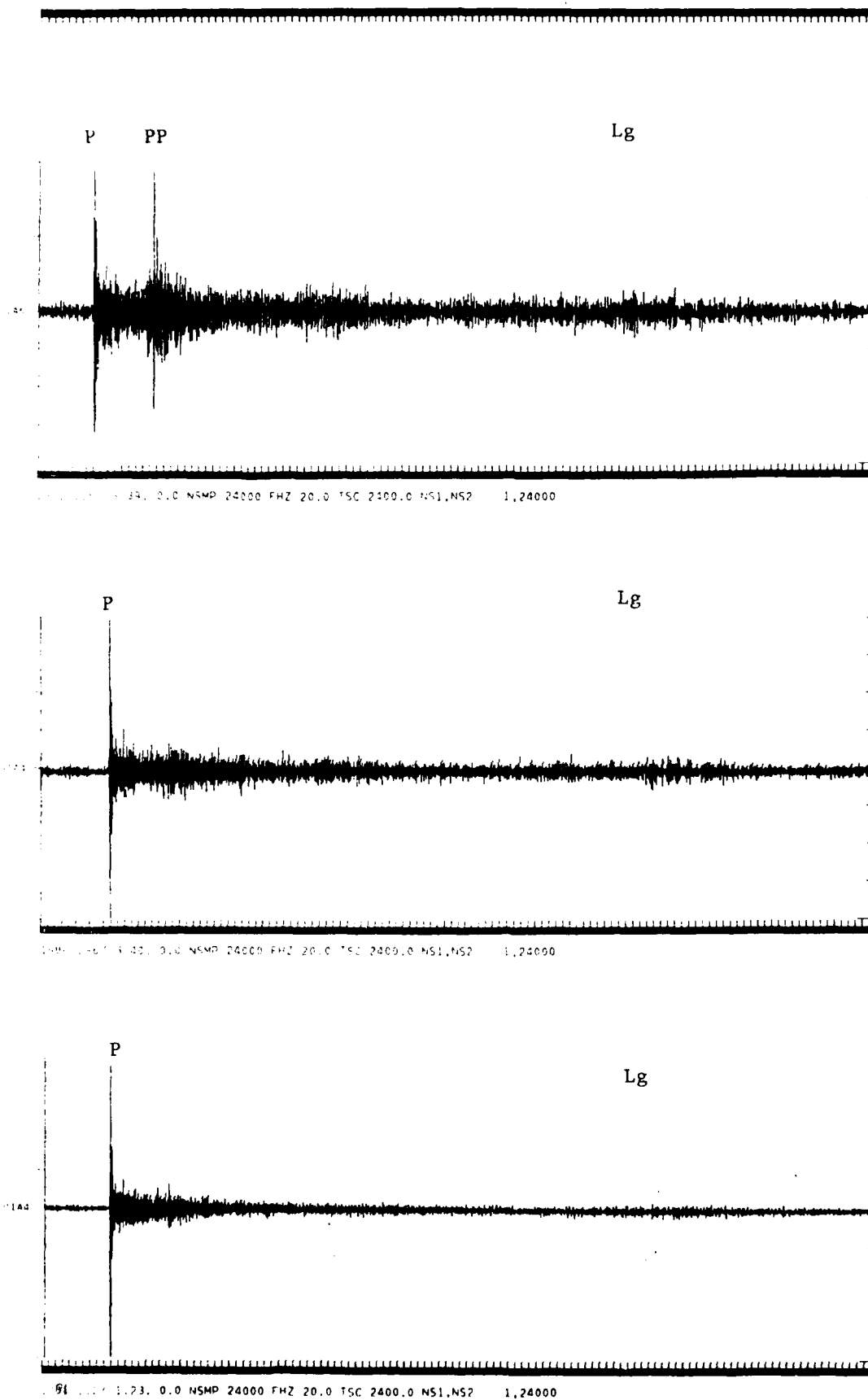
Fig. 4. 20 minutes recordings of the same three events as displayed in Figure 3. Note the much more rapid coda decay of event 3 (bottom).
