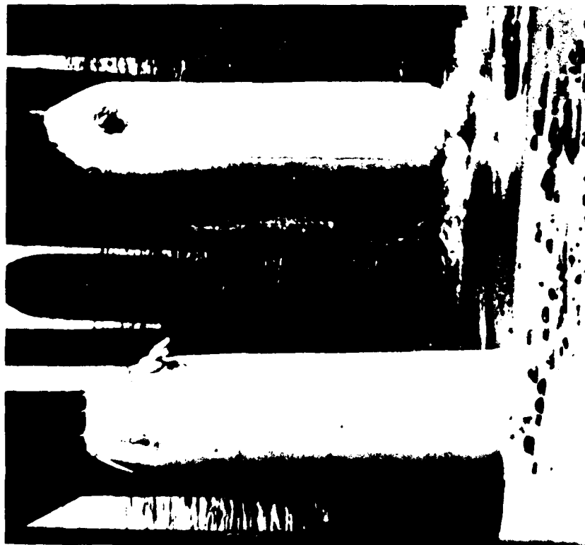
Figure 73. Piles repaired using fiberglass forms and grout (photo courtesy of Aquatic Marine Systems).
