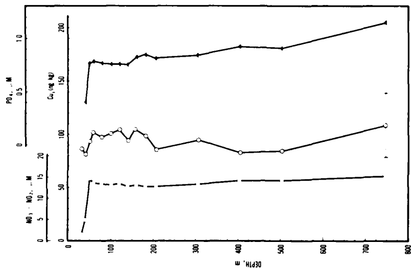
Figure 11. Station 030 vertical profiles showing copper (O), nitrate-plus-nitrite (□), and phosphate (▲).
