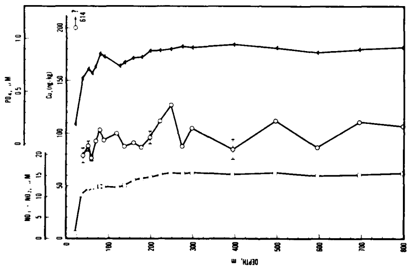
Figure 10. Station 026 vertical profiles showing copper (O), nitrate-plus-nitrite (□), and phosphate (▲). Potentially contaminated samples marked with "?".
