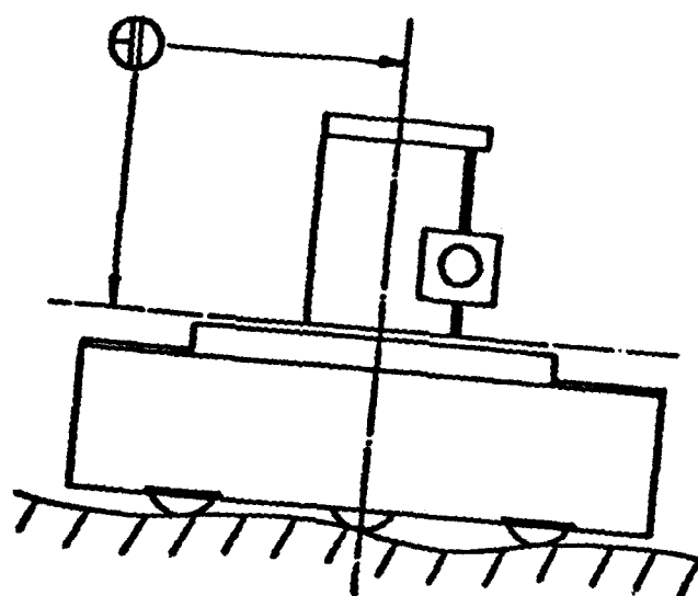
Three-point support: foundation movement does not distort the machine structure.
