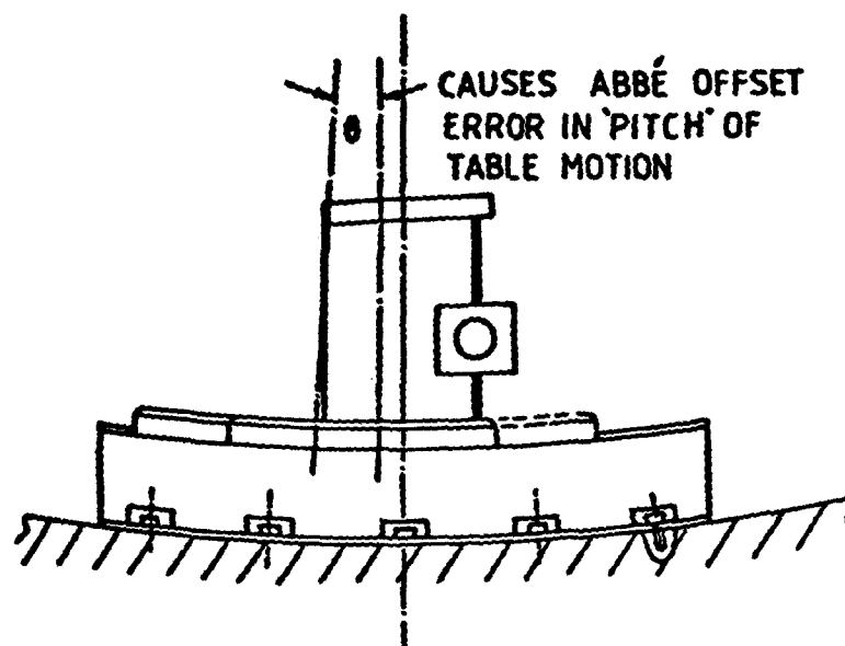
Multipoint support: foundation movement causes distortion of the machine structure.
