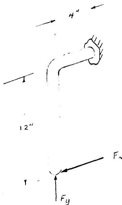
Figure 2. Alignment Arm Force Diagram
