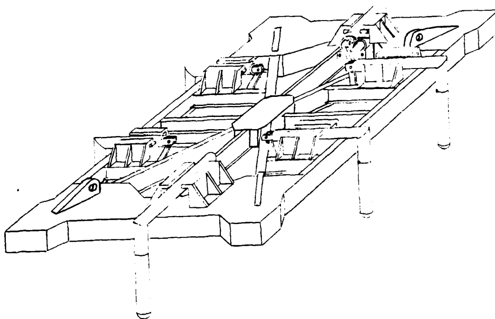
Figure 1. Spreader Bar with Energy Dampening Alignment Arms
