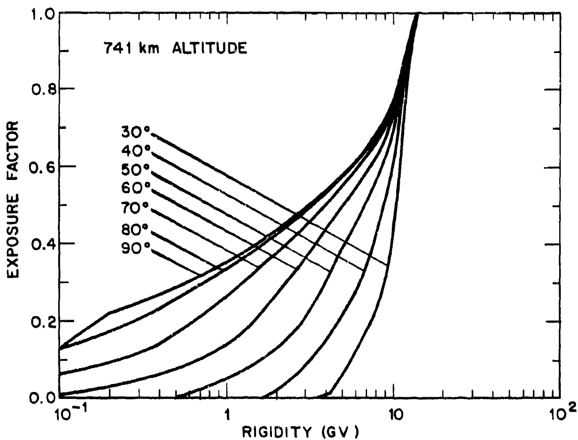
Figure 12. The same as figure 10, but for a 741 km altitude.
