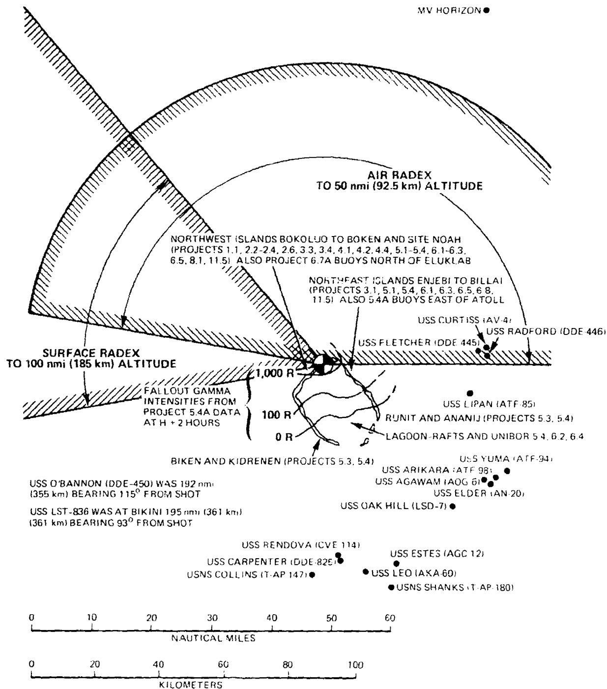
Figure 23. Radex areas, project instrumentation locations, and positions of task force ships, IVY, MIKE.
