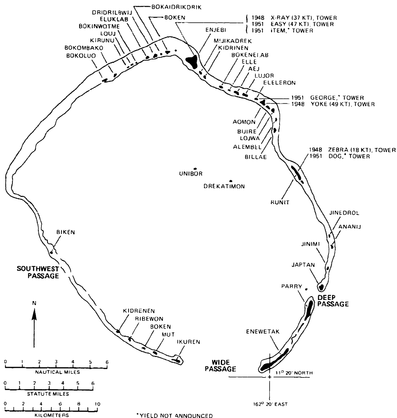
Figure 2. Enewetak Atoll, 1952, with pre-IVY test sites.
