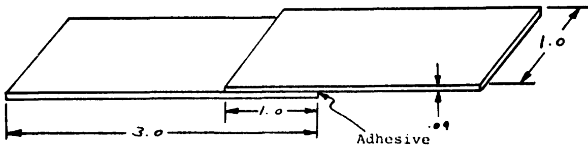
c. Strips for Shear Test
