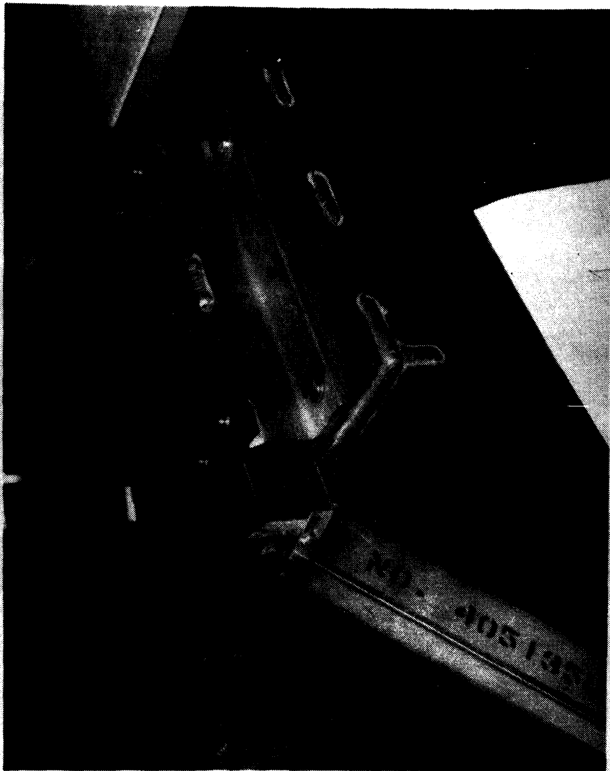
Figure 17. Impact Test Specimen III B-1
