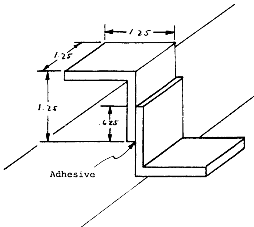
a. Angles for Qualitative Hammer Test
