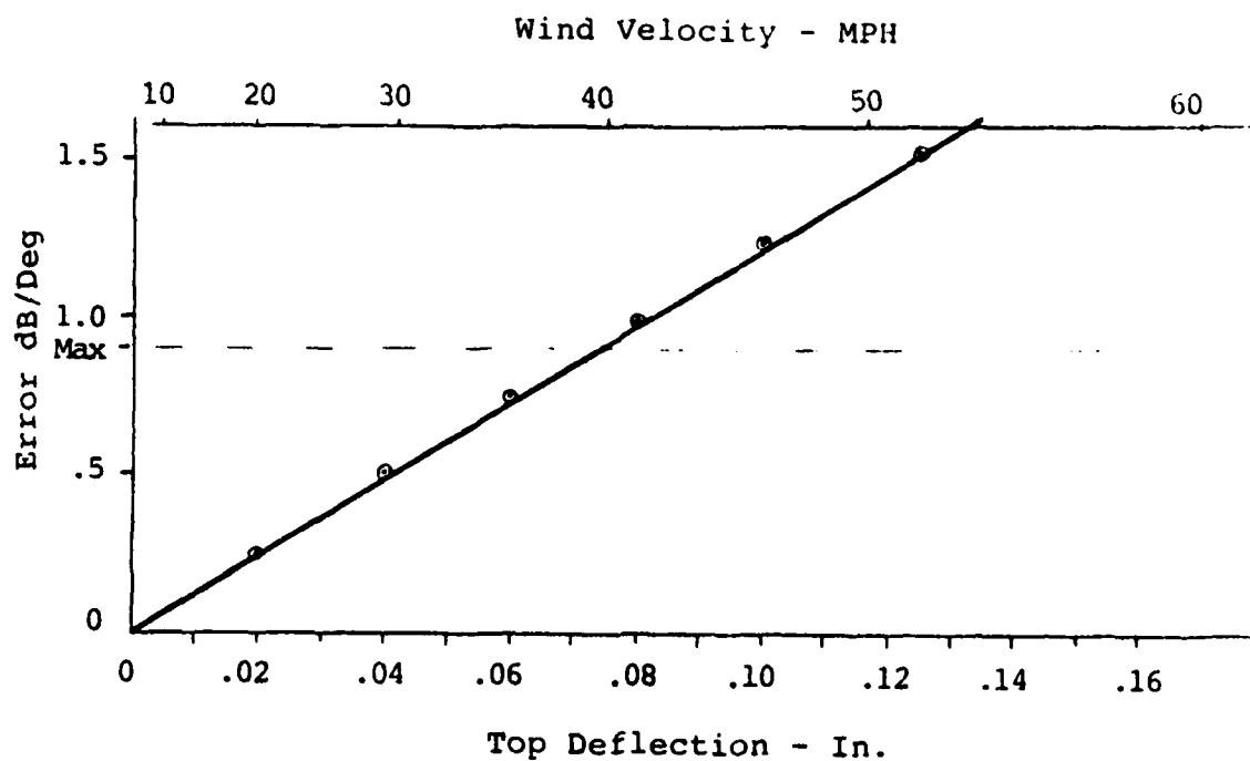
Figure 1. Computed Error Vs. Deflection and Wind Velocity for WR-159 AZ Cantilever Waveguide
