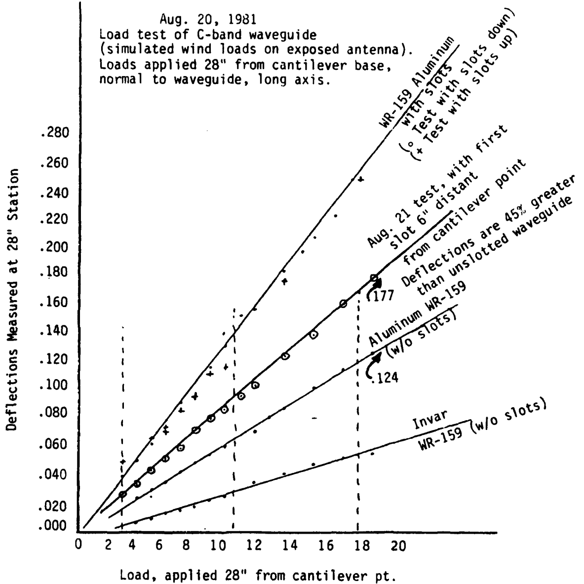
Figure 7. Preliminary Load Test of Slotted and Unslotted Waveguides
