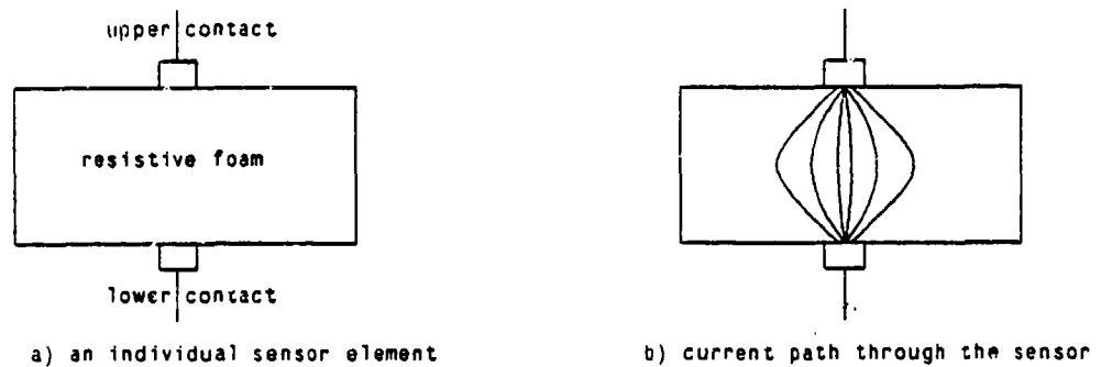
Figure 2-2: An Individual Sensor Element
