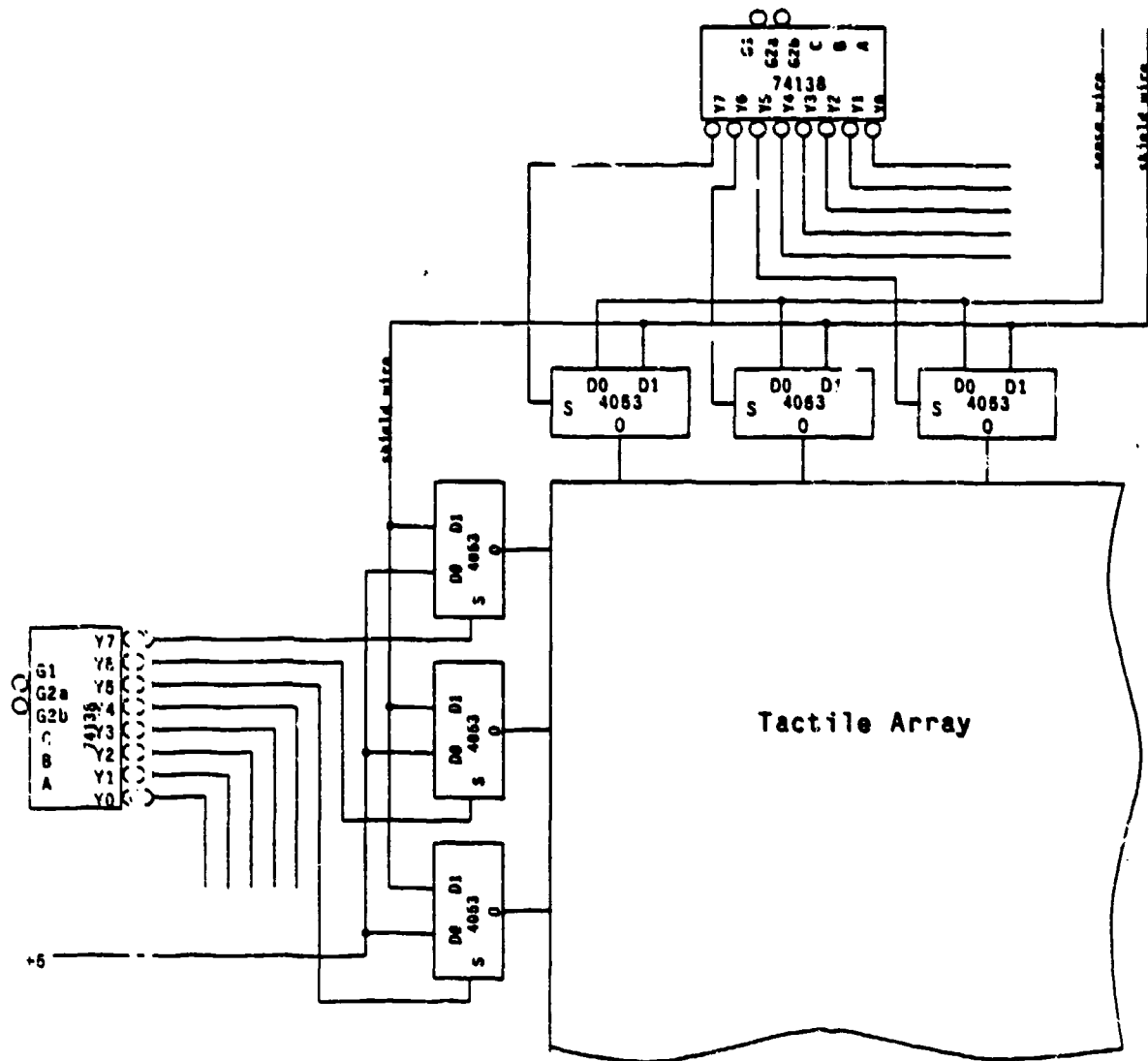
Figure 3-2: Detailed View of Connection to the Sensor Array
