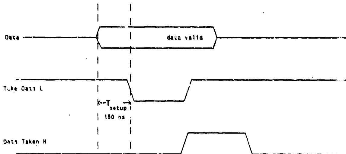
Figure 3-4: Output Timing Cycle
