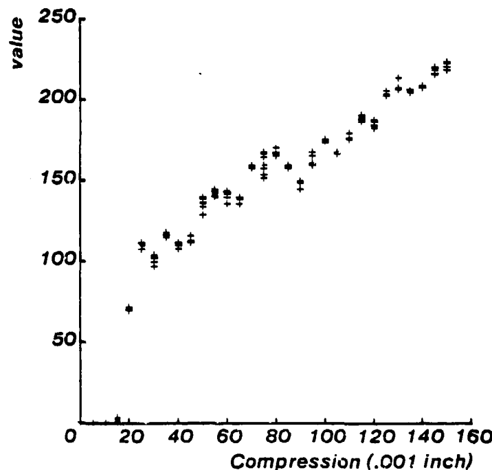
Figure 2-3: Sensor Reading versus Compression
