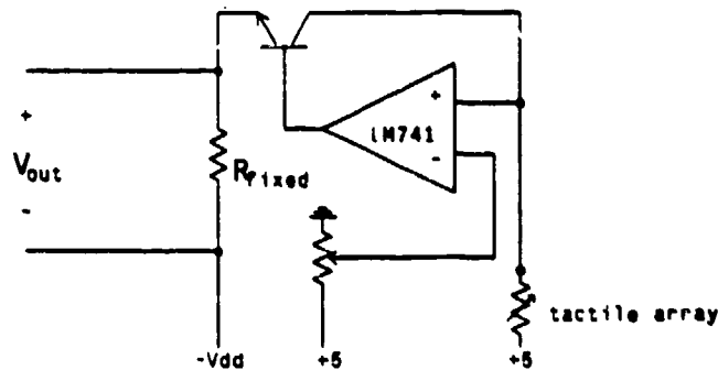
Figure 3-1: resistance to voltage conversion
