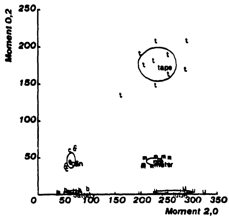
Figure 4-6: Scatter diagram of m_{0,2} versus m_{2,0} for the training set
