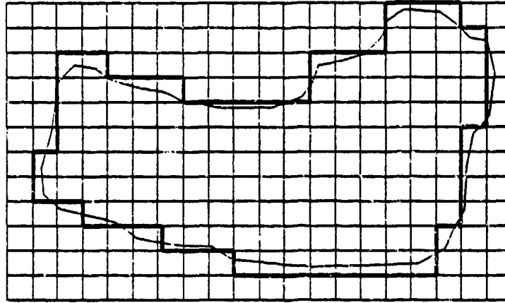
Figure 4-12: Discrete approximation to the area of an object
