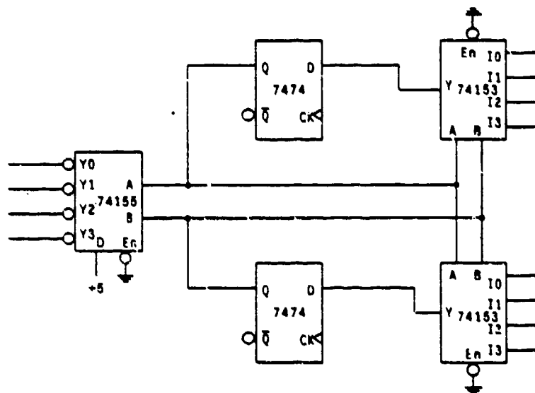
Figure 3-6: Four state finite state machine
