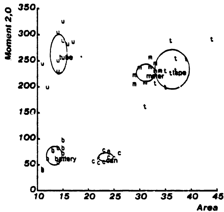
Figure 4-4: Scatter diagram of m_{2,0} versus Area for the training set
