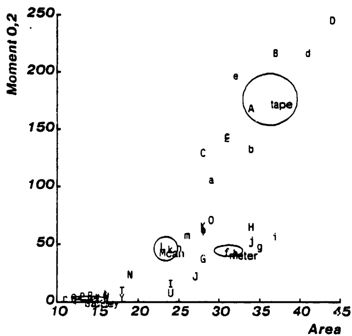
Figure 4-10: Scatter plot of m_{0,2} versus Area for test data
