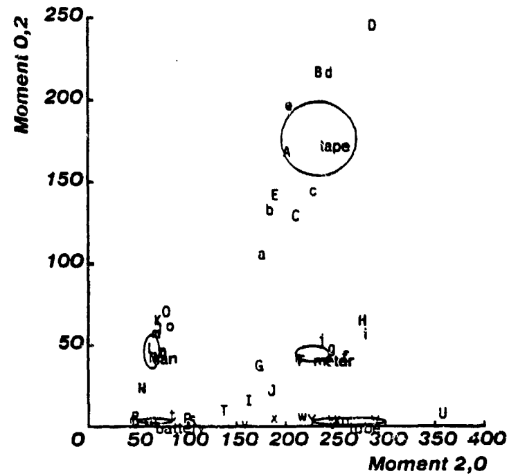
Figure 4-11: Scatter plot of m_{2,0} versus m_{0,2} for test data
