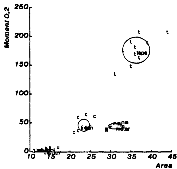
Figure 4-5: Scatter diagram of m_{0,2} versus Area for the training set
