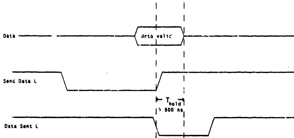
Figure 3-3: Input Timing Cycle
