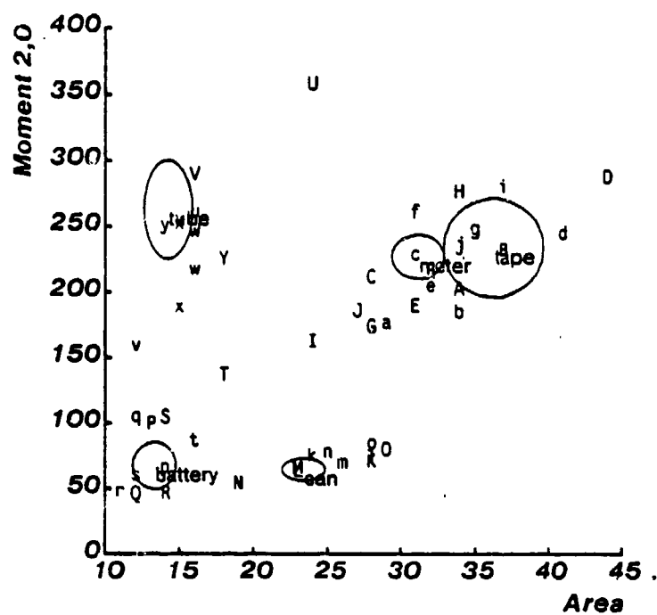
Figure 4-9: Scatter Plot of m_{2,0} versus Area for test data
