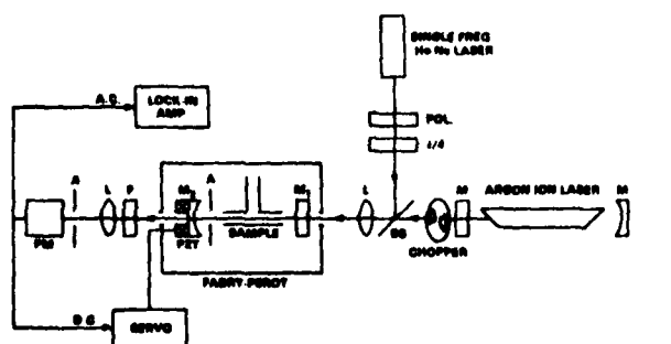
FIG. 1. Experimental configuration. BS—beam splitter, L —lens, M_1, M_2 —Fabry-Perot mirrors, F —633-nm bandpass filter, and PM—photomultiplier tube.
