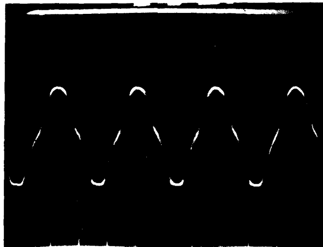
Figure 51. Generated Voltage Waveshape - Stator Winding Final Magnetization
