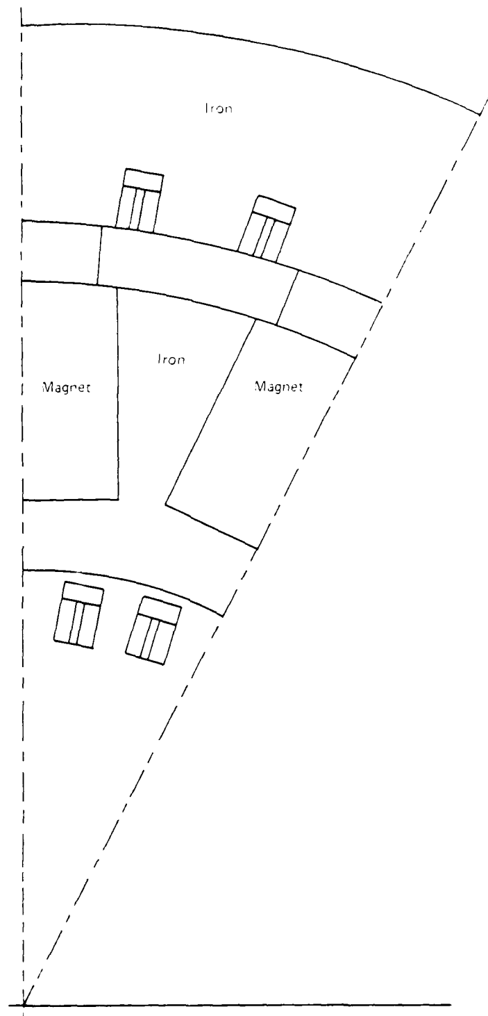
Figure 30. Rotor, Conductor and Back Iron Arrangement for Finite Element Analysis.
