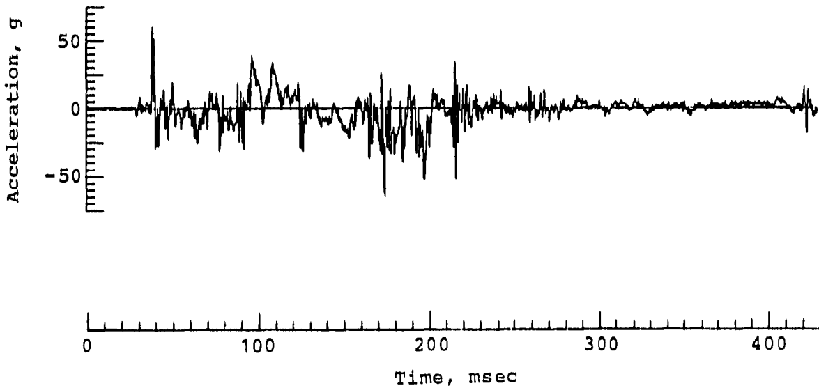
Tail rotor gearbox lateral acceleration
