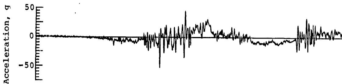
Main rotor hub longitudinal acceleration
