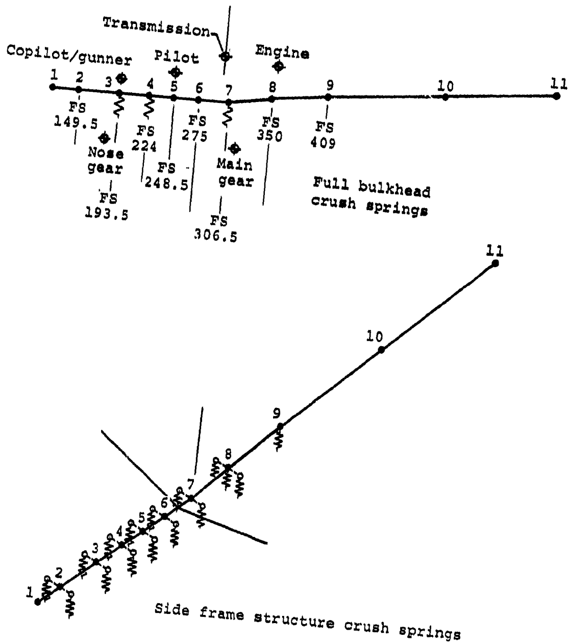
Figure D-6. KRASH math model of lower fuselage crushable structure.
