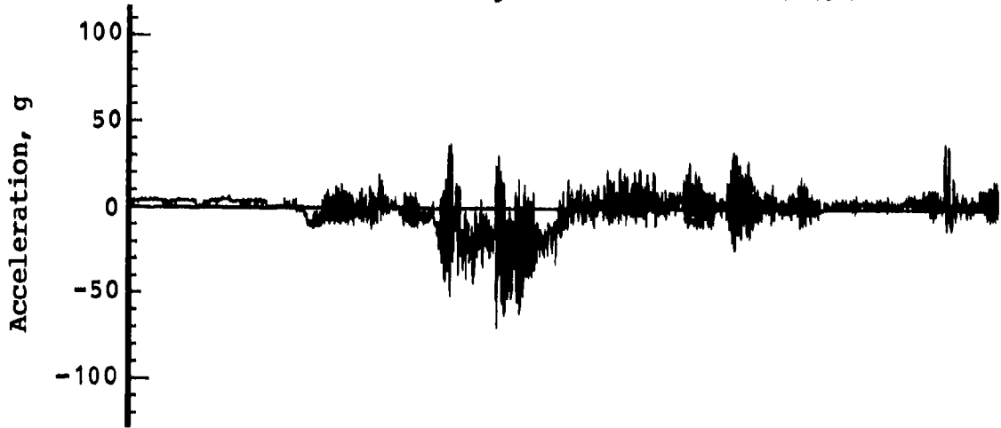
Transmission cg vertical acceleration
