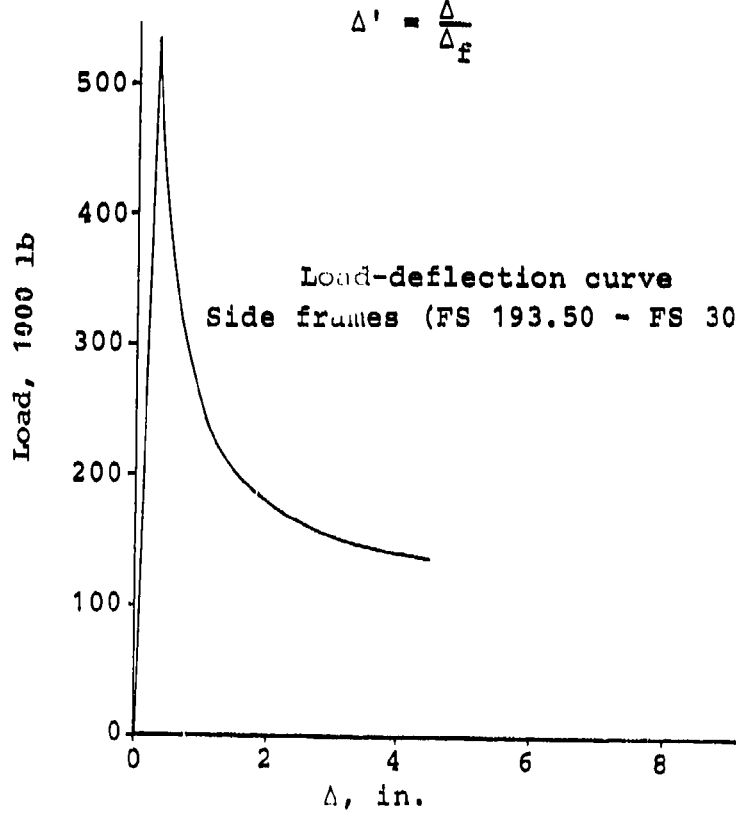
Figure B-5 (cont'd). Nondimensionalized curve shape.
