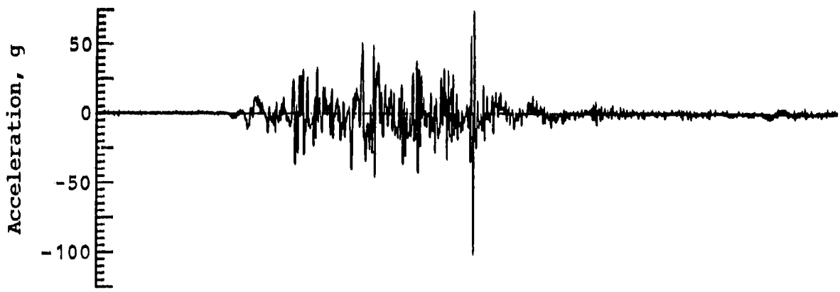
Pilot bulkhead lateral acceleration
