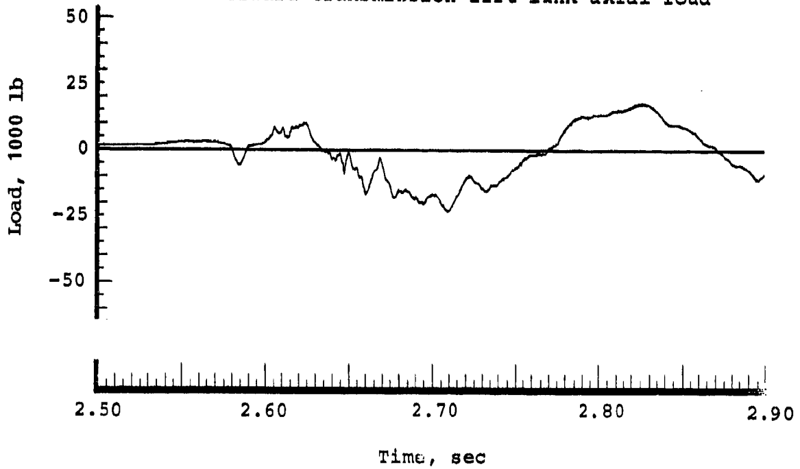
Left forward transmission lift link axial load
