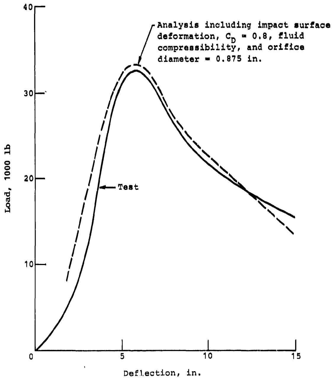
Figure 12. Test and analysis comparison of YAH-63 main landing gear shock strut load.
