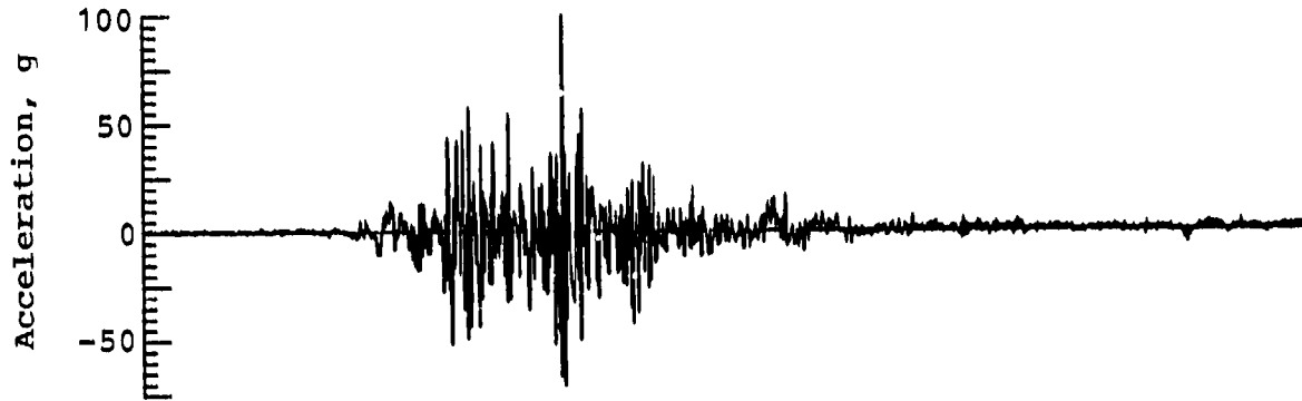
Aircraft cg longitudinal acceleration
