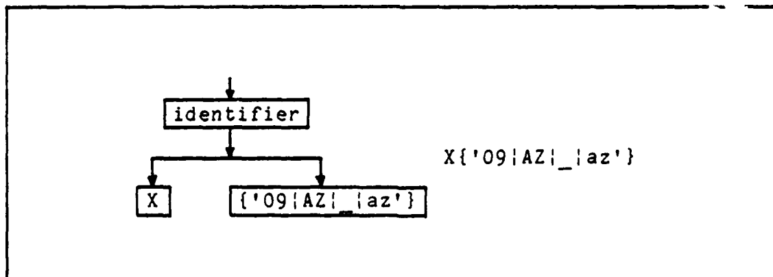
Figure 3-9. Identifier with first character.
