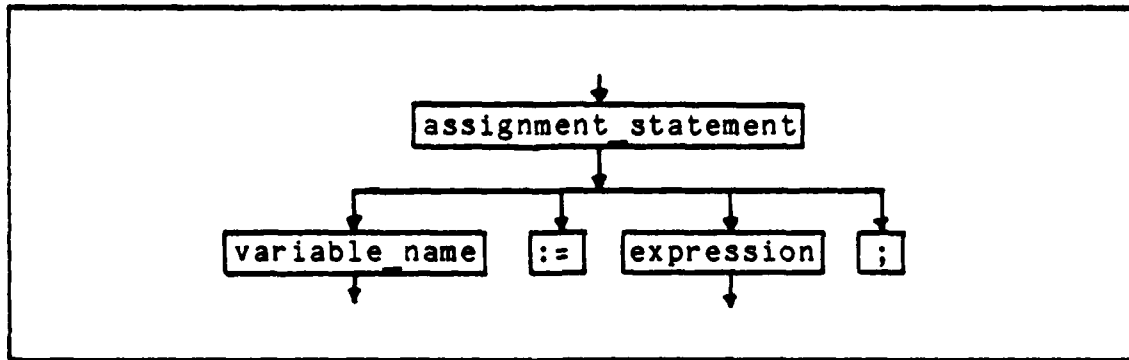
Figure 2-2. Parse tree for ADA assignment statement.
