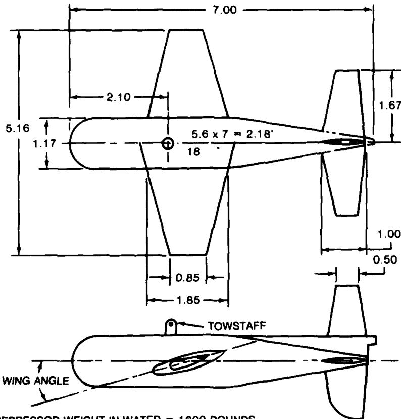
Figure 1 - DTNSRDC Depressor
